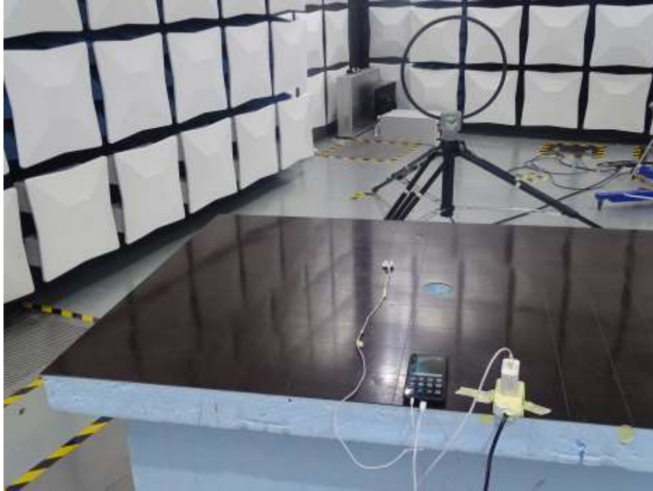
3. Radiated Spurious Emission (9K-30MHz)
