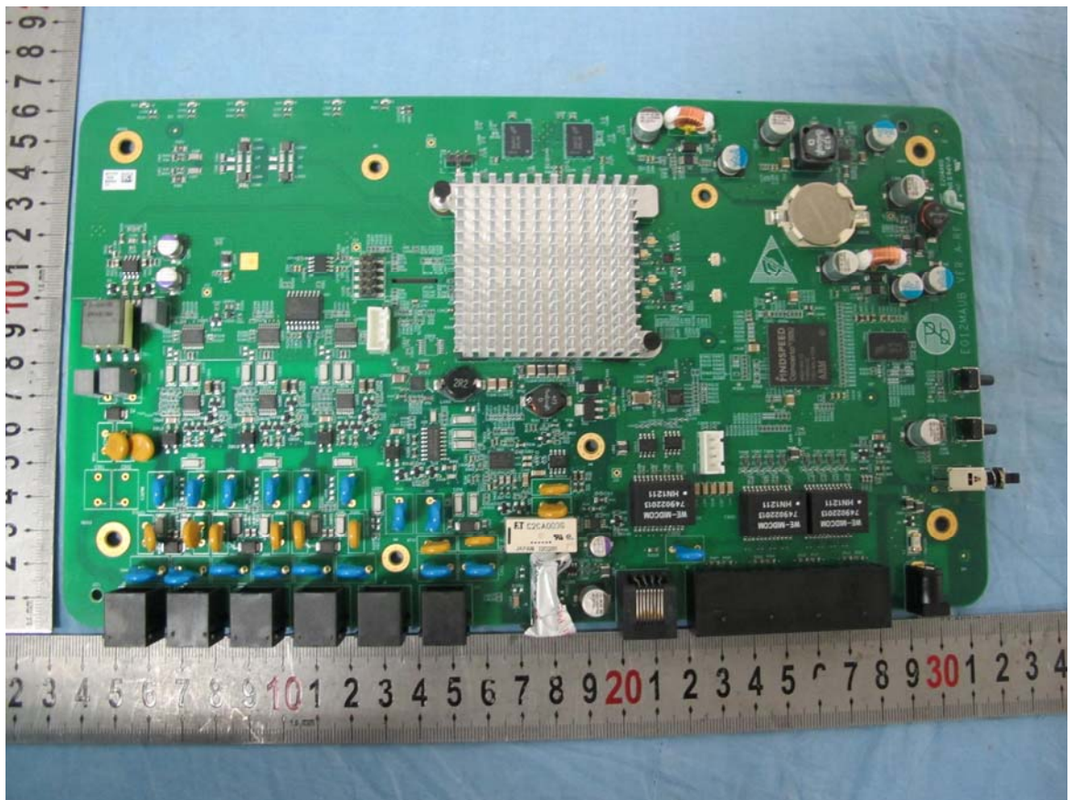
EG12MAUB board and interfaces of eSpace EGW1520(top)
