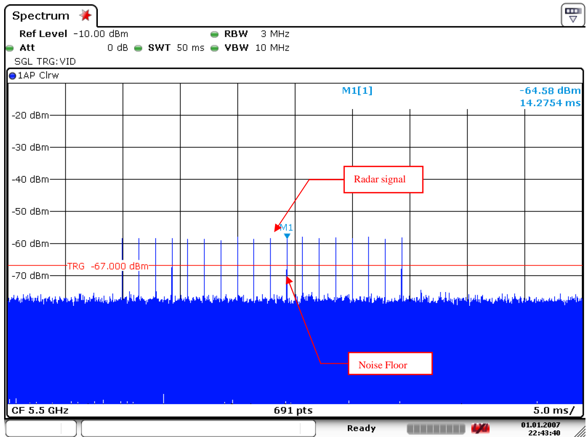
Radar Signal 1
