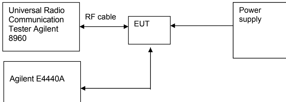
Figure 2. Test Set-up
