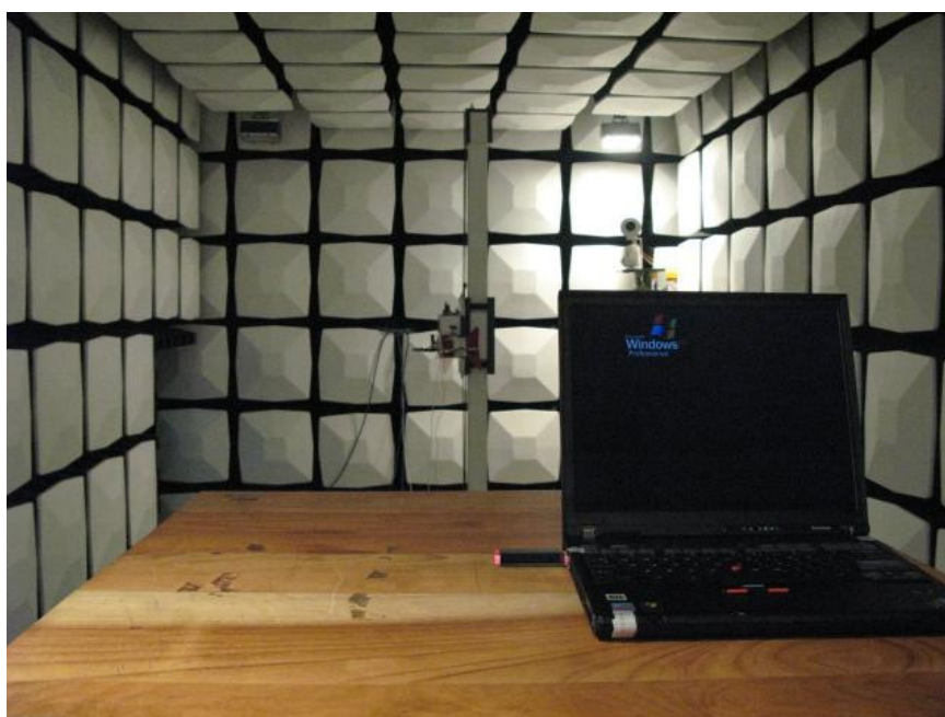
Radiated Spurious Emission 2G~18GHz (TC1)
