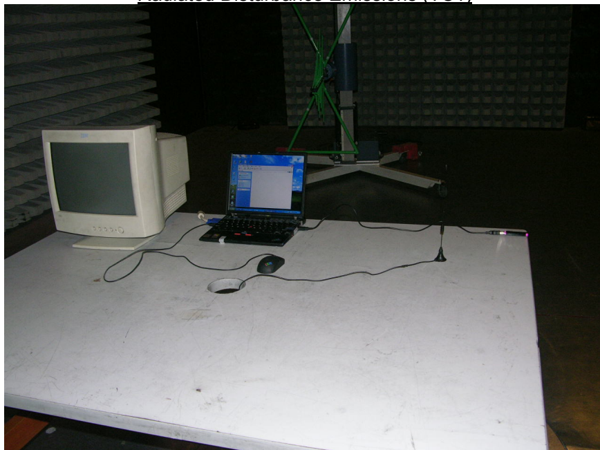
Radiated Disturbance Emissions (TC2)
