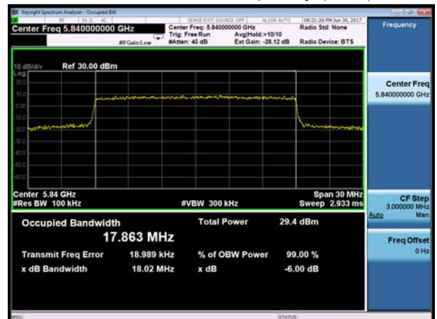
-6dB bandwidth, Carrier frequency (MHz): 5840
