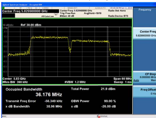
99% bandwidth, Carrier frequency (MHz): 5829.9
