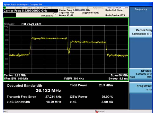
-6dB bandwidth, Carrier frequency (MHz):5829.9
