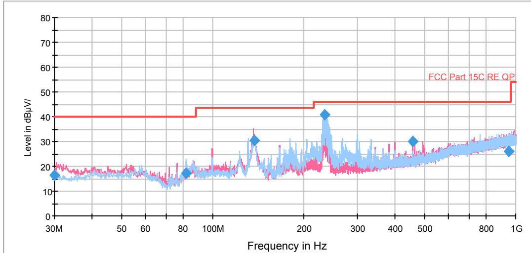
FCC RE 0.03-1GHz QP Class B
