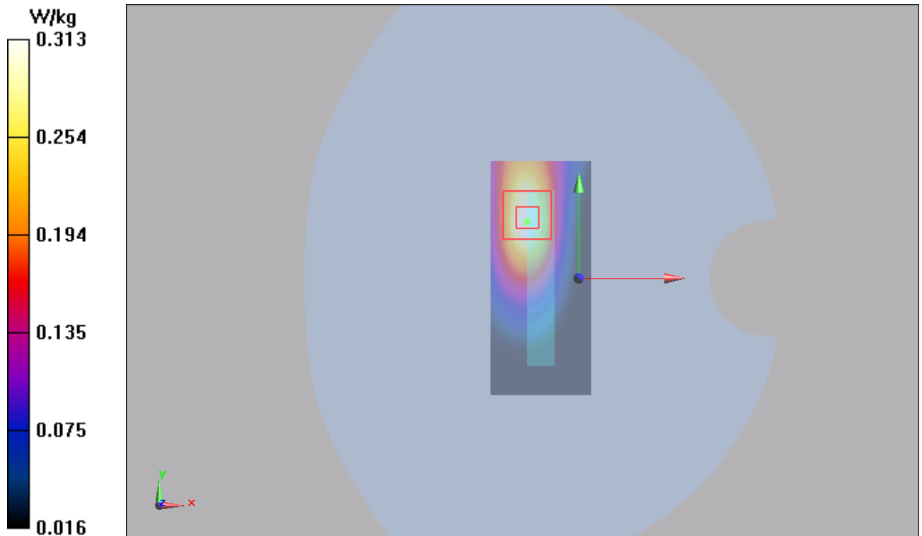
Figure 66 LTE Band 5 with Test Position 3 Channel 20525
