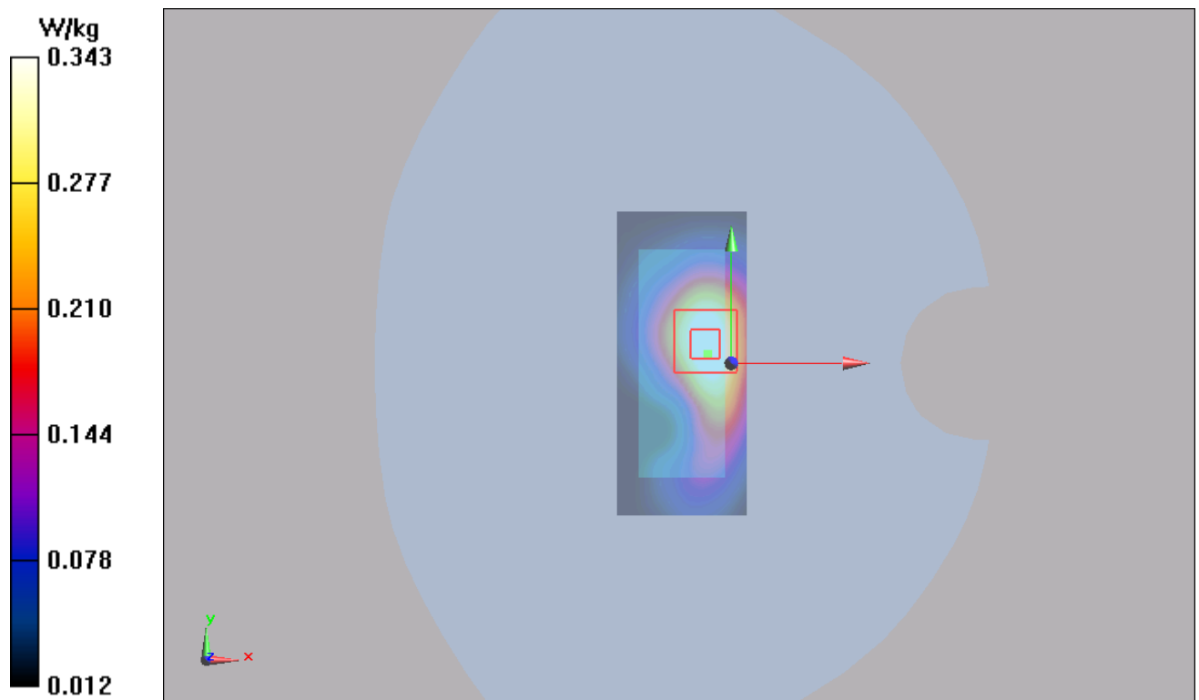
Figure 26 UMTS Band IV with Test Position 2 Channel 1413
