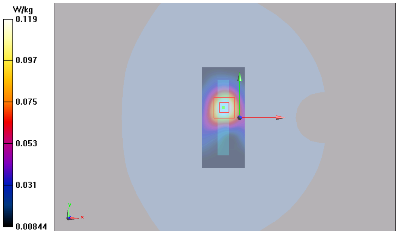
Figure 28 UMTS Band IV with Test Position 4 Channel 1413
