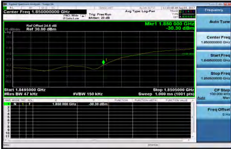
HSUPA_B2_LowCH9262-1852.4
