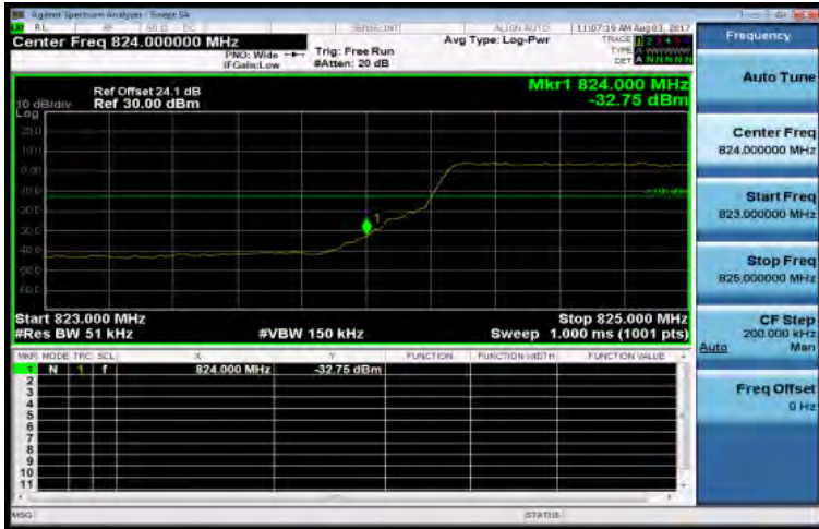
Band5_5MHz_QPSK_25_0_LowCH20425-826.5
