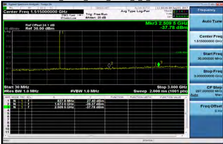
30MHz~3GHz_Band5_3MHz_QPSK_1_0_MidCH20525-836.5
