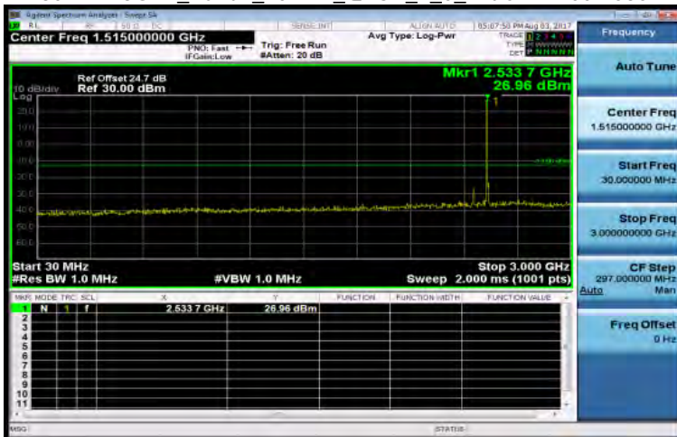
30MHz-3GHz_Band7_10MHz_QPSK_1_0_MidCH21100-2535
