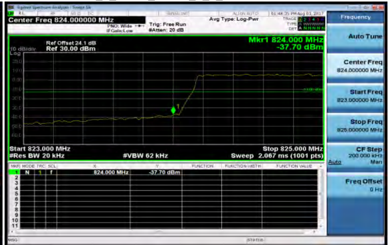
Band5_1_4MHz_QPSK_6_0_LowCH20407-824.7
