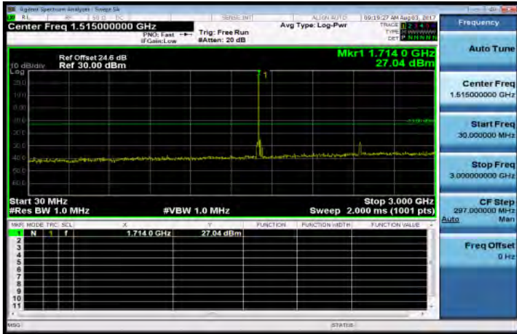
30MHz~3GHz_Band4_15MHz_QPSK_1_0_LowCH20025-1717.5
