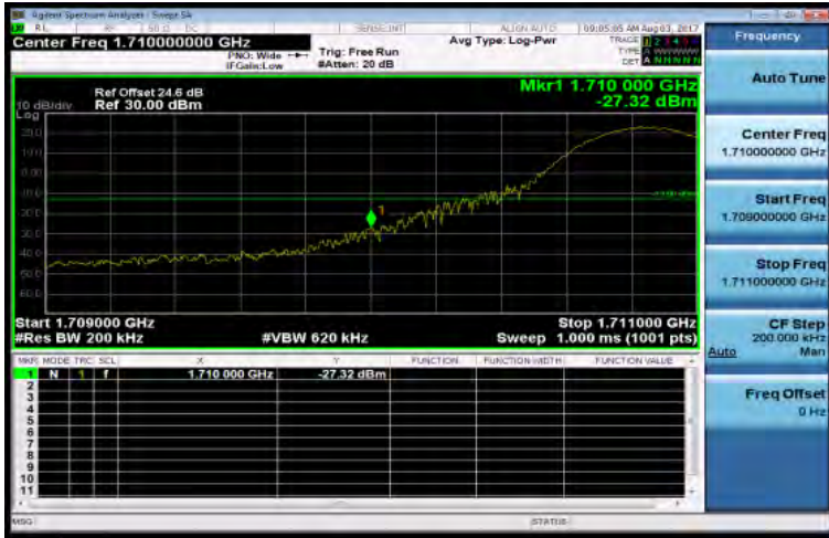
Band4_15MHz_QPSK_1_0_LowCH20025-1717.5
