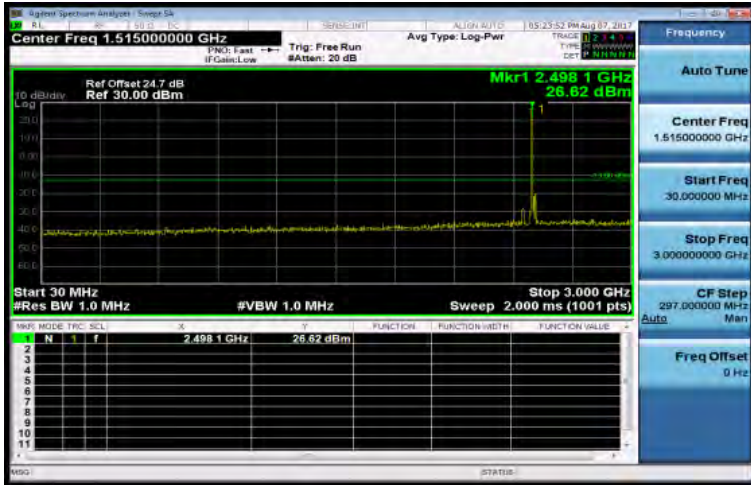
30MHz~3GHz_Band41_20MHz_QPSK_1_0_Low CH39750-2506
