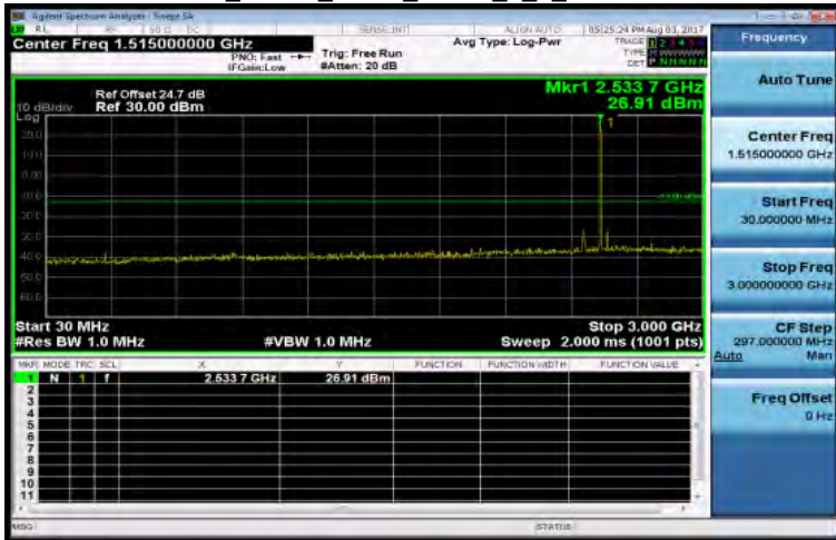
30MHz~3GHz_Band7_5MHz_QPSK_1_0_MidCH21100-2535
