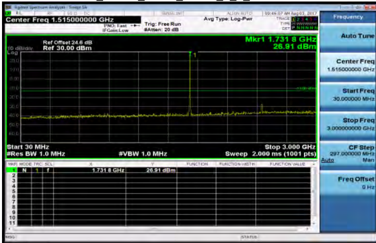
30MHz~3GHz_Band4_5MHz_QPSK_1_0_MidCH20175-1732.5
