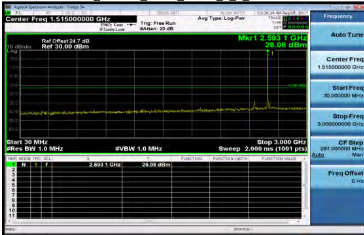
30MHz-3GHz_Band41_5MHz_QPSK_1_0_Mid CH40620-2593
