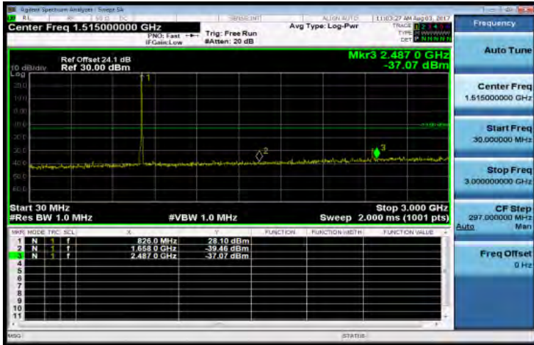
30MHz-3GHz_Band5_10MHz_QPSK_1_0_LowCH20450-829
