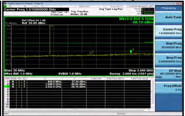
30MHz-3GHz_Band5_10MHz_QPSK_1_0_HighCH20600-844
