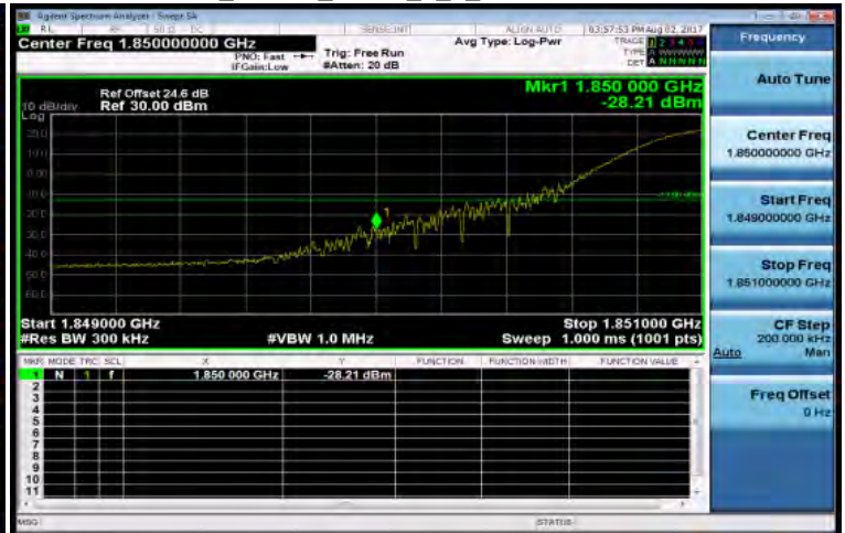
Band2_20MHz_QPSK_1_0_LowCH18700-1860
