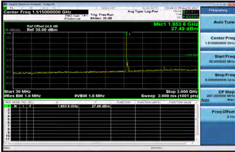
30MHz-3GHz_Band2_20MHz_QPSK_1_0_LowCH18700-1860
