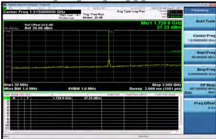
30MHz~3GHz_Band4_15MHz_QPSK_1_0_MidCH20175-1732.5
