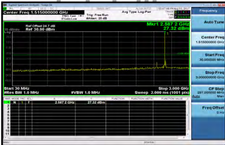
30MHz~3GHz_Band38_20MHz_QPSK_1_0_MidCH38000-2595
