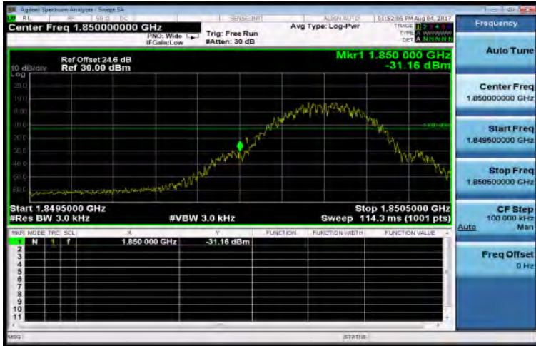
EDGE_1900MHz_LowCH512-1850.2
