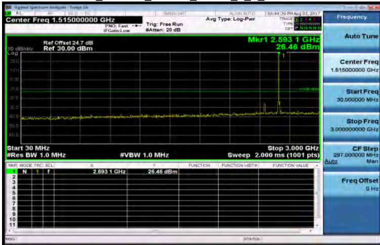
30MHz~3GHz_Band38_10MHz_QPSK_1_0_MidCH38000-2595
