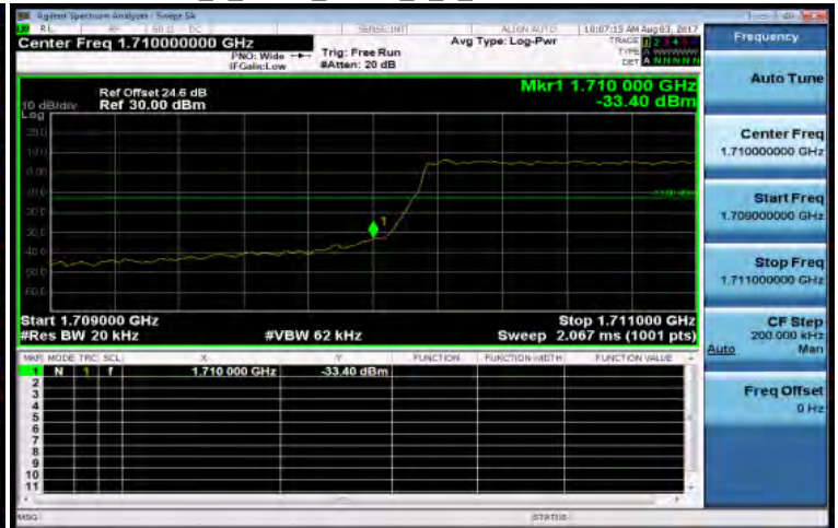
Band4_1_4MHz_QPSK_6_0_LowCH19957-1710.7
