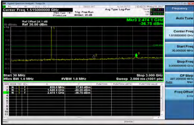
30MHz~3GHz_Band5_1_4MHz_QPSK_1_0_LowCH20407-824.7
