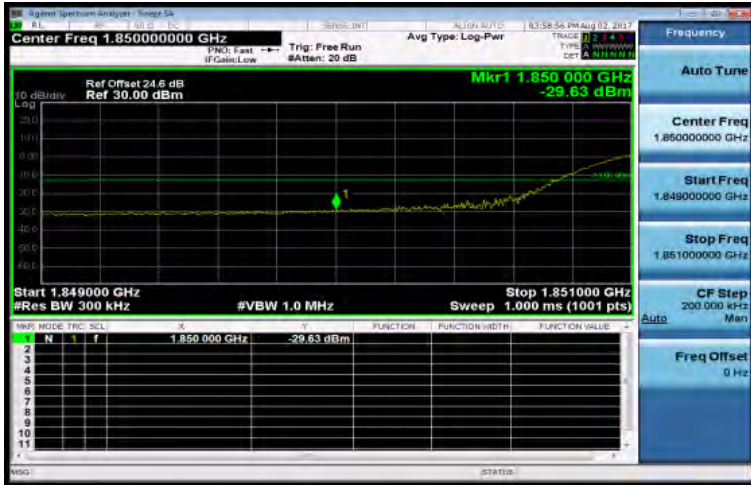
Band2_20MHz_QPSK_100_0_LowCH18700-1860
