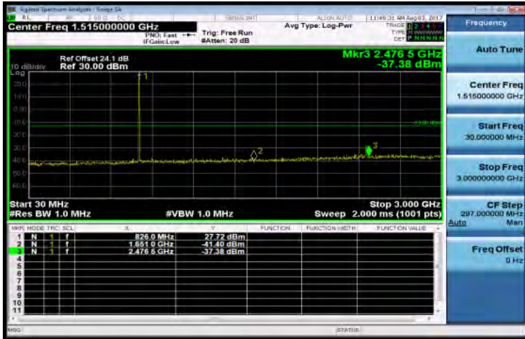
30MHz~3GHz_Band5_3MHz_QPSK_1_0_LowCH20415-825.5
