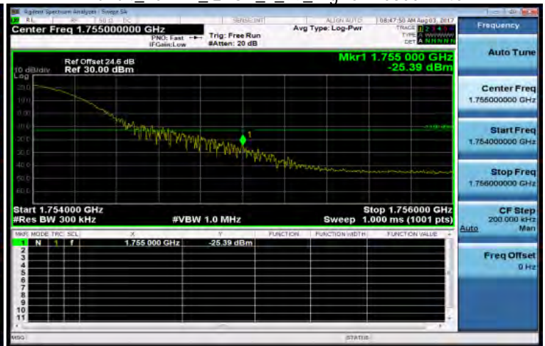
Band4_20MHz_QPSK_1_99_HighCH20300-1745
