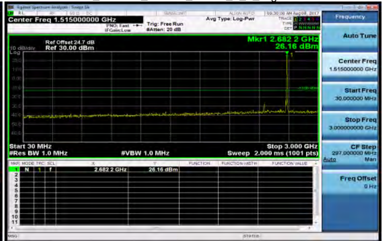
30MHz~3GHz_Band41_10MHz_QPSK_1_0_High CH41540-2685
