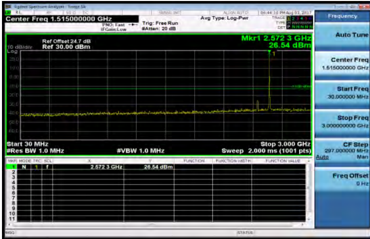
30MHz~3GHz_Band38_10MHz_QPSK_1_0_LowCH37800-2575
