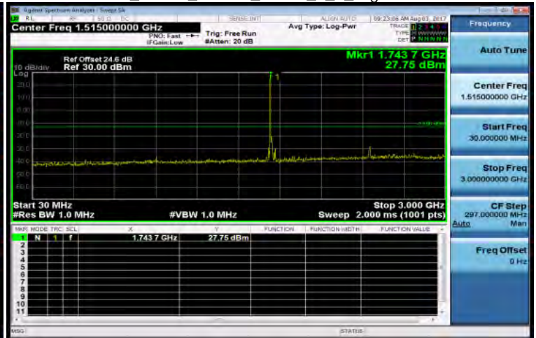
30MHz~3GHz_Band4_15MHz_QPSK_1_0_HighCH20325-1747.5
