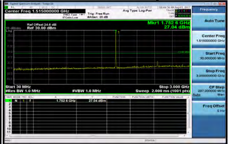
30MHz~3GHz_Band4_5MHz_QPSK_1_0_HighCH20375-1752.5
