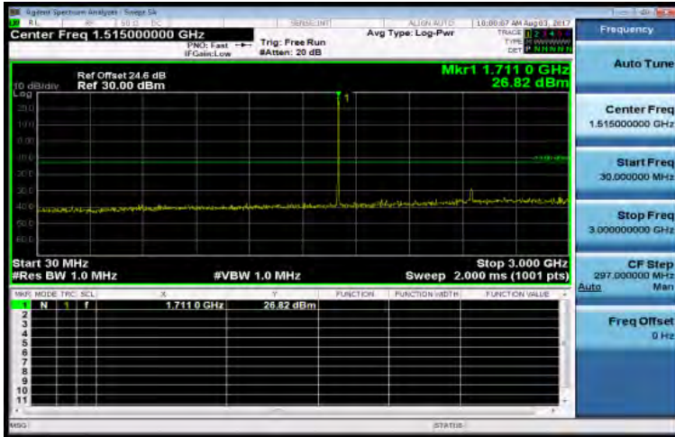
30MHz~3GHz_Band4_3MHz_QPSK_1_0_LowCH19965-1711.5
