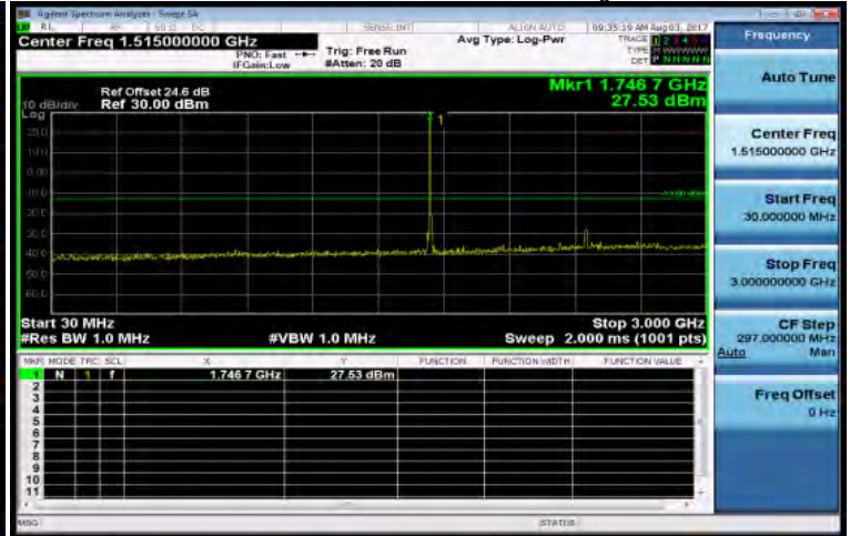
30MHz~3GHz_Band4_10MHz_QPSK_1_0_HighCH20350-1750
