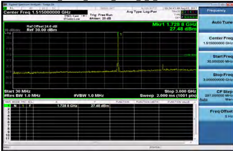
30MHz~3GHz_Band4_10MHz_QPSK_1_0_MidCH20175-1732.5
