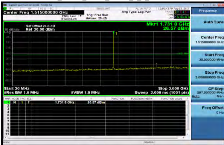
30MHz~3GHz_Band4_3MHz_QPSK_1_0_MidCH20175-1732.5
