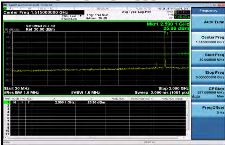
30MHz~3GHz_Band41_10MHz_QPSK_1_0_Mid CH40620-2593
