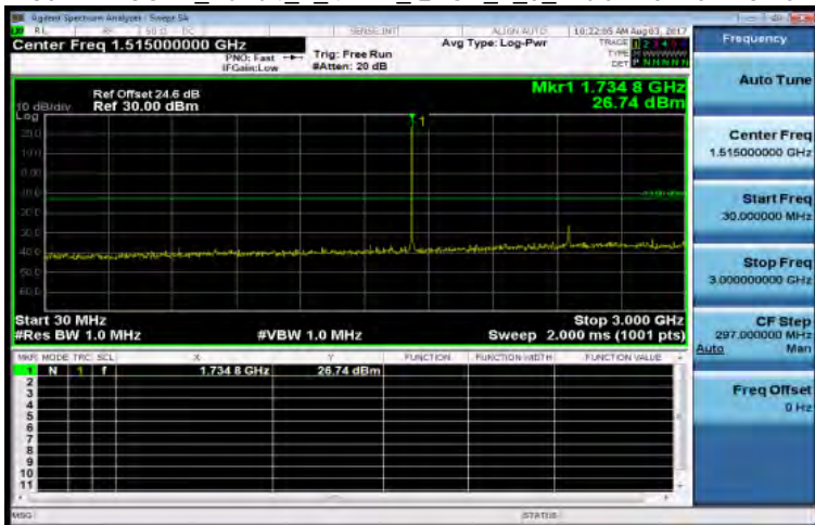
30MHz-3GHz_Band4_1_4MHz_QPSK_1_0_MidCH20175-1732.5
