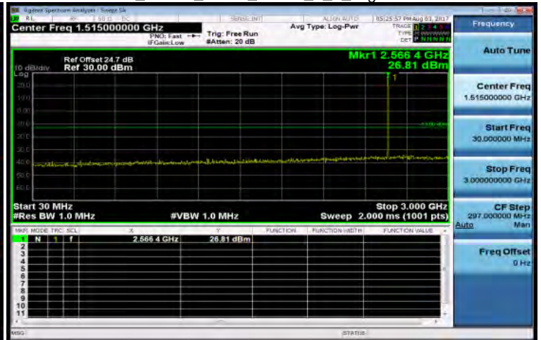
30MHz~3GHz_Band7_5MHz_QPSK_1_0_HighCH21425-2567.5
