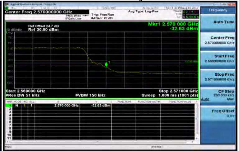
Band7_5MHz_QPSK_25_0_HighCH21425-2567.5
