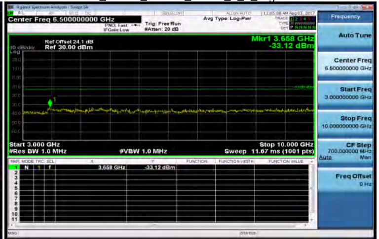
3GHz-10GHz_Band5_10MHz_QPSK_1_0_HighCH20600-844
