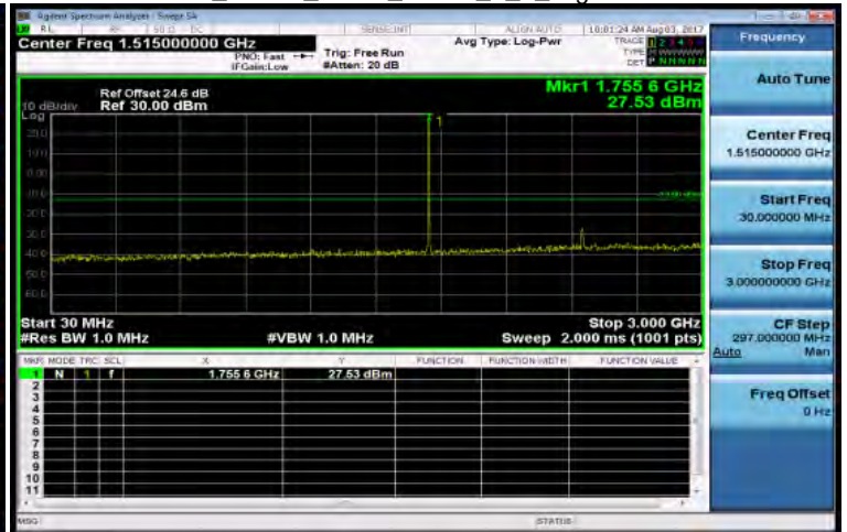
30MHz~3GHz_Band4_3MHz_QPSK_1_0_HighCH20385-1753.5
