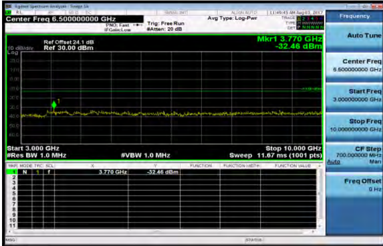
3GHz~10GHz_Band5_3MHz_QPSK_1_0_LowCH20415-825.5
