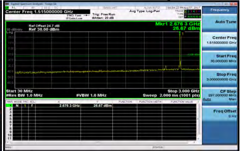
30MHz~3GHz_Band41_15MHz_QPSK_1_0_High CH41515-2682.5
