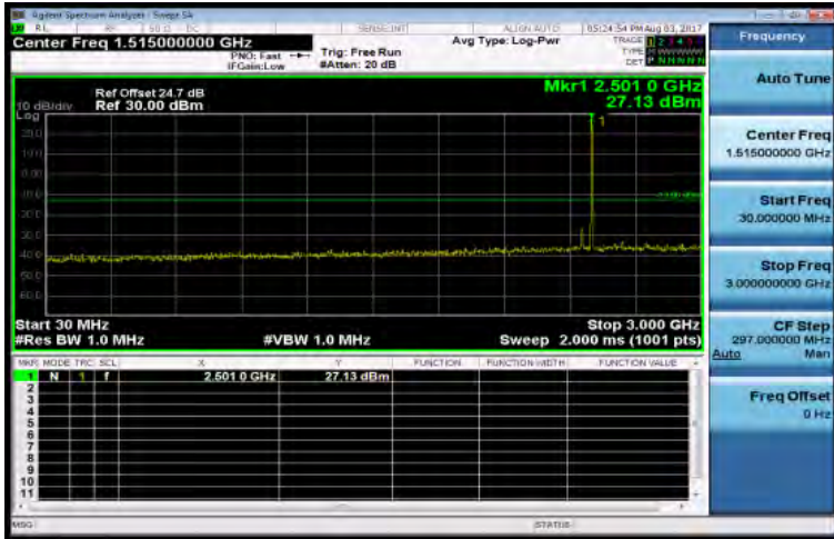
30MHz~3GHz_Band7_5MHz_QPSK_1_0_LowCH20775-2502.5
