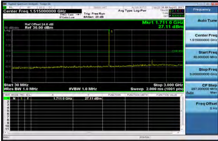
30MHz-3GHz_Band4_1_4MHz_QPSK_1_0_LowCH19957-1710.7
