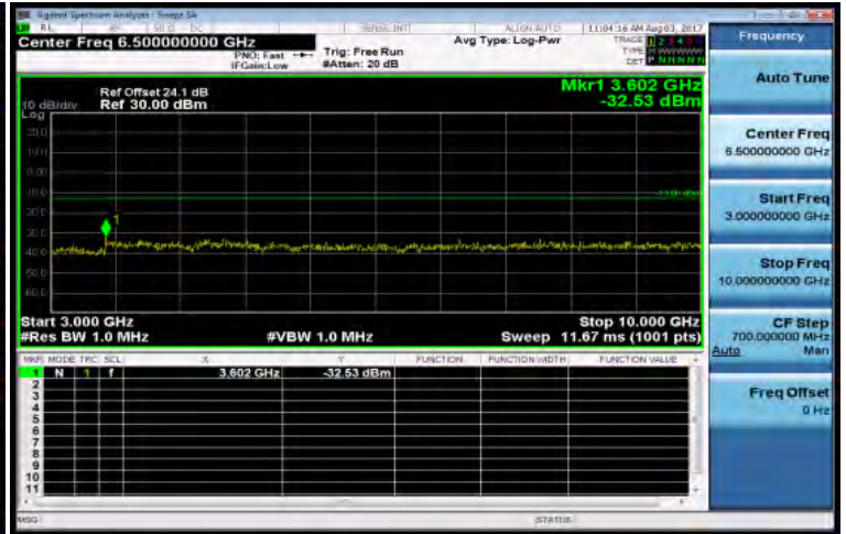
3GHz-10GHz_Band5_10MHz_QPSK_1_0_MidCH20525-836.5
