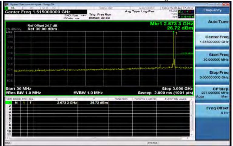
30MHz~3GHz_Band41_20MHz_QPSK_1_0_High CH41490-2680
