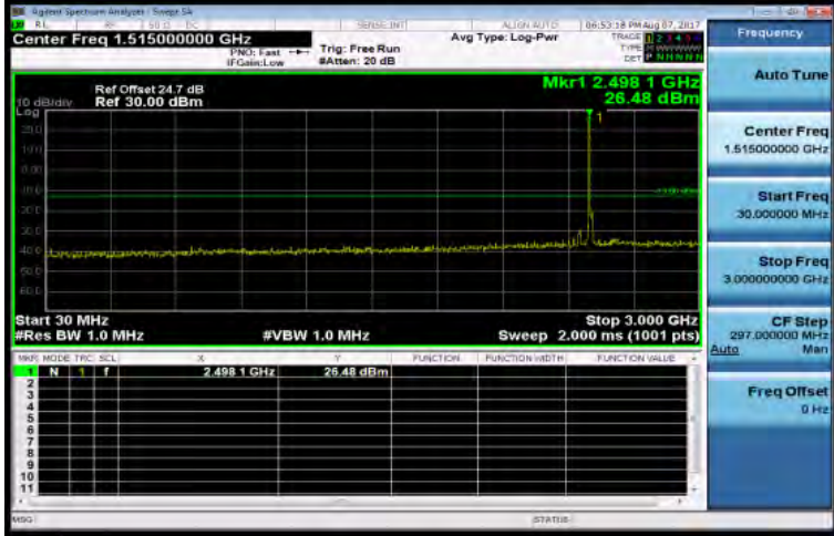
30MHz~3GHz_Band41_15MHz_QPSK_1_0_Low CH39725-2503.5
