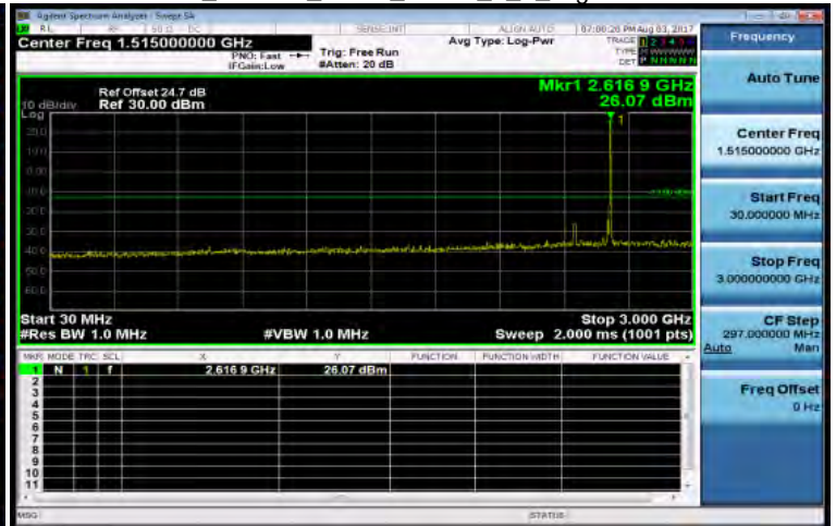
30MHz~3GHz_Band38_5MHz_QPSK_1_0_HighCH38225-2617.5
