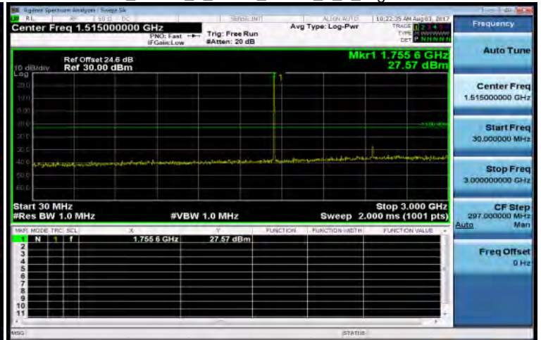
30MHz~3GHz_Band4_1_4MHz_QPSK_1_0_HighCH20393-1754.3
