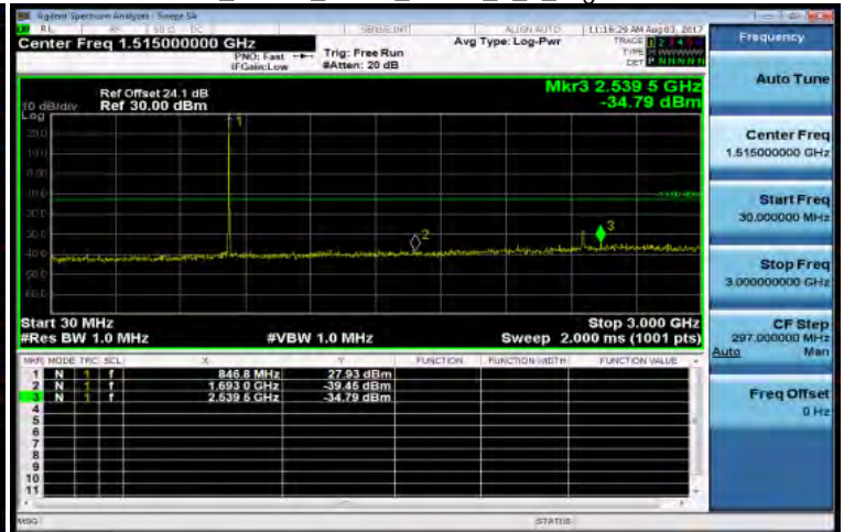
30MHz~3GHz_Band5_5MHz_QPSK_1_0_HighCH20625-846.5
