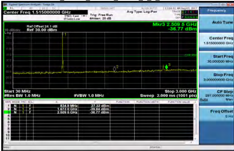
30MHz-3GHz_Band5_10MHz_QPSK_1_0_MidCH20525-836.5
