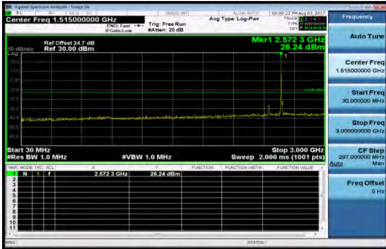
30MHz~3GHz_Band38_15MHz_QPSK_1_0_LowCH37825-2577.5
