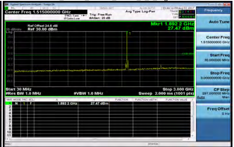
30MHz-3GHz_Band2_20MHz_QPSK_1_0_HighCH19100-1900
