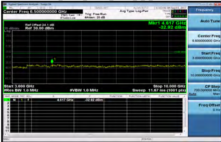
3GHz-10GHz_Band5_10MHz_QPSK_1_0_LowCH20450-829
