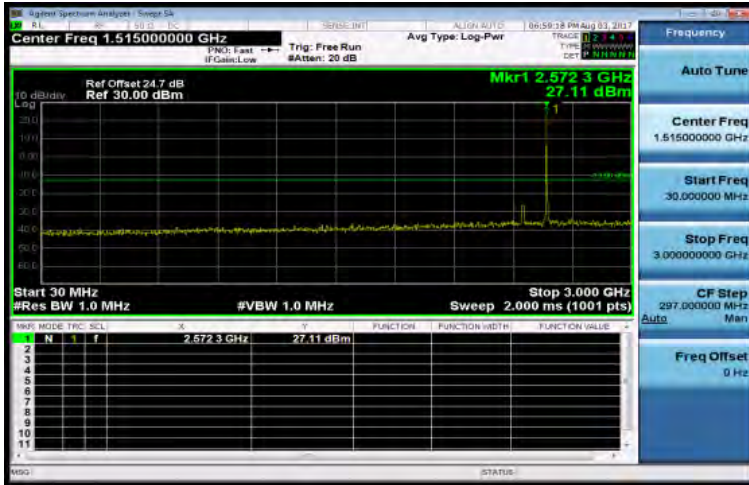
30MHz~3GHz_Band38_5MHz_QPSK_1_0_LowCH37775-2572.5
