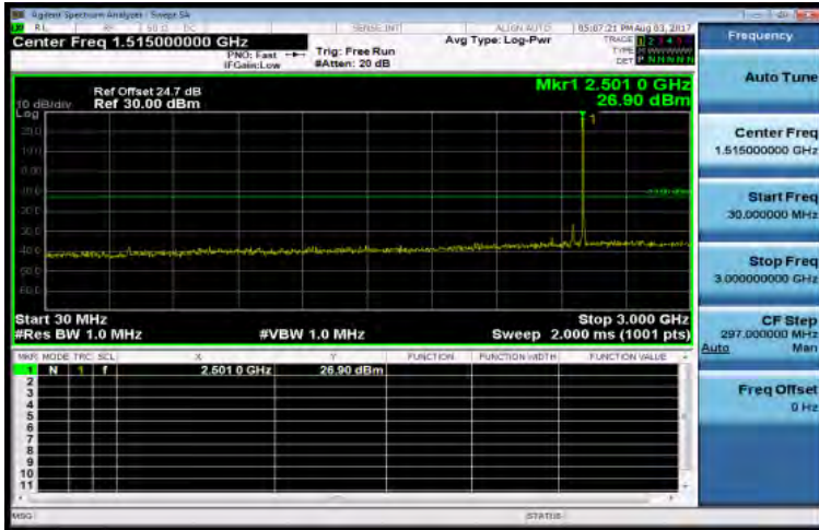
30MHz-3GHz_Band7_10MHz_QPSK_1_0_LowCH20800-2505
