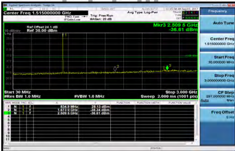
30MHz~3GHz_Band5_5MHz_QPSK_1_0_MidCH20525-836.5
