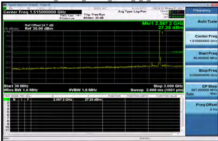
30MHz~3GHz_Band41_20MHz_QPSK_1_0_Mid CH40620-2593
