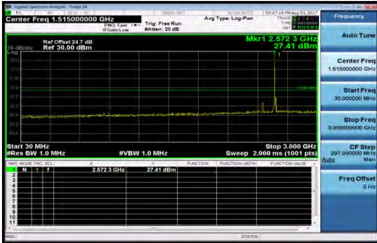
30MHz~3GHz_Band38_20MHz_QPSK_1_0_LowCH37850-2580
