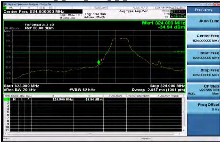
Band5_1_4MHz_QPSK_1_0_LowCH20407-824.7
