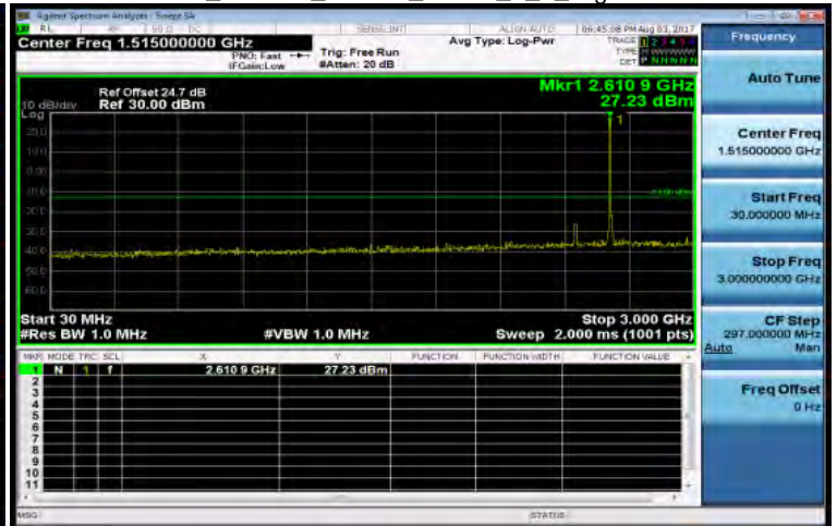
30MHz~3GHz_Band38_10MHz_QPSK_1_0_HighCH38200-2615
