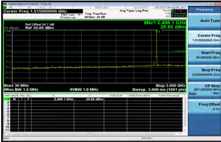
30MHz~3GHz_Band41_10MHz_QPSK_1_0_Low CH39700-2501
