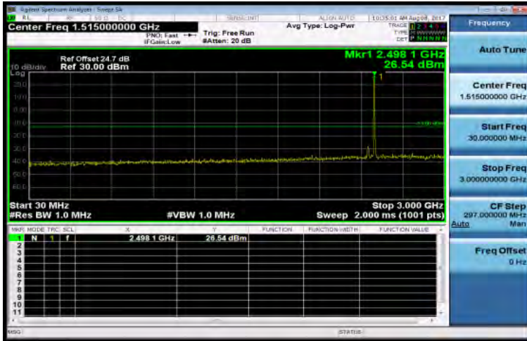
30MHz-3GHz_Band41_5MHz_QPSK_1_0_Low CH39675-2498.5
