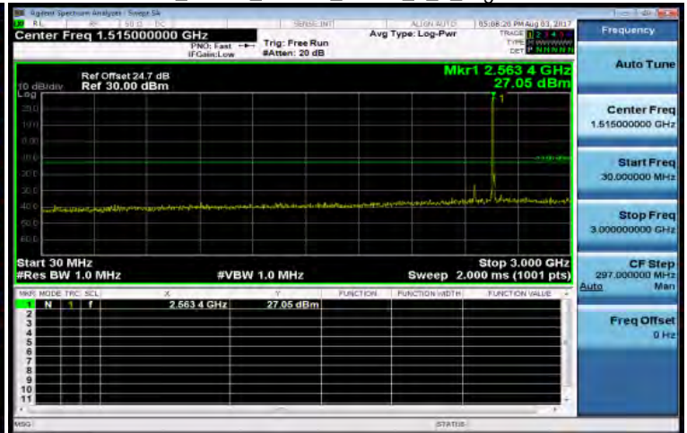
30MHz-3GHz_Band7_10MHz_QPSK_1_0_HighCH21400-2565
