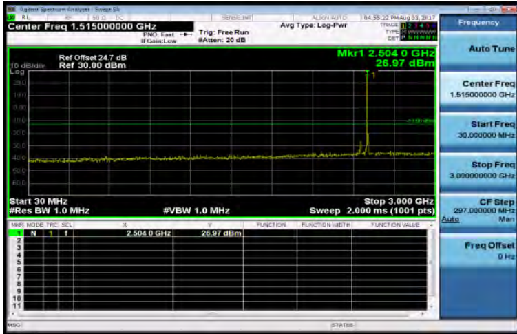
30MHz~3GHz_Band7_15MHz_QPSK_1_0_LowCH20825-2507.5
