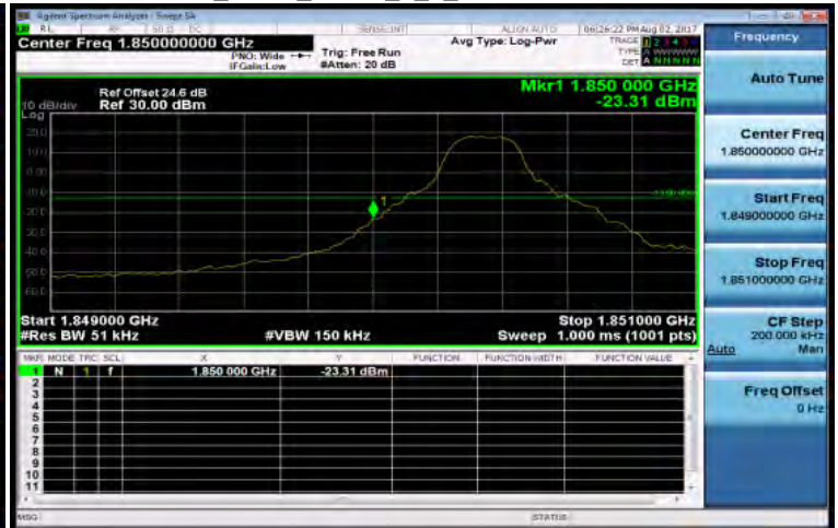
Band2_5MHz_QPSK_1_0_LowCH18625-1852.5
