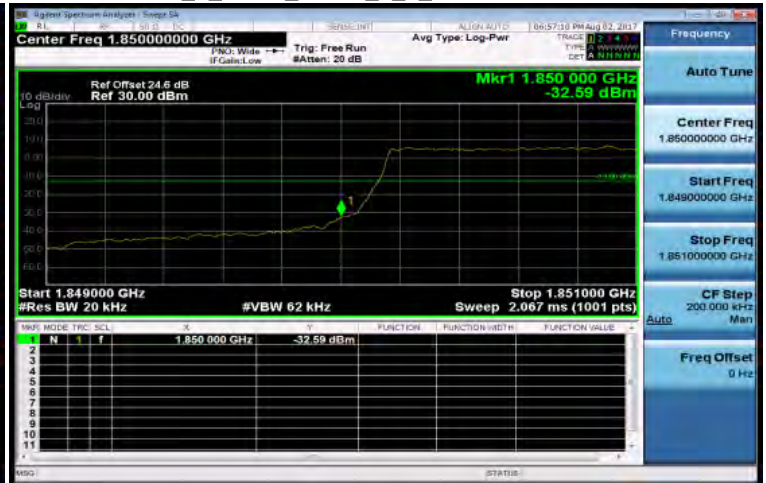
Band2_1_4MHz_QPSK_6_0_LowCH18607-1850.7
