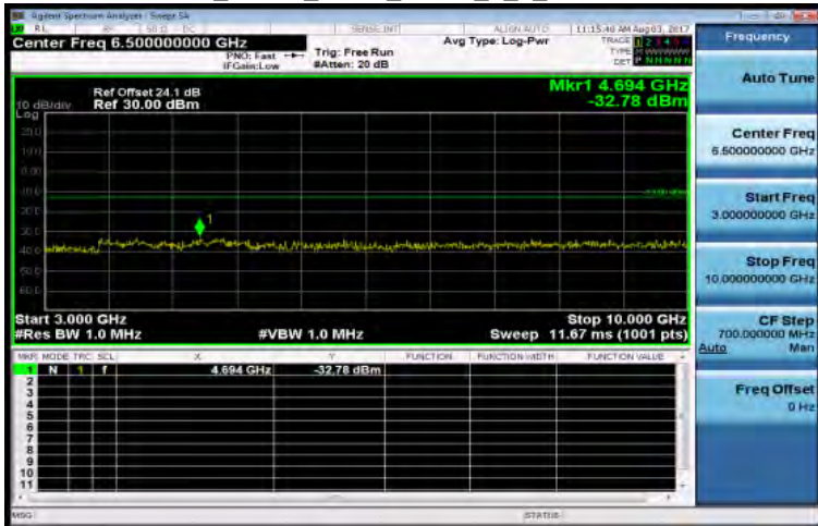
3GHz~10GHz_Band5_5MHz_QPSK_1_0_LowCH20425-826.5
