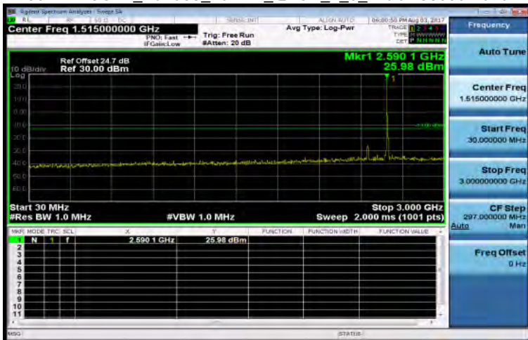
30MHz~3GHz_Band38_15MHz_QPSK_1_0_MidCH38000-2595
