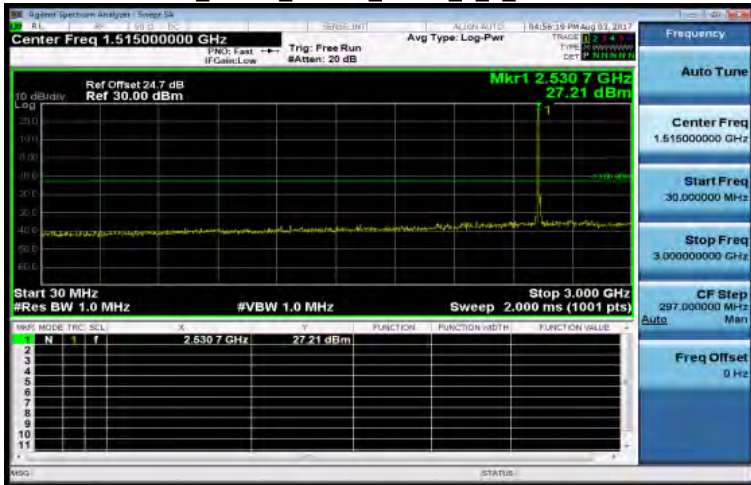
30MHz~3GHz_Band7_15MHz_QPSK_1_0_MidCH21100-2535
