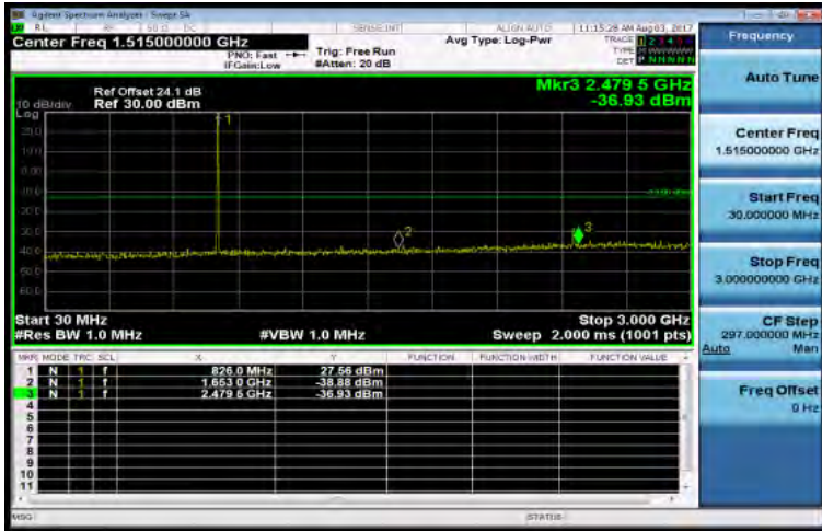
30MHz~3GHz_Band5_5MHz_QPSK_1_0_LowCH20425-826.5
