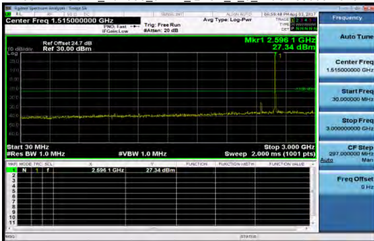
30MHz~3GHz_Band38_5MHz_QPSK_1_0_MidCH38000-2595
