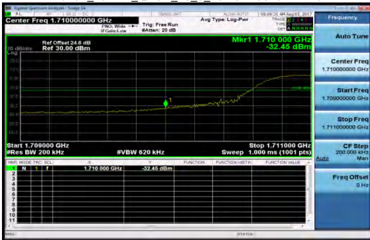
Band4_15MHz_QPSK_75_0_LowCH20025-1717.5
