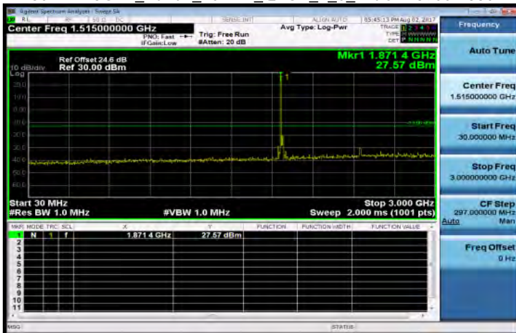
30MHz-3GHz_Band2_20MHz_QPSK_1_0_MidCH18900-1880
