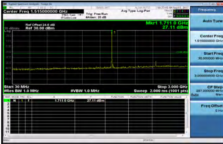
30MHz~3GHz_Band4_10MHz_QPSK_1_0_LowCH20000-1715
