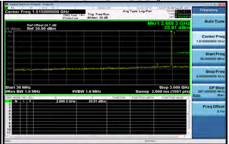
30MHz-3GHz_Band41_5MHz_QPSK_1_0_High CH41565-2687.5
