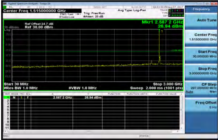
30MHz~3GHz_Band41_15MHz_QPSK_1_0_Mid CH40620-2593
