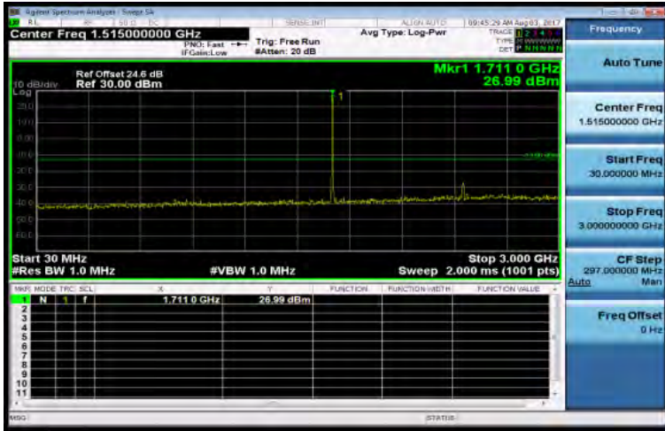
30MHz~3GHz_Band4_5MHz_QPSK_1_0_LowCH19975-1712.5
