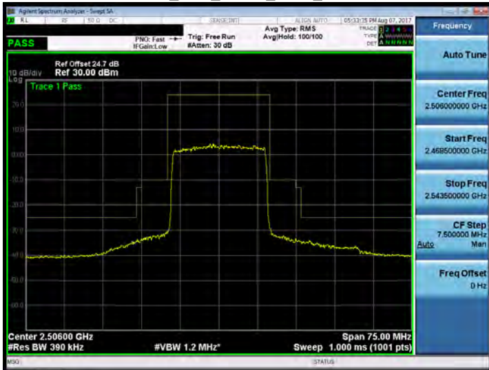
Band 41_20M_QPSK_MID_RB1,0
