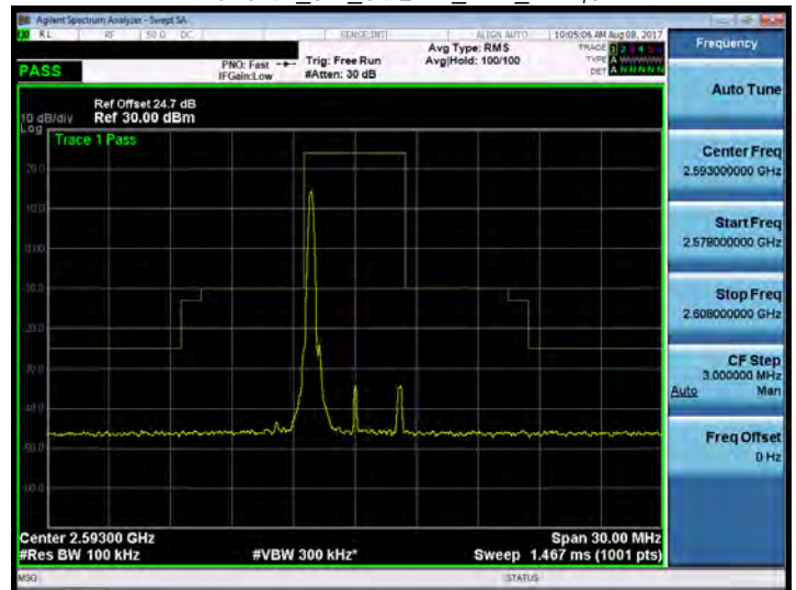
Band 41_5M_64QAM_MID_RB1,0
