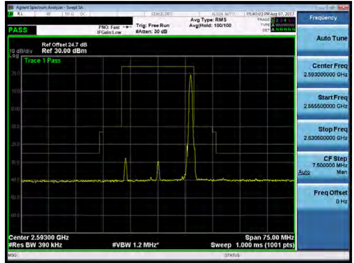
Band 41_20M_QPSK_MID_RB100,0
