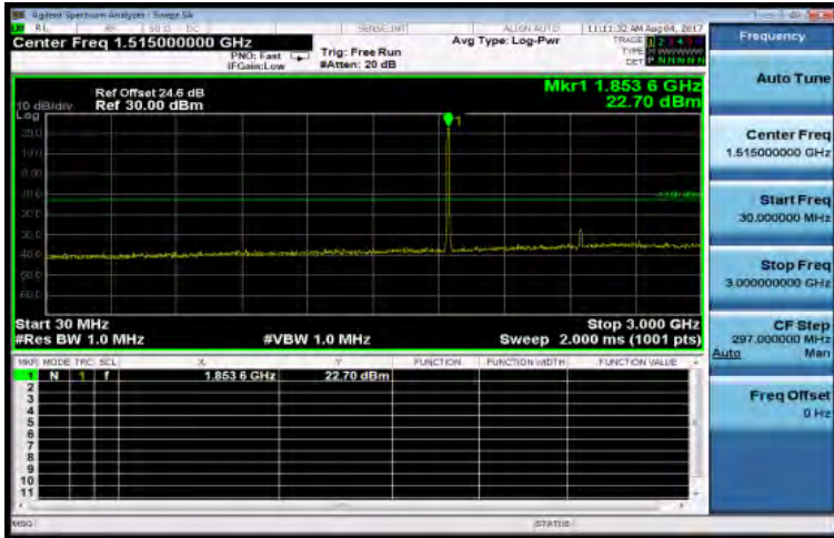
30MHz~3GHz_HSUPA_B2_LowCH9262-1852.4
