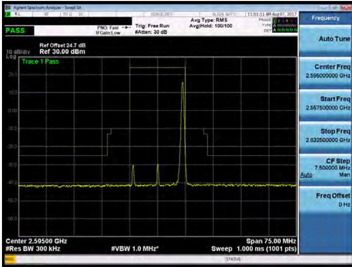
Band 38_15M_64QAM_MID_RB75,0
