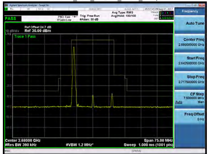
Band 41_20M_64QAM_HIGH_RB1,0
