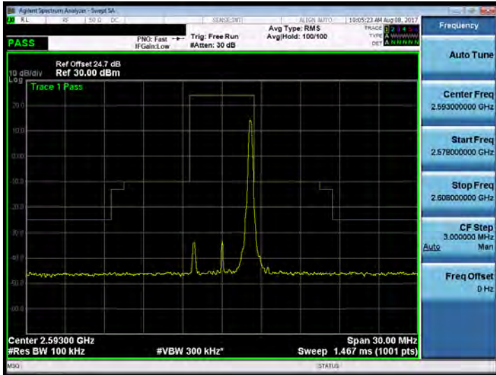
Band 41_5M_64QAM_MID_RB25,0
