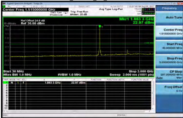
30MHz~3GHz_HSDPA_B2_MidCH9400-1880
