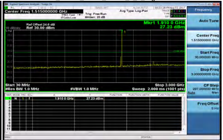
30MHz~3GHz_Band2_3MHz_QPSK_1_0_HighCH19185-1908.5
