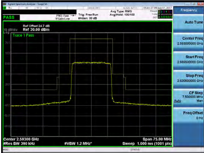
Band 41_20M_16QAM_HIGH_RB1,0
