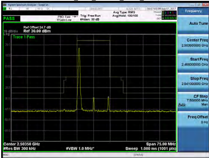
Band 41_15M_64QAM_LOW_RB1,0
