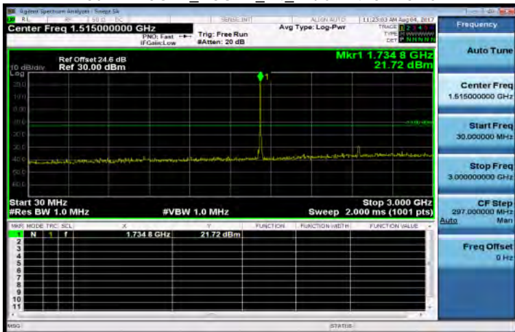
30MHz~3GHz_HSUPA_B4_MidCH1413-1732.6
