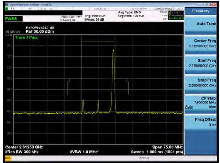
Band 38_15M_64QAM_HIGH_RB75,0
