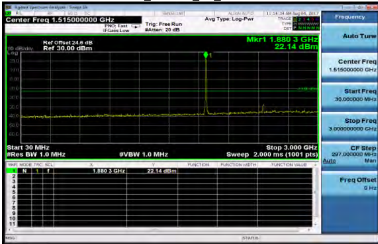
30MHz~3GHz_HSUPA_B2_MidCH9400-1880
