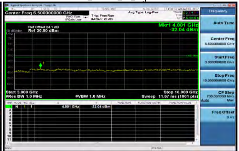
3GHz~10GHz_HSUPA_B5_HighCH4233-846.6
