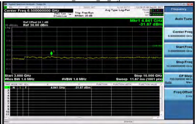
3GHz~10GHz_HSDPA_B5_HighCH4233-846.6
