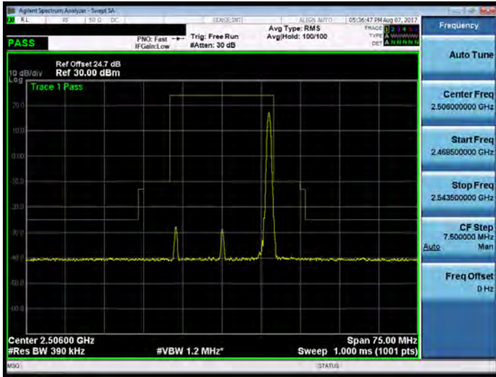
Band 41_20M_64QAM_LOW_RB100,0
