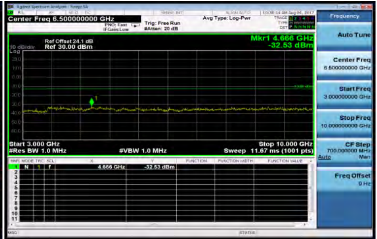
3GHz~10GHz_WCDMA_B5_MidCH4183-836.6
