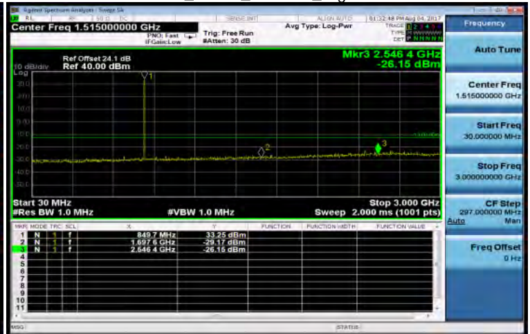
30MHz~3GHz_EDGE_850MHz_HighCH251-848.8
