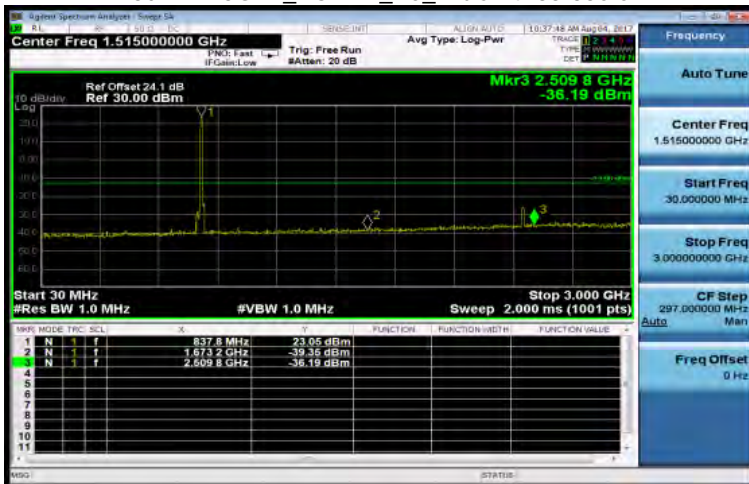
30MHz~3GHz_HSDPA_B5_MidCH4183-836.6
