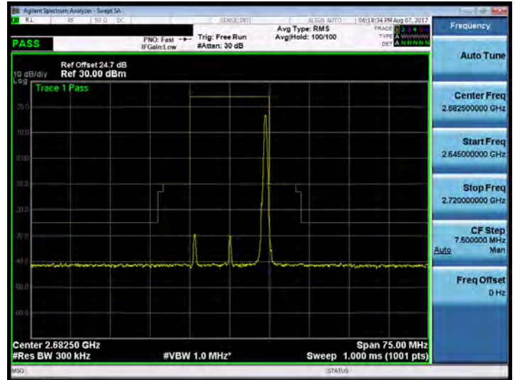
Band 41_15M_64QAM_HIGH_RB75,0
