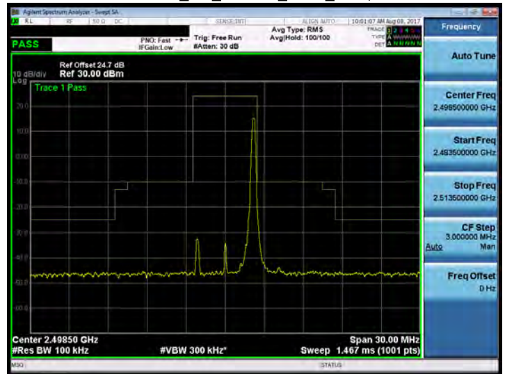
Band 41_5M_64QAM_LOW_RB25,0
