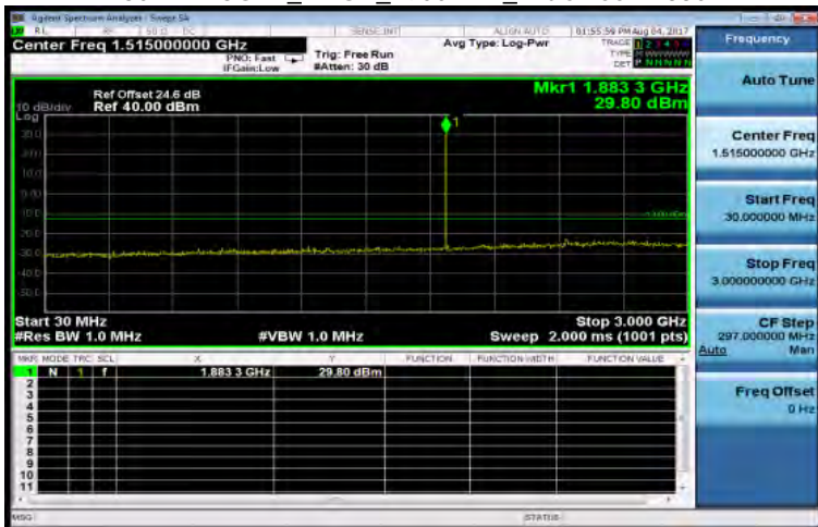
30MHz~3GHz_EDGE_1900MHz_MidCH661-1880
