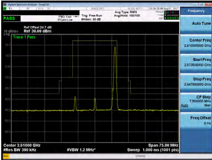
Band 38_20M_QPSK_HIGH_RB100,0
