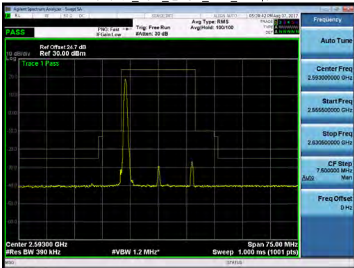
Band 41_20M_QPSK_MID_RB1,0
