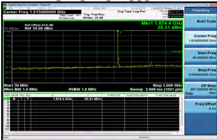
30MHz~3GHz_Band2_15MHz_QPSK_1_0_MidCH1890-1880
