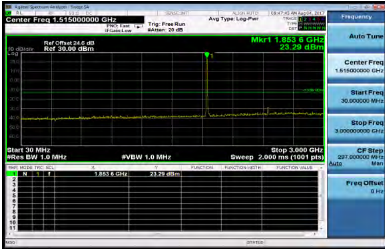
30MHz~3GHz_WCDMA_B2_LowCH9262-1852.4
