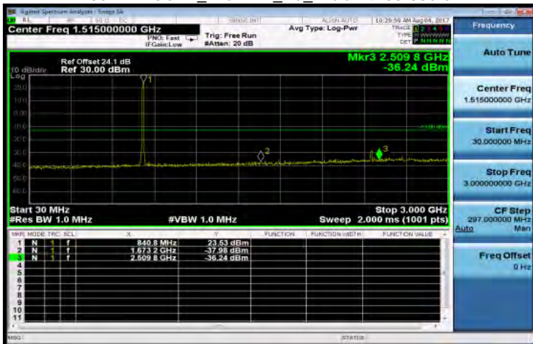
30MHz~3GHz_WCDMA_B5_MidCH4183-836.6
