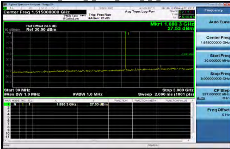
30MHz~3GHz_Band2_1_4MHz_QPSK_1_0_MidCH18900-1880
