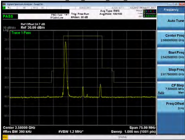
Band 38_20M_16QAM_LOW_RB1,0
