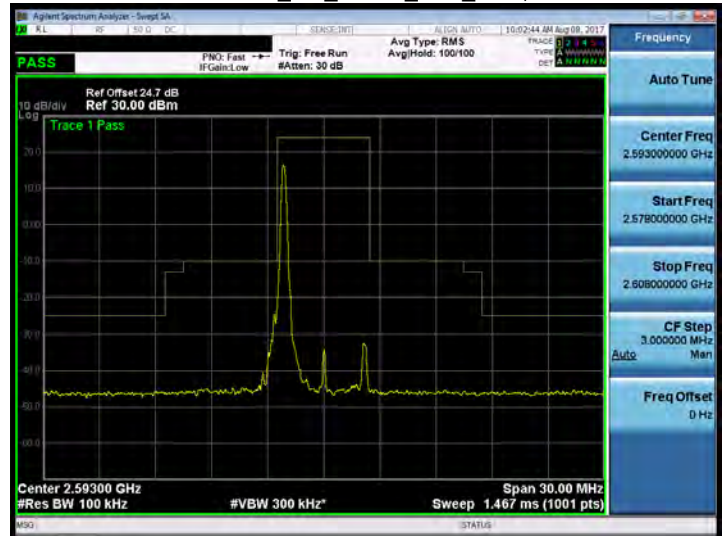
Band 41_5M_QPSK_MID_RB1,0
