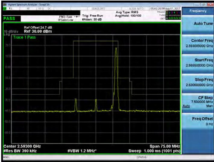
Band 41_20M_16QAM_MID_RB100,0
