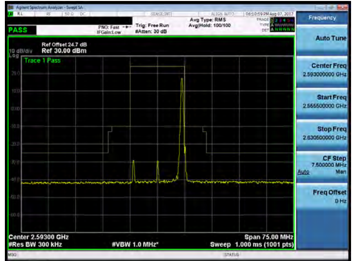
Band 41_15M_16QAM_MID_RB75,0
