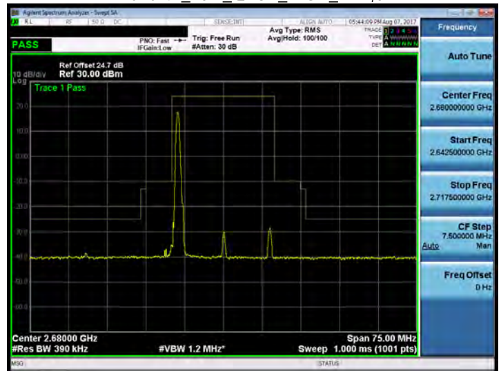
Band 41_20M_QPSK_HIGH_RB1,0
