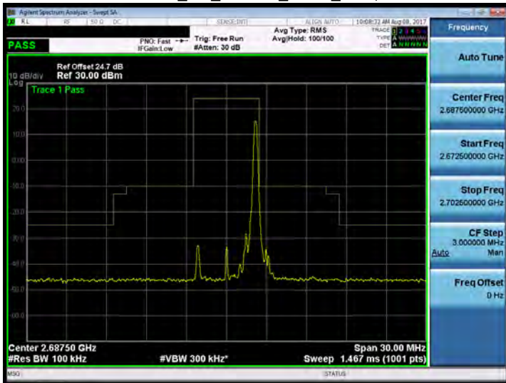
Band 41_5M_16QAM_HIGH_RB25,0
