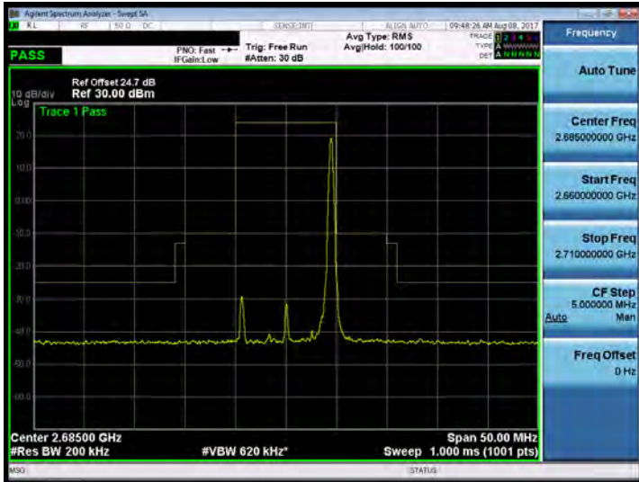
Band 41_10M_QPSK_HIGH_RB50,0
