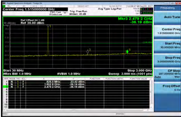
30MHz~3GHz_WCDMA_B5_LowCH4132-826.4
