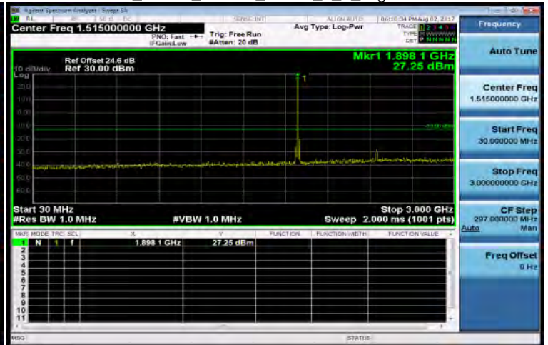
30MHz~3GHz_Band2_15MHz_QPSK_1_0_HighCH19125-1902.5
