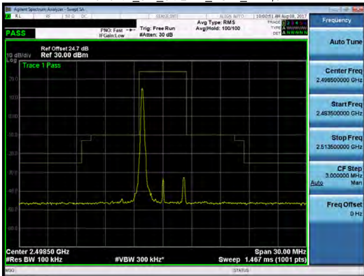
Band 41_5M_64QAM_LOW_RB1,0
