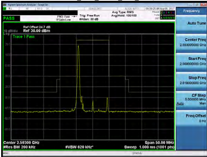
Band 41_10M_QPSK_MID_RB1,0
