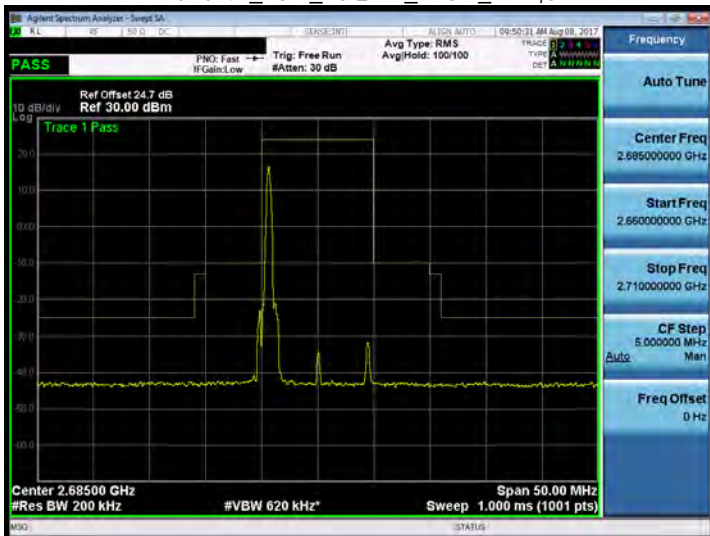
Band 41_10M_16QAM_HIGH_RB1,0
