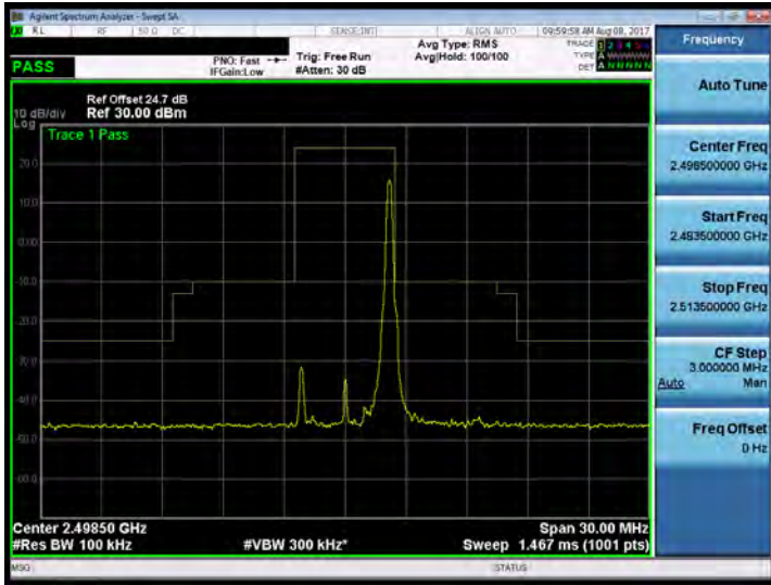
Band 41_5M_16QAM_LOW_RB25,0
