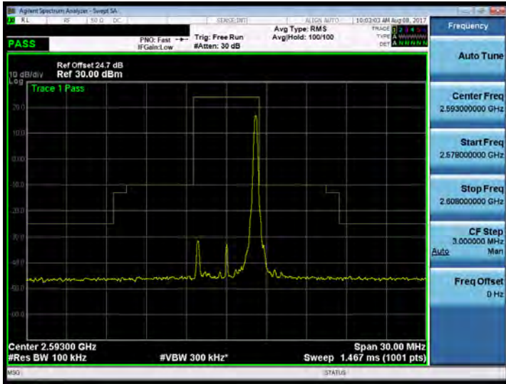
Band 41_5M_QPSK_MID_RB25,0
