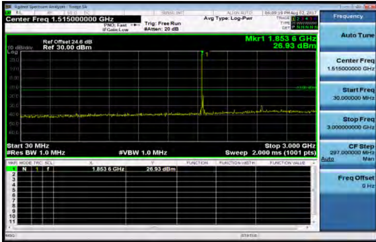
30MHz~3GHz_Band2_15MHz_QPSK_1_0_LowCH18675-1857.5
