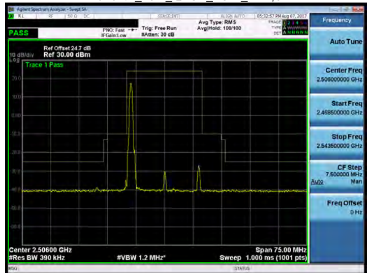
Band 41_20M_QPSK_LOW_RB1,0
