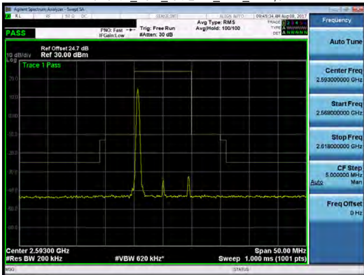
Band 41_10M_64QAM_MID_RB1,0
