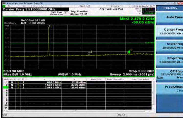
30MHz~3GHz_HSUPA_B5_LowCH4132-826.4
