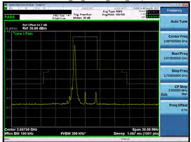
Band 41_5M_16QAM_HIGH_RB1,0
