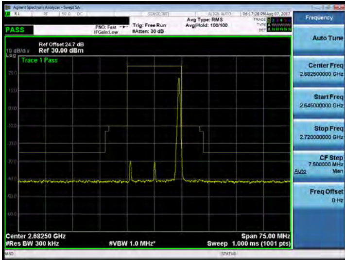
Band 41_15M_16QAM_HIGH_RB75,0
