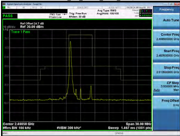
Band 41_5M_QPSK_LOW_RB1,0
