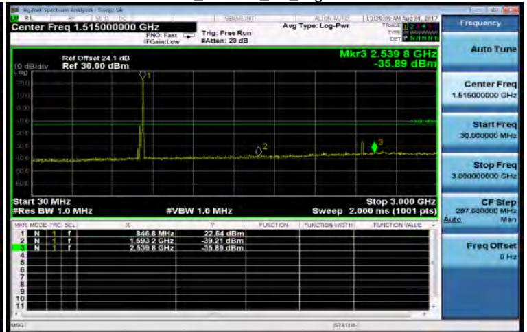
30MHz~3GHz_HSDPA_B5_HighCH4233-846.6
