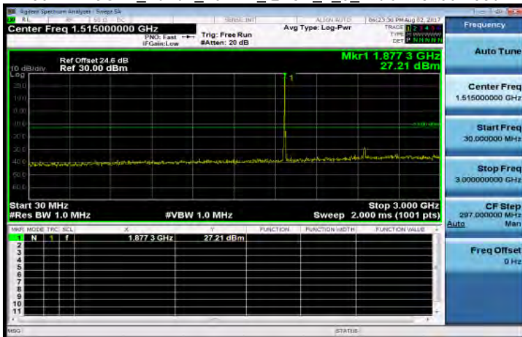
30MHz-3GHz_Band2_10MHz_QPSK_1_0_MidCH1890-1880
