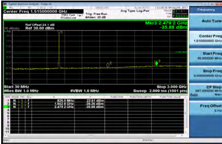
30MHz~3GHz_HSDPA_B5_LowCH4132-826.4
