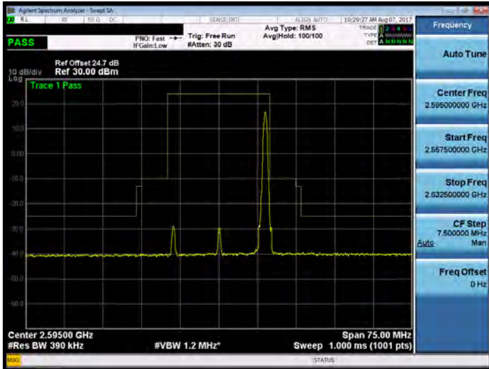
Band 38_20M_16QAM_MID_RB100,0
