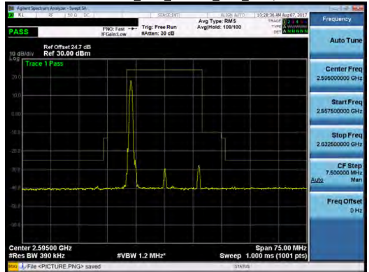
Band 38_20M_16QAM_MID_RB1,0
