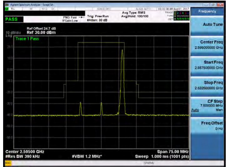
Band 38_20M_64QAM_MID_RB100,0
