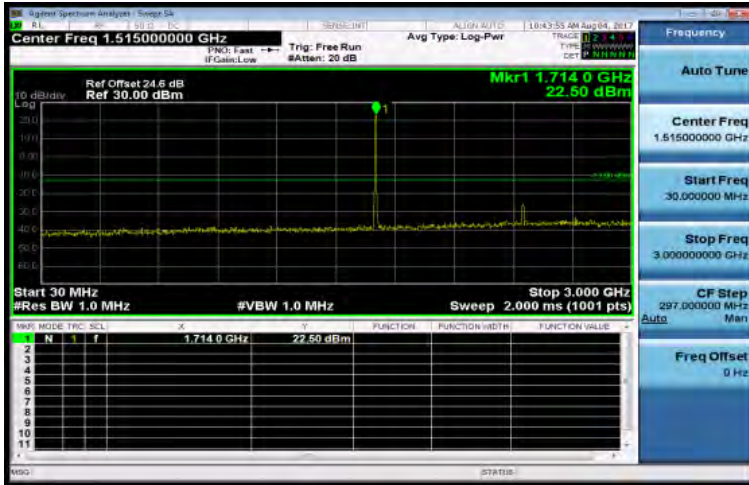
30MHz~3GHz_HSDPA_B4_LowCH1312-1712.4
