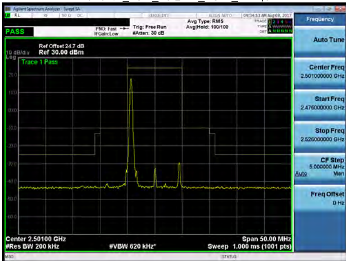
Band 41_10M_16QAM_LOW_RB1,0
