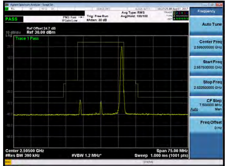
Band 38_20M_QPSK_MID_RB100,0
