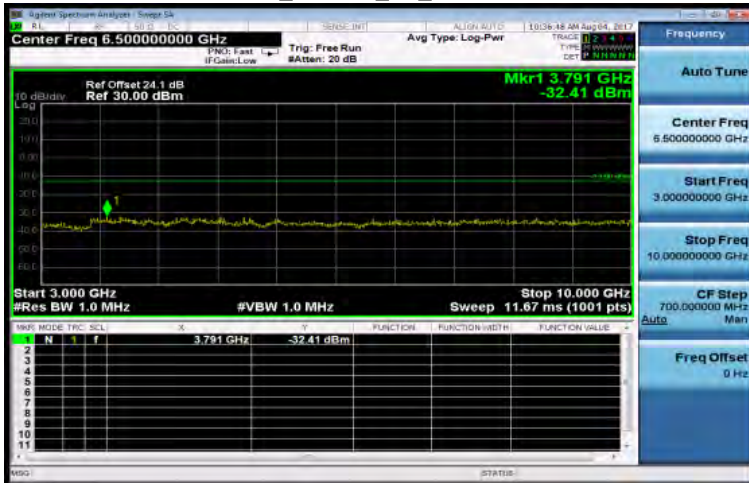
3GHz~10GHz_HSDPA_B5_LowCH4132-826.4
