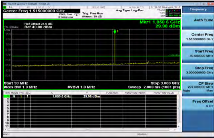
30MHz~3GHz_GPRS_1900MHz_LowCH512-1850.2
