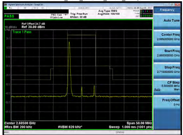
Band 41_10M_64QAM_HIGH_RB1,0
