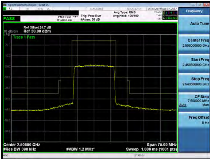
Band 41_20M_64QAM_MID_RB1,0
