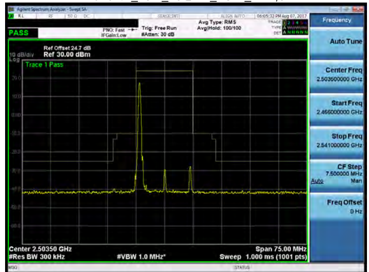
Band 41_15M_16QAM_LOW_RB1,0
