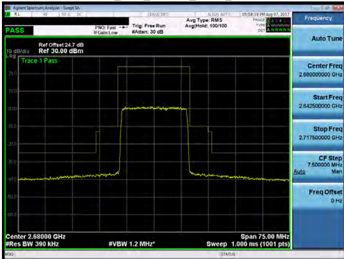
Band 41_20M_64QAM_HIGH_RB100,0
