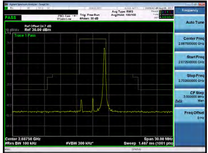
Band 41_5M_64QAM_HIGH_RB25,0
