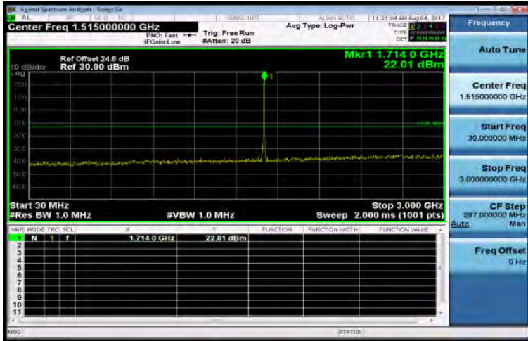
30MHz~3GHz_HSUPA_B4_LowCH1312-1712.4
