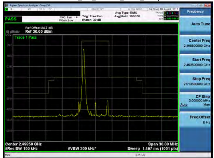
Band 41_5M_16QAM_LOW_RB1,0
