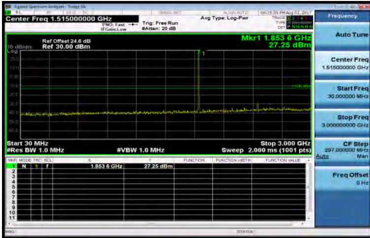
30MHz~3GHz_Band2_5MHz_QPSK_1_0_LowCH18625-1852.5
