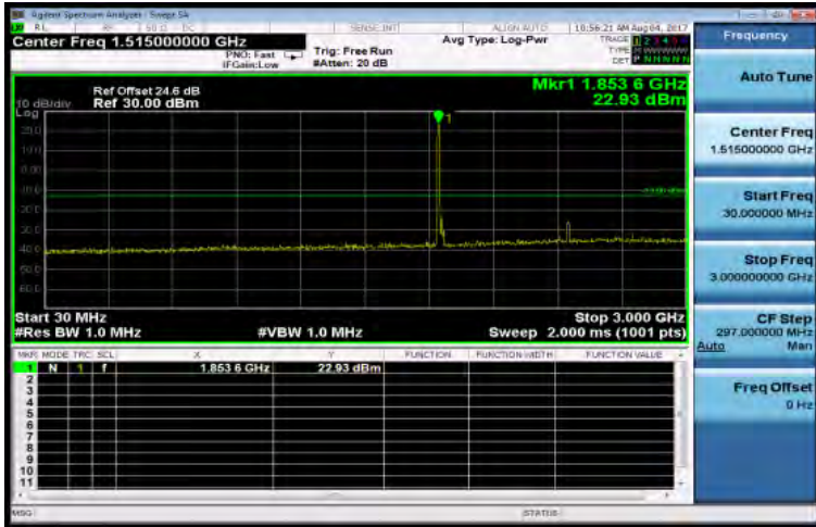
30MHz~3GHz_HSDPA_B2_LowCH9262-1852.4
