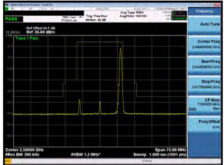
Band 38_20M_16QAM_LOW_RB100,0
