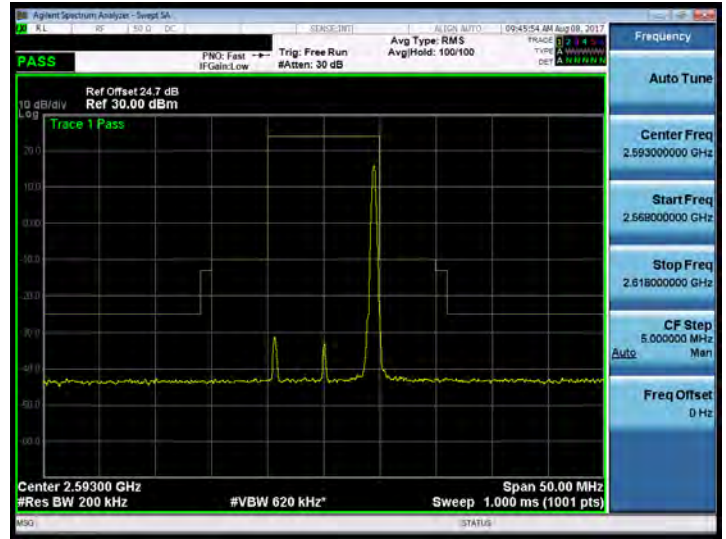
Band 41_10M_64QAM_MID_RB50,0
