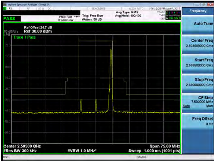
Band 41_15M_64QAM_MID_RB75,0
