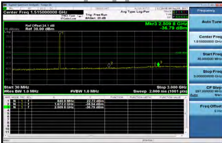
30MHz~3GHz_HSUPA_B5_MidCH4183-836.6
