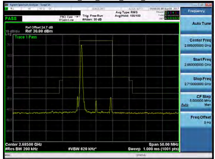
Band 41_10M_QPSK_HIGH_RB1,0
