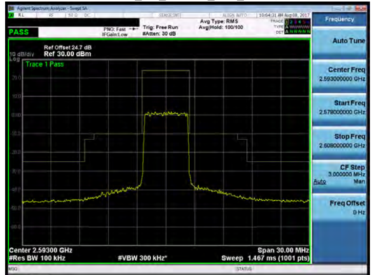
Band 41_5M_16QAM_HIGH_RB1,0
