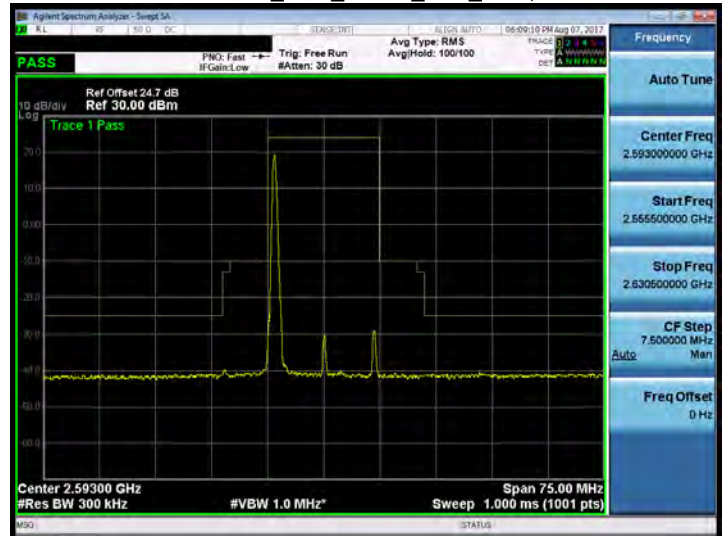
Band 41_15M_QPSK_MID_RB1,0
