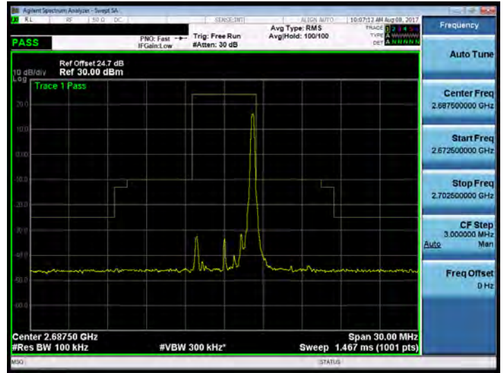
Band 41_5M_QPSK_HIGH_RB25,0
