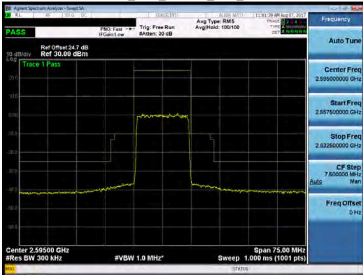
Band 38_15M_64QAM_HIGH_RB1,0
