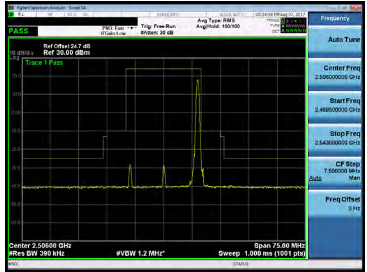
Band 41_20M_16QAM_LOW_RB100,0
