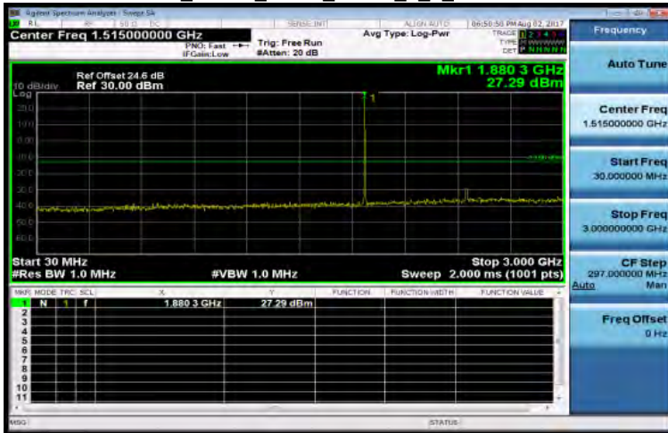
30MHz~3GHz_Band2_3MHz_QPSK_1_0_MidCH18900-1880
