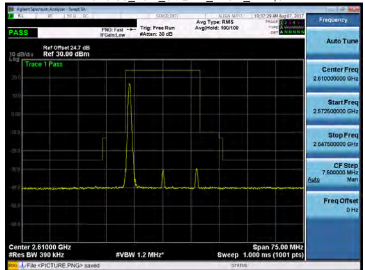
Band 38_20M_64QAM_HIGH_RB1,0
