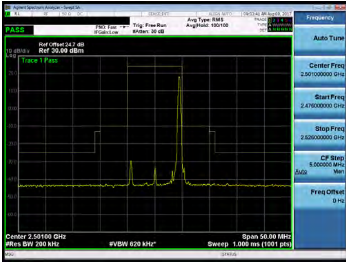
Band 41_10M_QPSK_LOW_RB50,0
