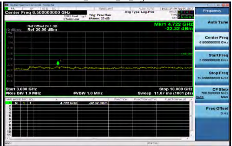
3GHz~10GHz_WCDMA_B5_HighCH4233-846.6
