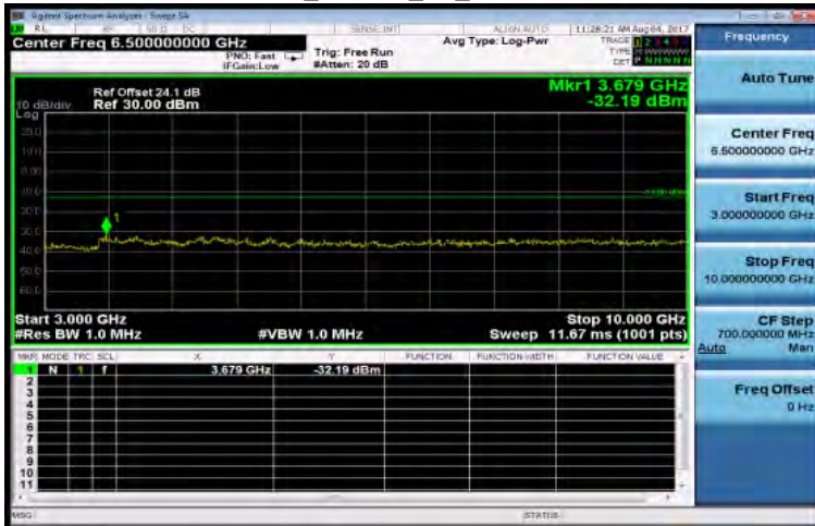
3GHz~10GHz_HSUPA_B5_LowCH4132-826.4
