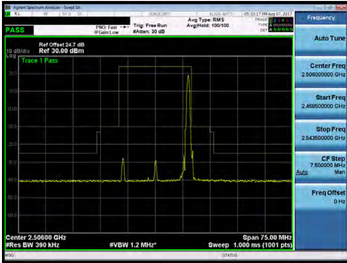
Band 41_20M_QPSK_LOW_RB100,0
