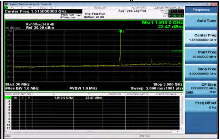
30MHz~3GHz_HSDPA_B2_HighCH9538-1907.6
