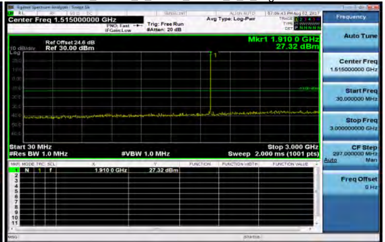
30MHz~3GHz_Band2_1_4MHz_QPSK_1_0_HighCH19193-1909.3
