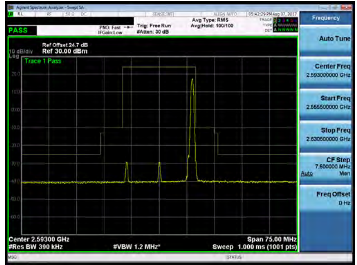
Band 41_20M_64QAM_MID_RB100,0
