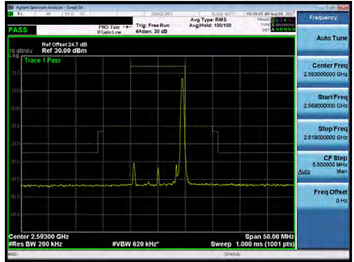
Band 41_10M_QPSK_MID_RB50,0
