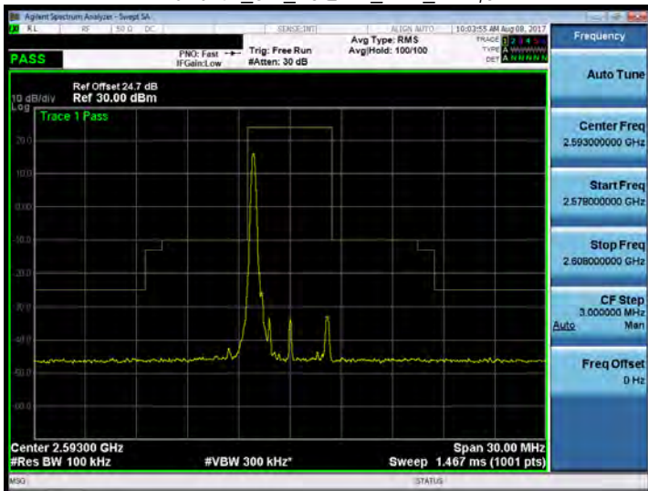
Band 41_5M_16QAM_MID_RB1,0
