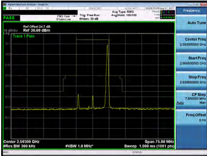
Band 41_15M_QPSK_MID_RB75,0
