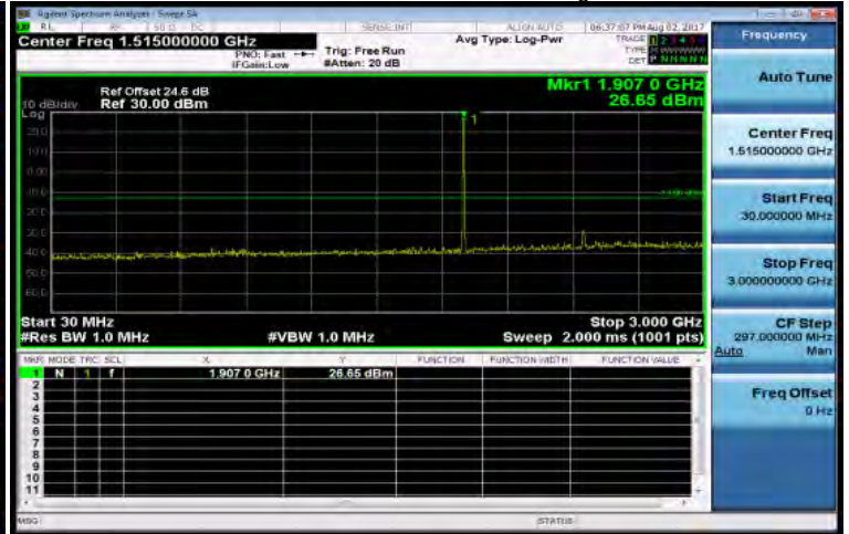
30MHz~3GHz_Band2_5MHz_QPSK_1_0_HighCH19175-1907.5
