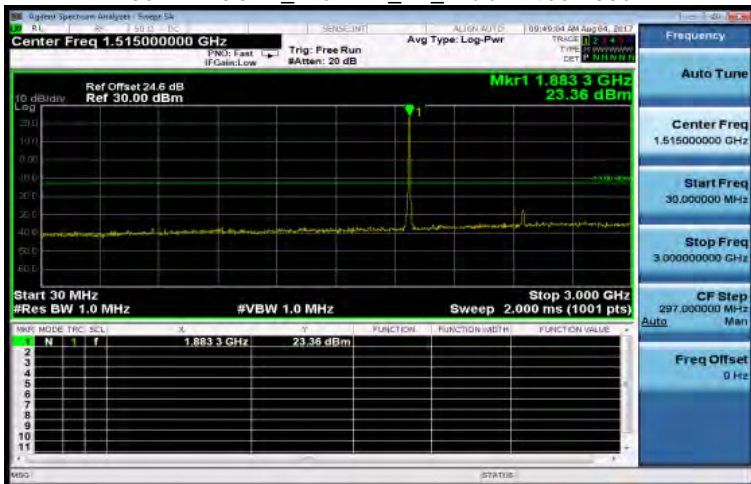
30MHz~3GHz_WCDMA_B2_MidCH9400-1880
