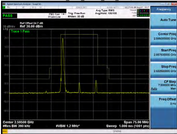
Band 38_20M_QPSK_MID_RB1,0
