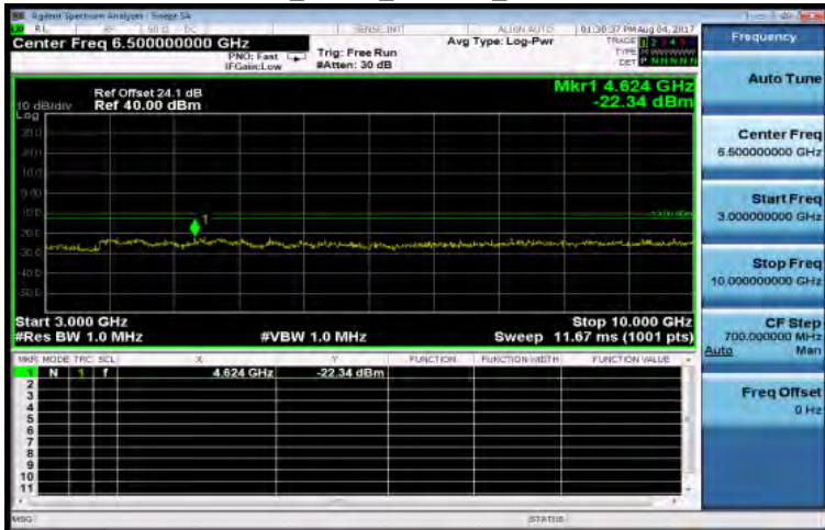
3GHz~10GHz_EDGE_850MHz_LowCH128-824.2
