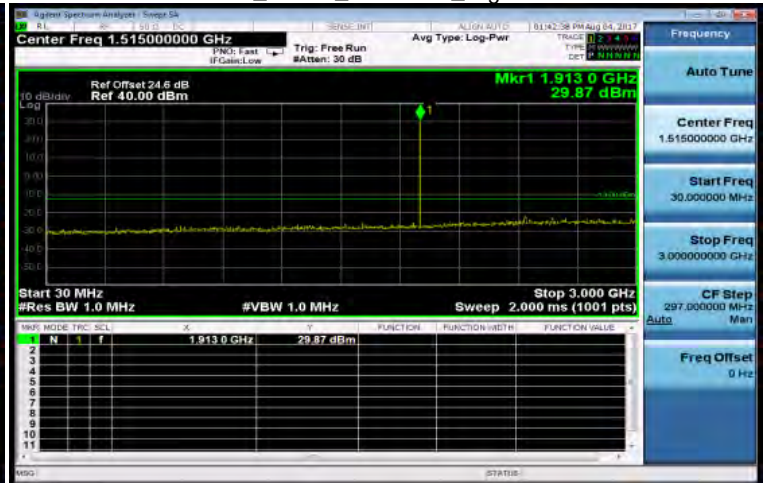
30MHz~3GHz_GPRS_1900MHz_HighCH810-1909.8
