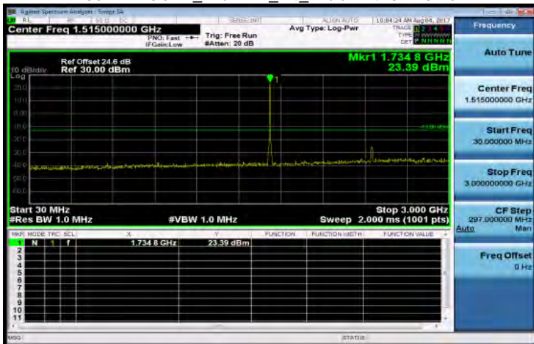
30MHz~3GHz_WCDMA_B4_MidCH1413-1732.6
