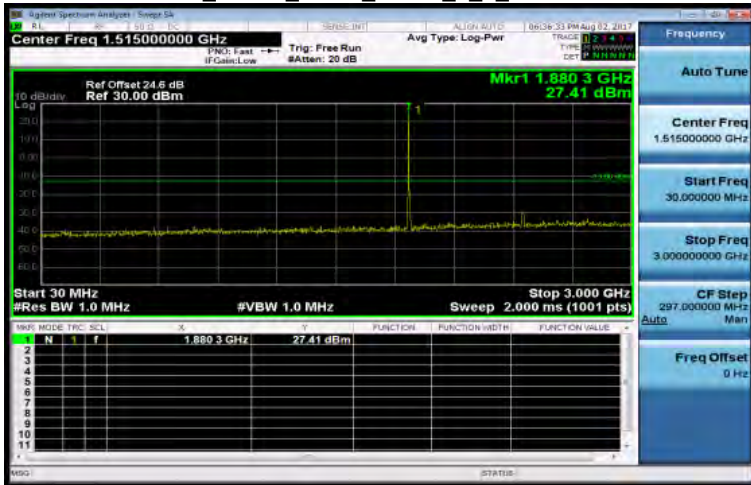
30MHz~3GHz_Band2_5MHz_QPSK_1_0_MidCH18900-1880
