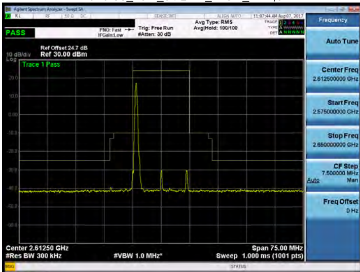
Band 38_15M_64QAM_HIGH_RB1,0
