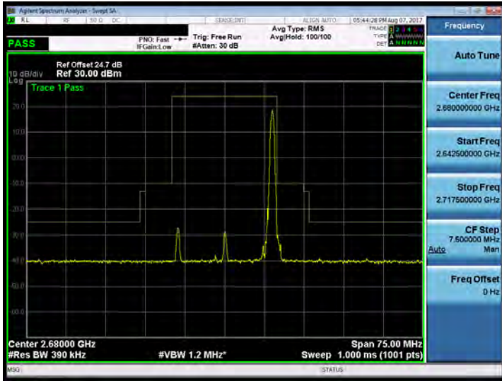
Band 41_20M_QPSK_HIGH_RB100,0
