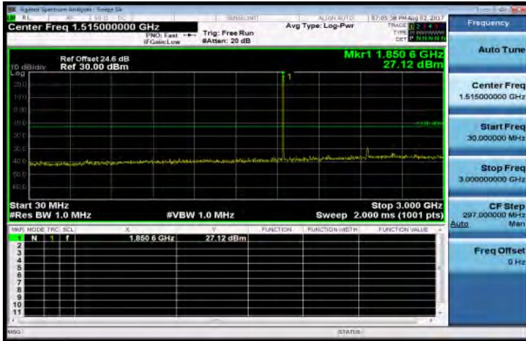
30MHz~3GHz_Band2_1_4MHz_QPSK_1_0_LowCH18607-1850.7
