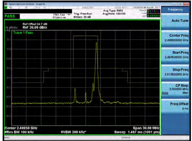
Band 41_5M_QPSK_LOW_RB25,0
