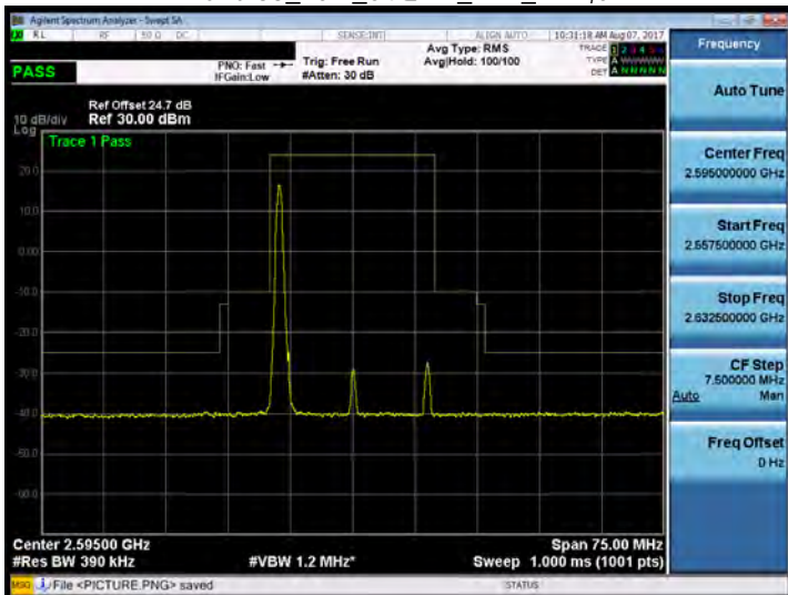
Band 38_20M_64QAM_MID_RB1,0
