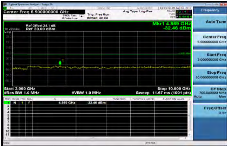
3GHz~10GHz_WCDMA_B5_LowCH4132-826.4
