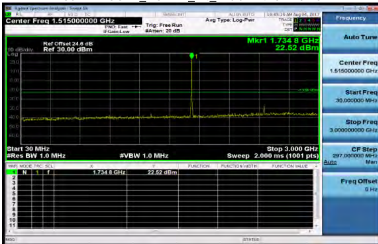
30MHz~3GHz_HSDPA_B4_MidCH1413-1732.6
