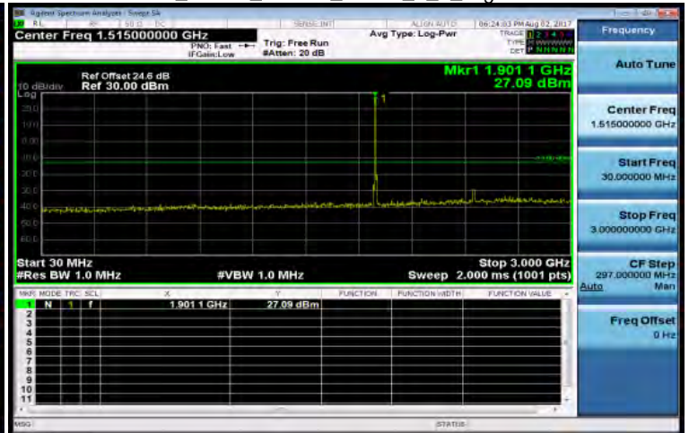
30MHz-3GHz_Band2_10MHz_QPSK_1_0_HighCH19150-1905
