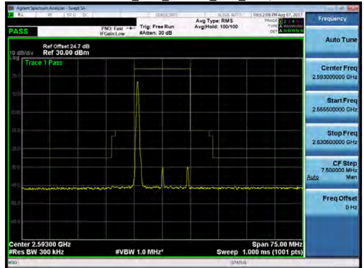
Band 41_15M_64QAM_MID_RB1,0
