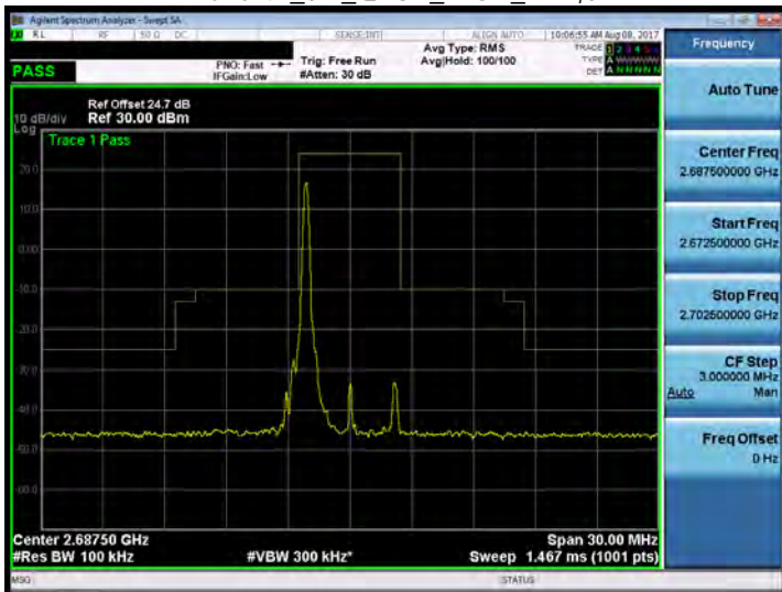
Band 41_5M_QPSK_HIGH_RB1,0
