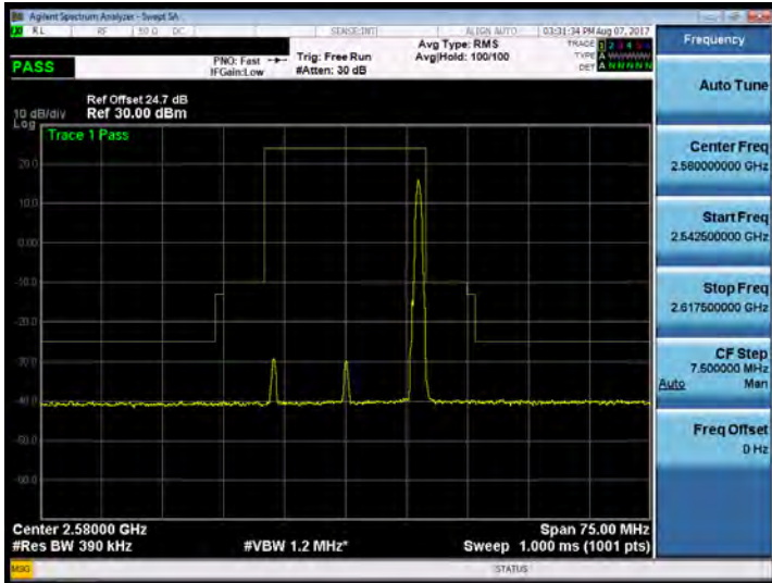
Band 38_20M_64QAM_LOW_RB100,0
