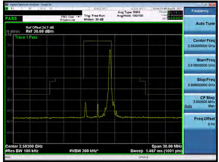
Band 41_5M_16QAM_MID_RB25,0
