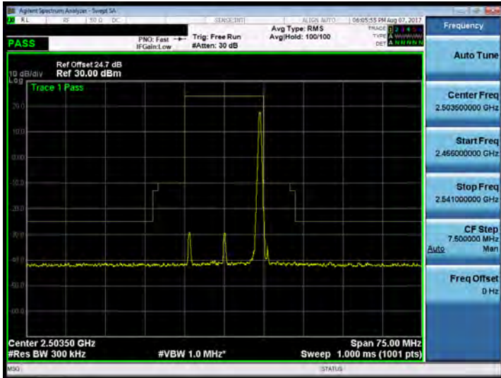
Band 41_15M_16QAM_LOW_RB75,0
