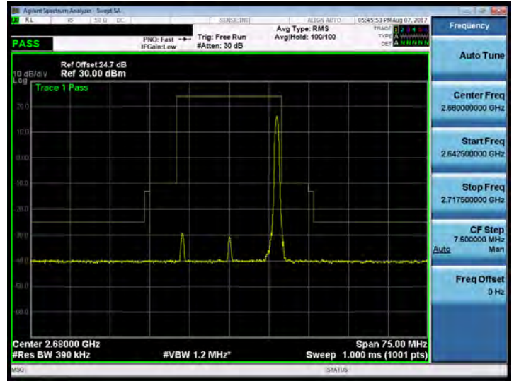
Band 41_20M_16QAM_HIGH_RB100,0
