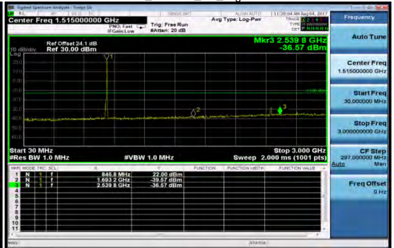
30MHz~3GHz_HSUPA_B5_HighCH4233-846.6
