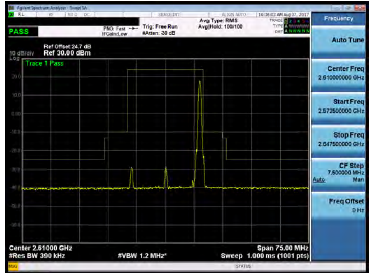
Band 38_20M_16QAM_HIGH_RB100,0
