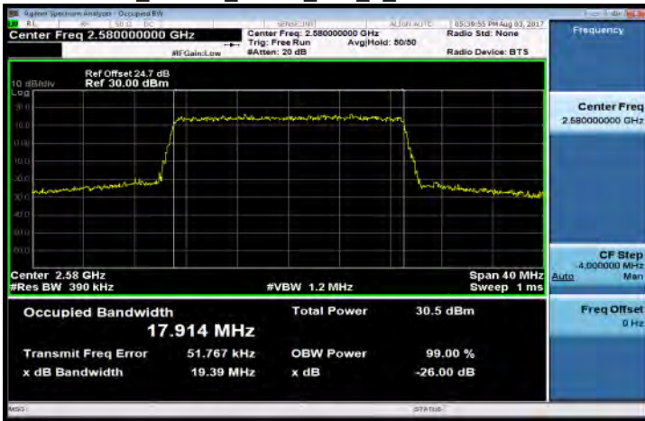
Band38_20MHz_QPSK_100_0_LowCH37850-2580
