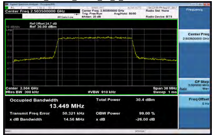
Band41_15MHz_QPSK_75_0_Low CH39725-2503.5
