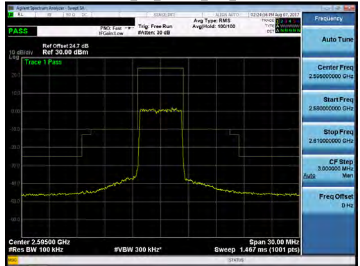
Band 38_5M_16QAM_HIGH_RB1,0
