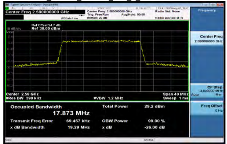
Band38_20MHz_16QAM_100_0_LowCH37850-2580
