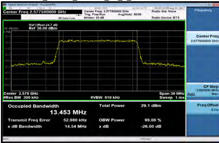
Band38_15MHz_16QAM_75_0_LowCH37825-2577.5
