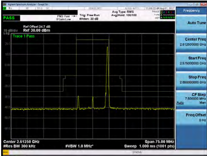
Band 38_15M_16QAM_HIGH_RB75,0
