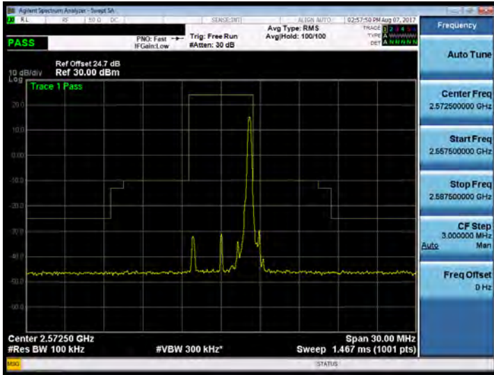
Band 38_5M_16QAM_LOW_RB25,0
