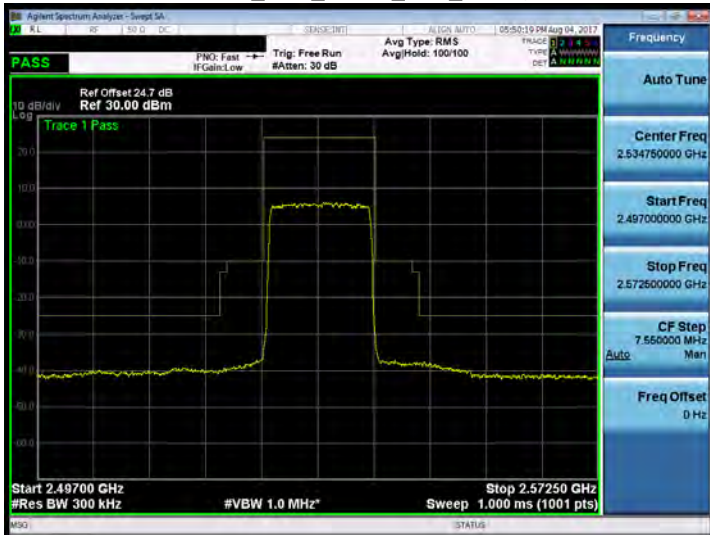
Band 7_15M_QPSK_HIGH_RB1,0
