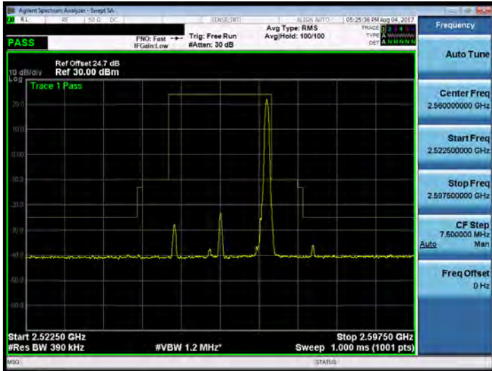
Band 7_20M_QPSK_HIGH_RB100,0
