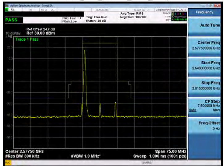
Band 38_15M_16QAM_LOW_RB1,0
