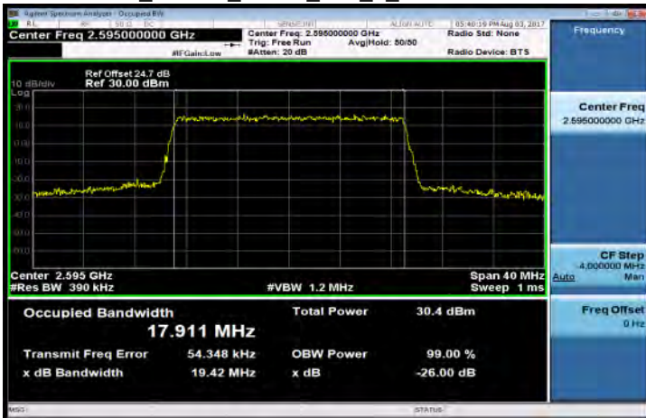
Band38_20MHz_QPSK_100_0_MidCH38000-2595
