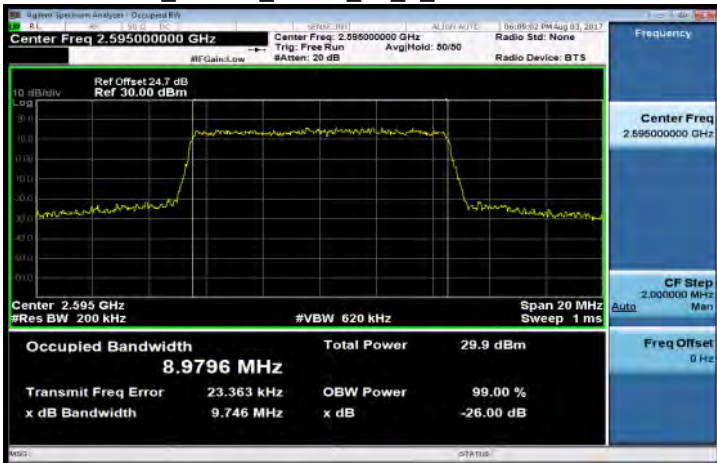
Band38_10MHz_QPSK_50_0_MidCH38000-2595
