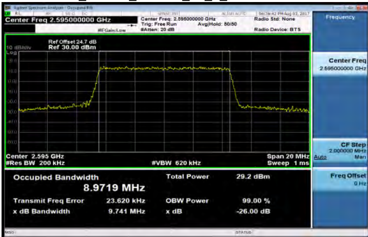
Band38_10MHz_64QAM_50_0_MidCH38000-2595
