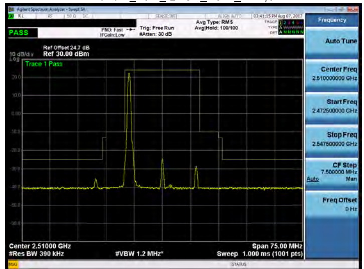
Band 7_20M_QPSK_LOW_RB1,0
