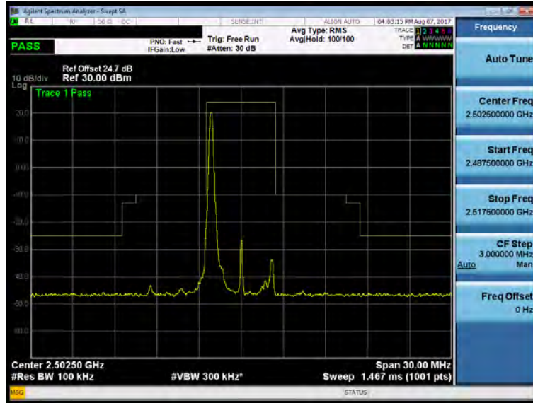
Band 7_5M_QPSK_LOW_RB1,0
