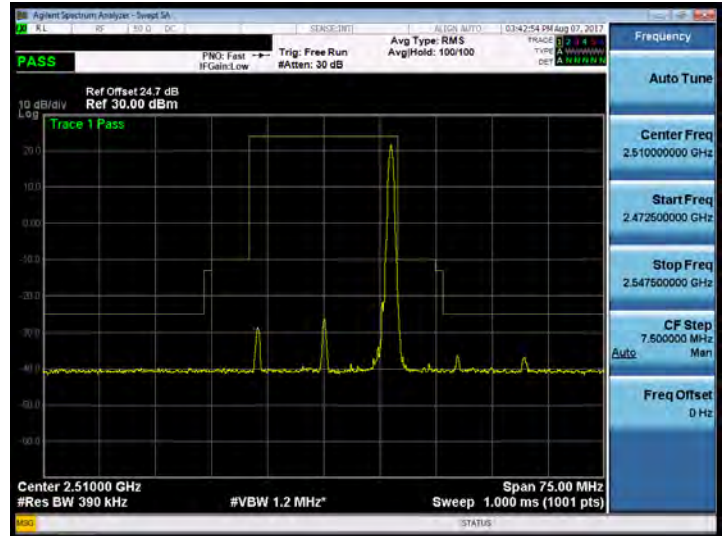
Band 7_20M_16QAM_LOW_RB100,0
