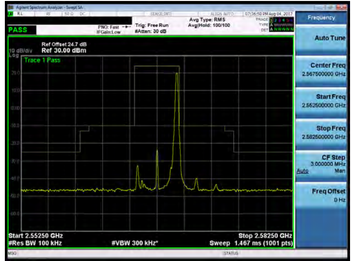
Band 7_5M_QPSK_HIGH_RB25,0
