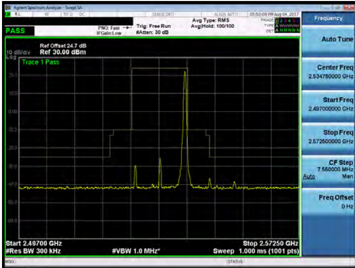
Band 7_15M_QPSK_MID_RB75,0
