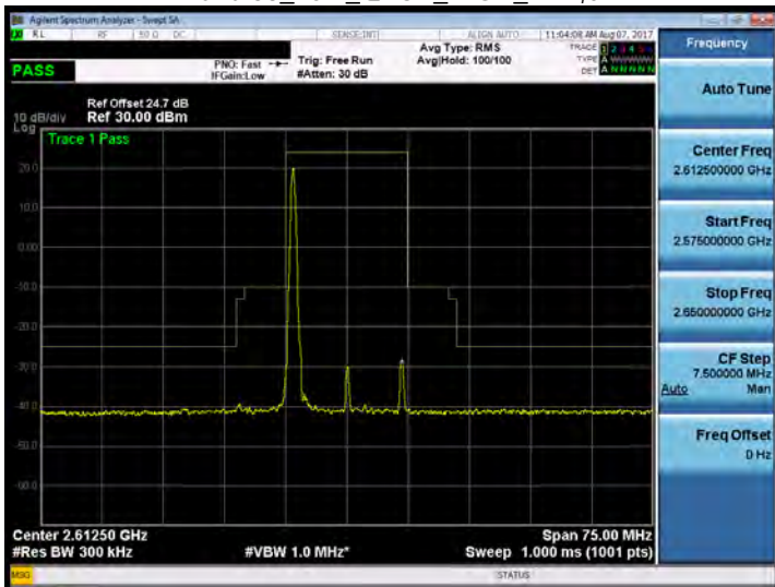
Band 38_15M_QPSK_HIGH_RB1,0
