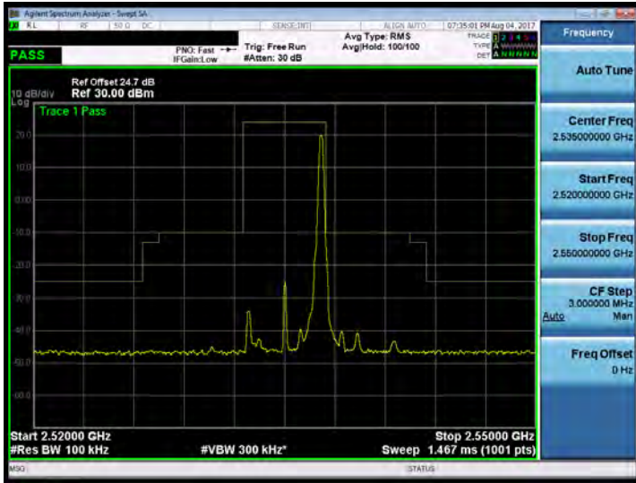
Band 7_5M_QPSK_MID_RB25,0
