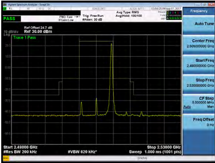
Band 7_10M_QPSK_LOW_RB50,0
