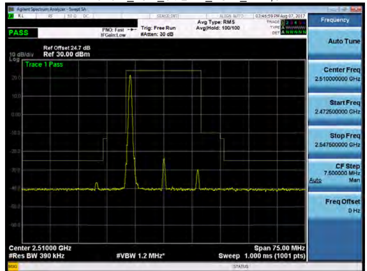
Band 7_20M_64QAM_LOW_RB1,0
