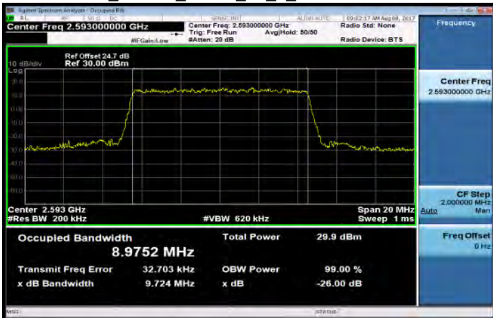
Band41_10MHz_QPSK_50_0_Mid CH40620-2593
