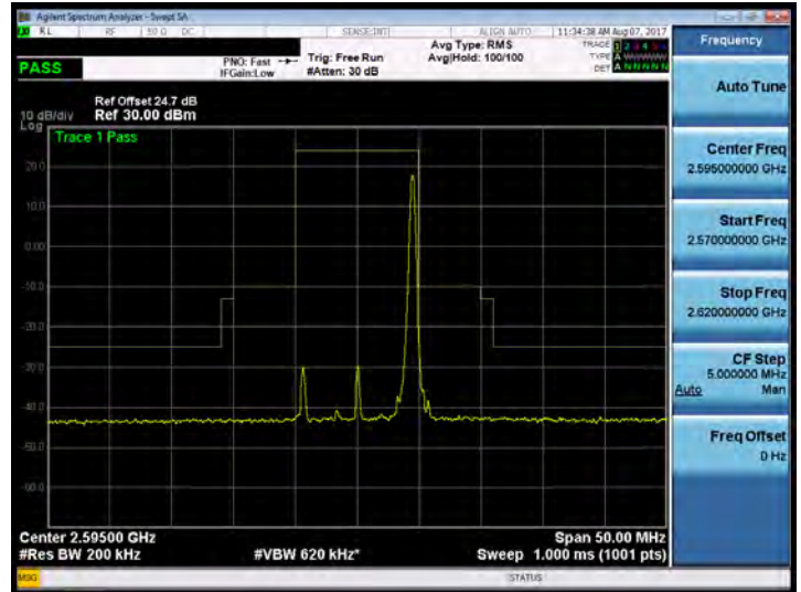
Band 38_10M_QPSK_MID_RB50,0
