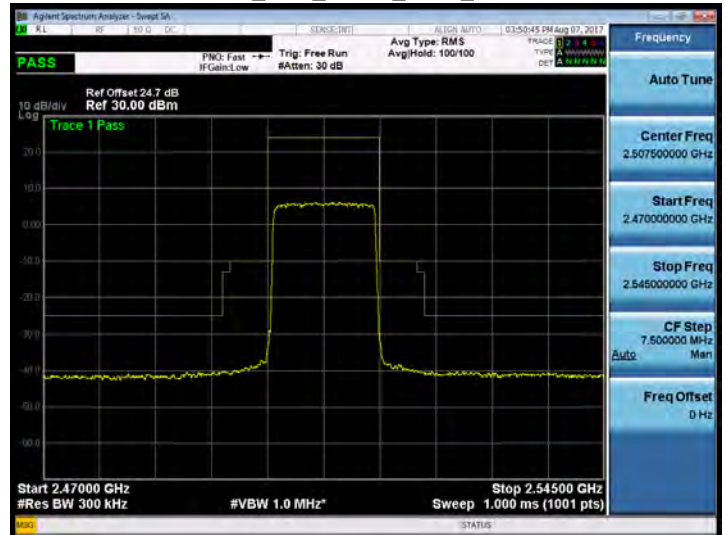
Band 7_15M_QPSK_MID_RB1,0
