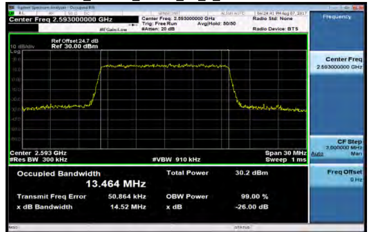
Band41_15MHz_QPSK_75_0_Mid CH40620-2593
