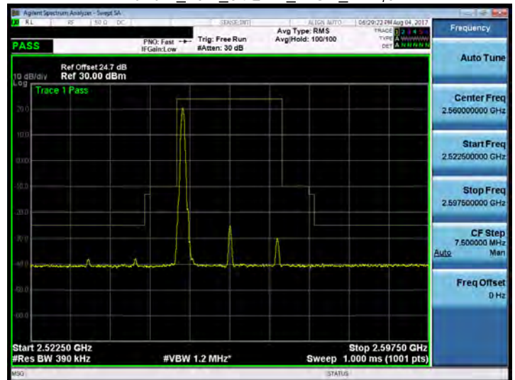
Band 7_20M_64QAM_HIGH_RB1,0
