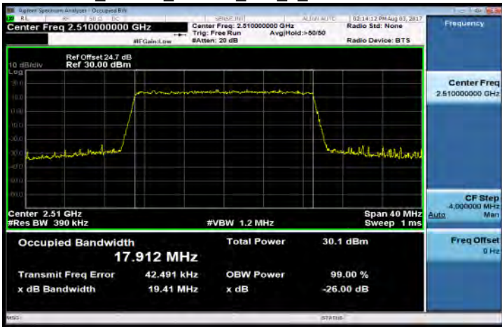
Band7_20MHz_64QAM_100_0_LowCH20850-2510
