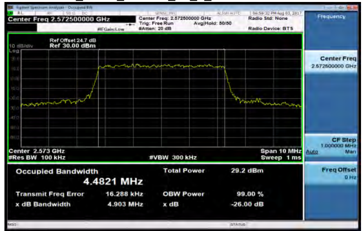
Band38_5MHz_64QAM_25_0_LowCH37775-2572.5
