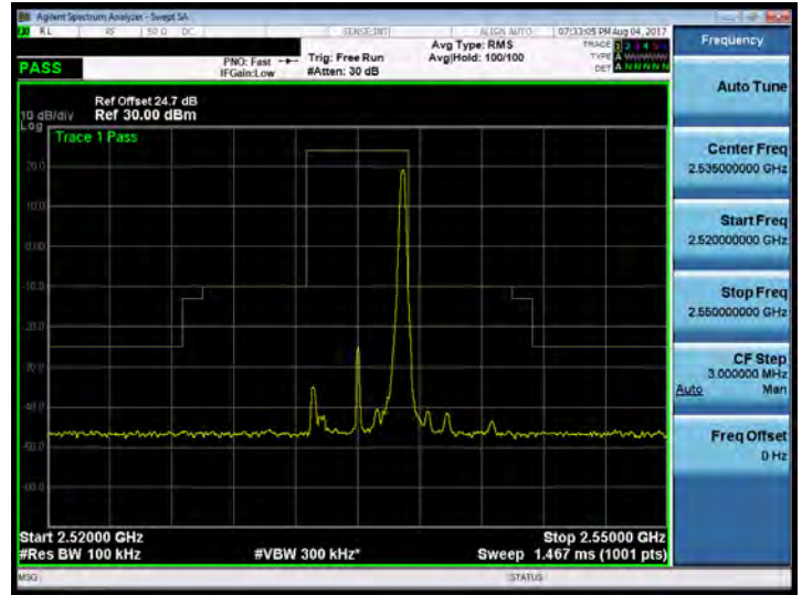
Band 7_5M_16QAM_MID_RB25,0
