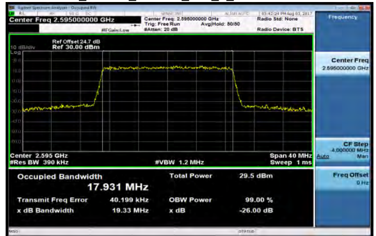
Band38_20MHz_16QAM_100_0_MidCH38000-2595
