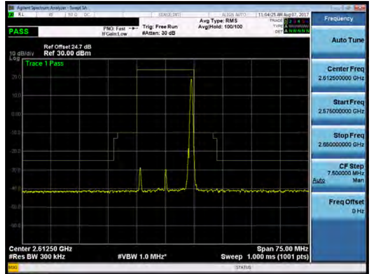
Band 38_15M_QPSK_HIGH_RB75,0
