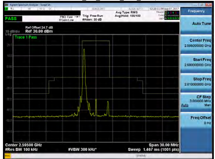
Band 38_5M_QPSK_MID_RB1,0
