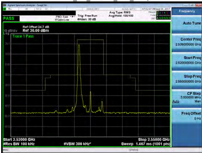
Band 7_5M_16QAM_MID_RB1,0
