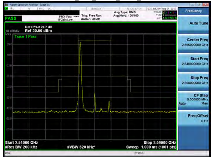
Band 7_10M_QPSK_HIGH_RB1,0
