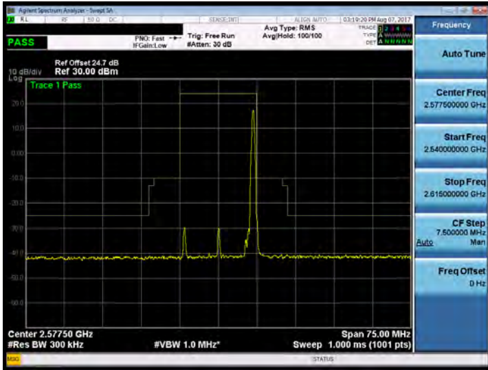
Band 38_15M_16QAM_LOW_RB75,0
