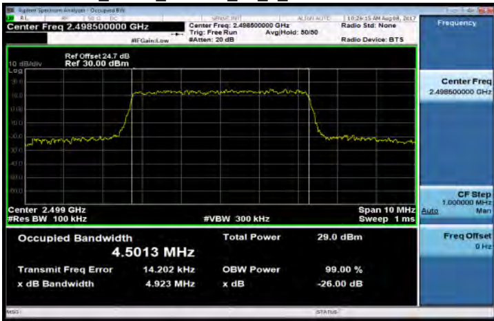
Band41_5MHz_16QAM_25_0_Low CH39675-2498.5
