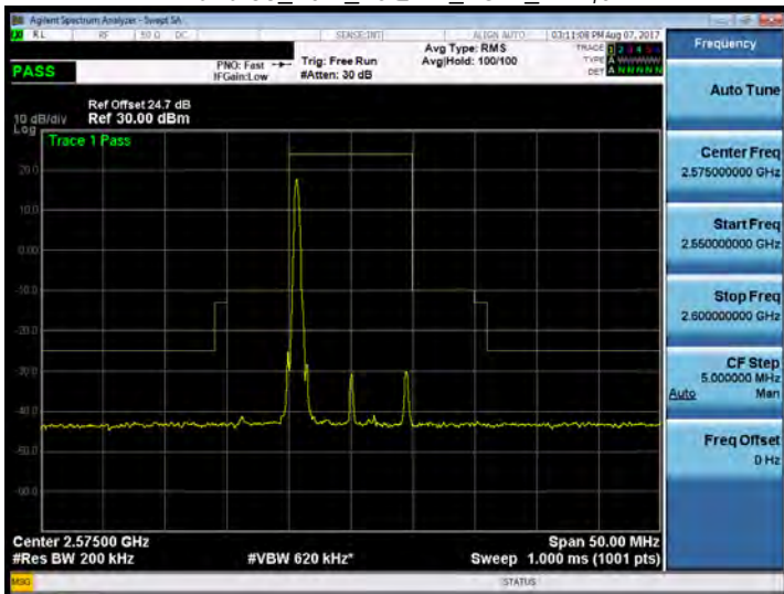
Band 38_10M_16QAM_LOW_RB1,0
