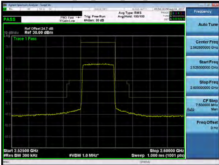
Band 7_15M_64QAM_LOW_RB1,0
