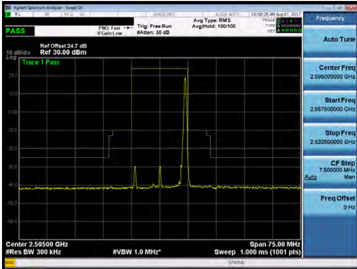
Band 38_15M_QPSK_MID_RB75,0
