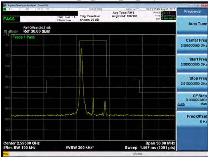
Band 38_5M_16QAM_MID_RB1,0
