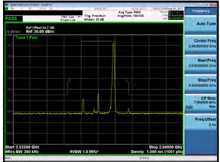
Band 7_15M_QPSK_HIGH_RB75,0
