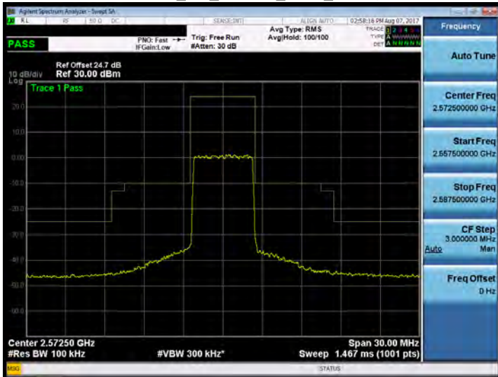
Band 38_5M_16QAM_MID_RB1,0
