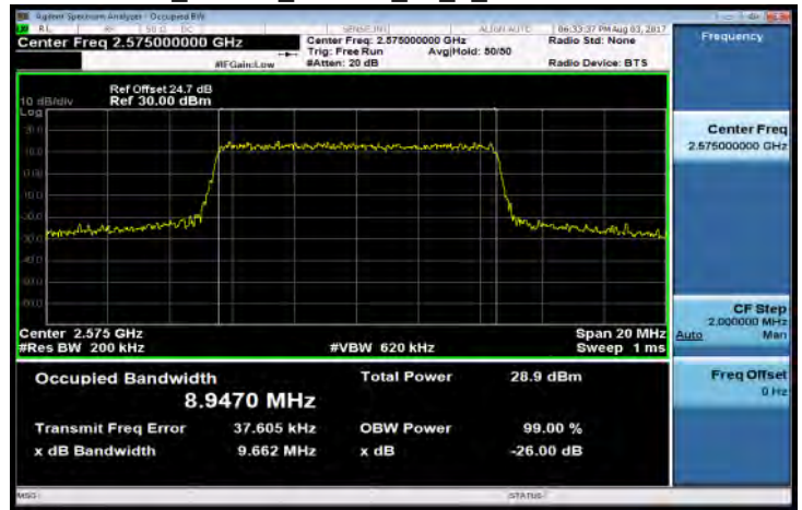
Band38_10MHz_16QAM_50_0_LowCH37800-2575
