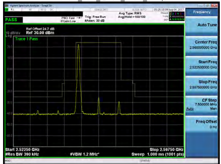
Band 7_20M_QPSK_HIGH_RB1,0
