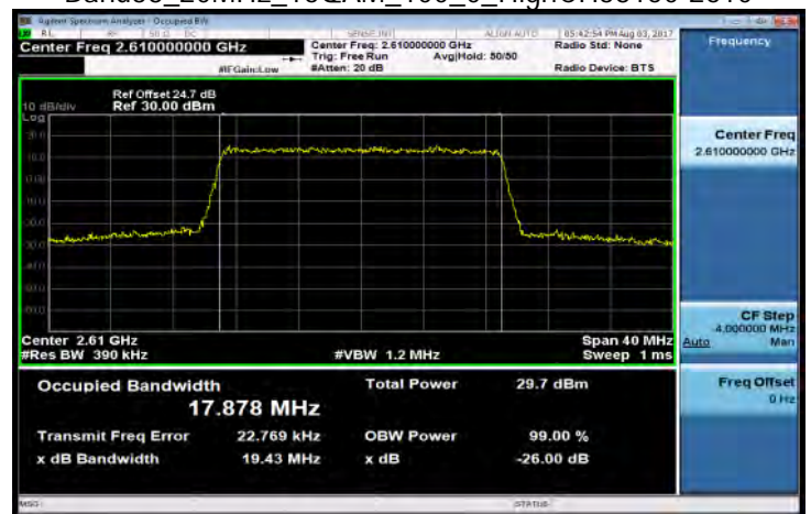
Band38_20MHz_16QAM_100_0_HighCH38150-2610
