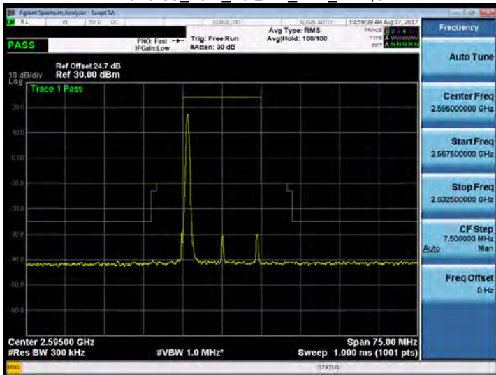
Band 38_15M_16QAM_MID_RB1,0
