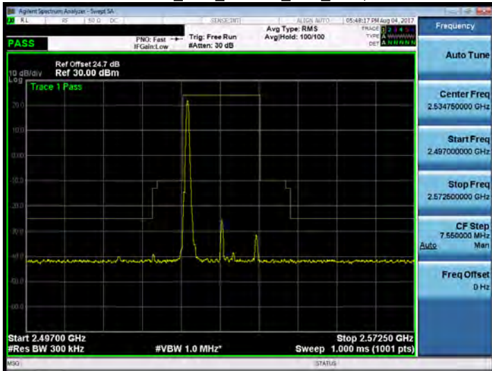
Band 7_15M_16QAM_MID_RB1,0
