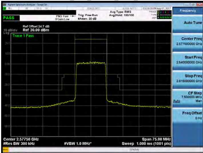
Band 38_15M_16QAM_MID_RB1,0
