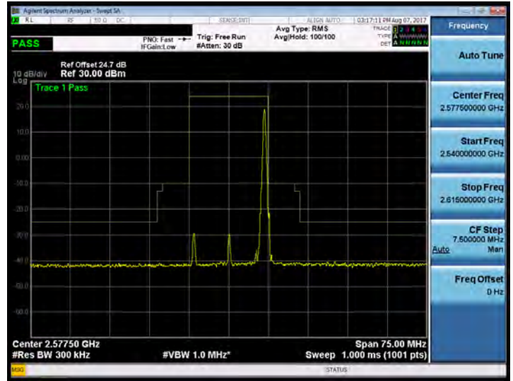
Band 38_15M_QPSK_LOW_RB75,0
