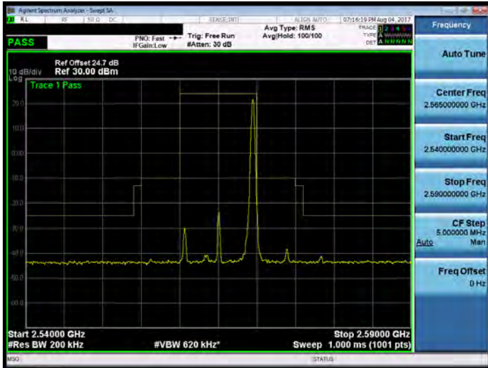
Band 7_10M_QPSK_HIGH_RB50,0
