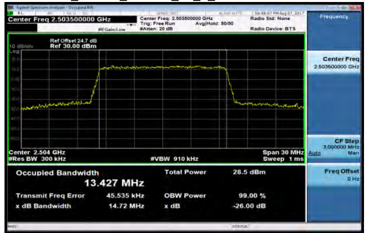
Band41_15MHz_64QAM_75_0_Low CH39725-2503.5
