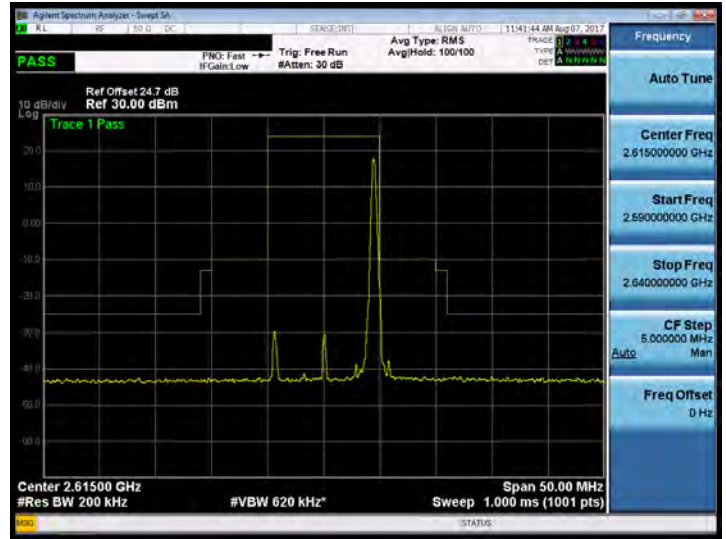
Band 38_10M_16QAM_HIGH_RB50,0
