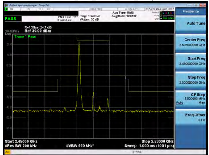
Band 7_10M_QPSK_LOW_RB1,0
