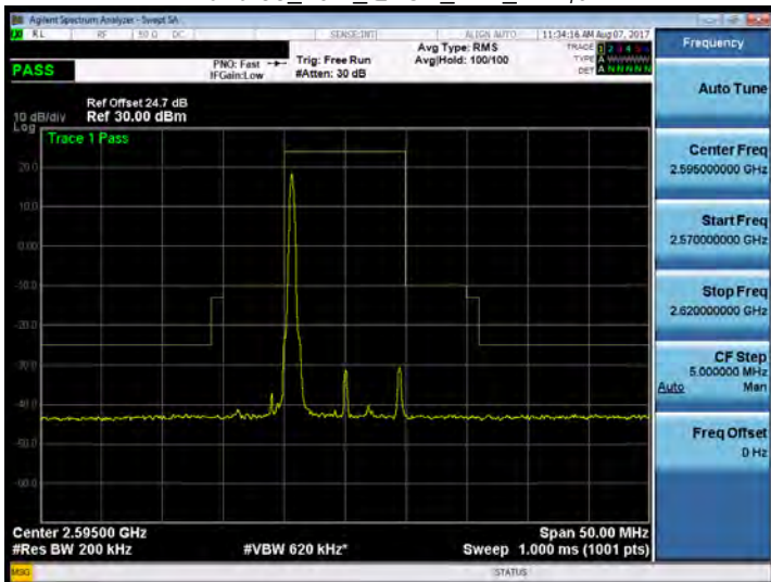
Band 38_10M_QPSK_MID_RB1,0
