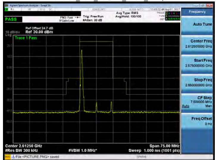
Band 38_15M_16QAM_HIGH_RB1,0
