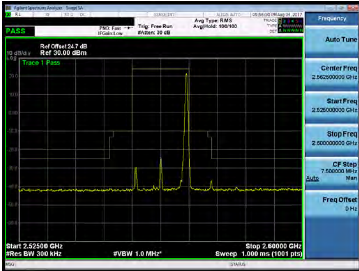
Band 7_15M_16QAM_HIGH_RB75,0
