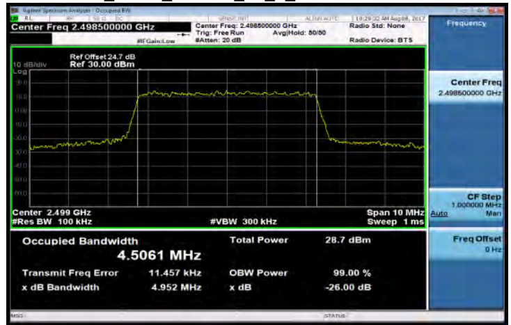
Band41_5MHz_64QAM_25_0_Low CH39675-2498.5
