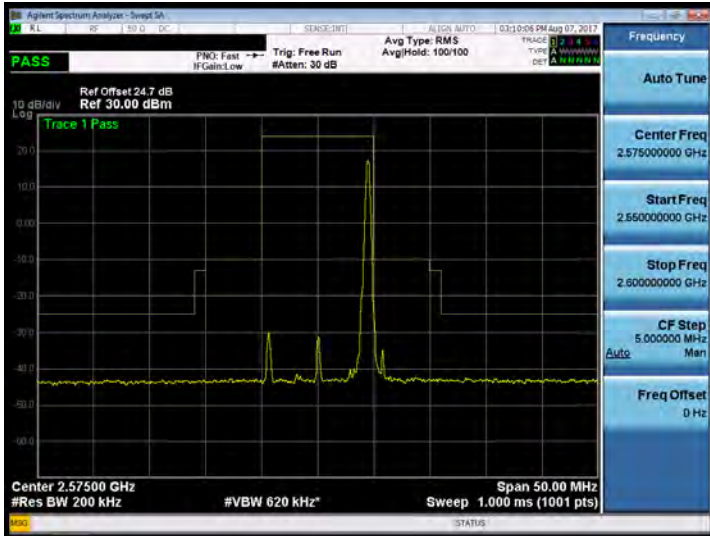
Band 38_10M_QPSK_LOW_RB50,0
