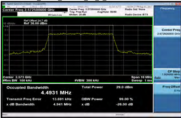
Band38_5MHz_16QAM_25_0_LowCH37775-2572.5
