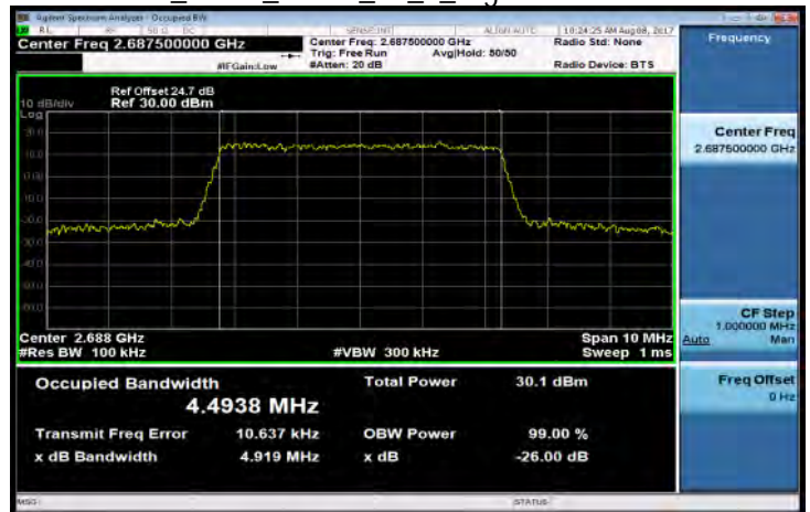
Band41_5MHz_QPSK_25_0_High CH41565-2687.5
