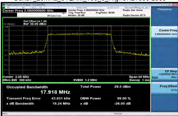
Band7_20MHz_64QAM_100_0_HighCH21350-2560
