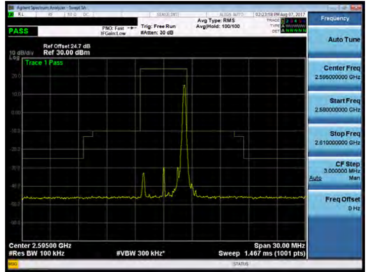
Band 38_5M_16QAM_MID_RB25,0
