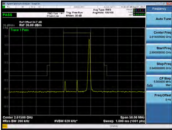
Band 38_10M_64QAM_HIGH_RB50,0
