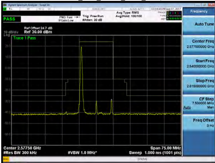
Band 38_15M_QPSK_LOW_RB1,0
