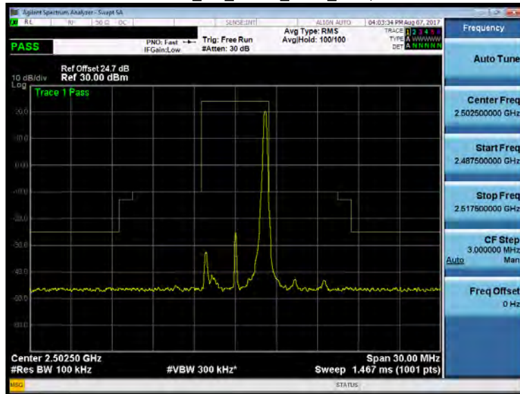
Band 7_5M_QPSK_LOW_RB1,24
