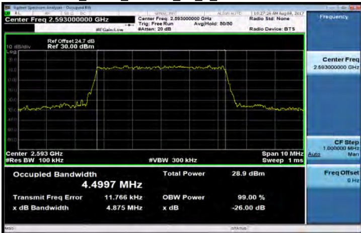
Band41_5MHz_16QAM_25_0_Mid CH40620-2593
