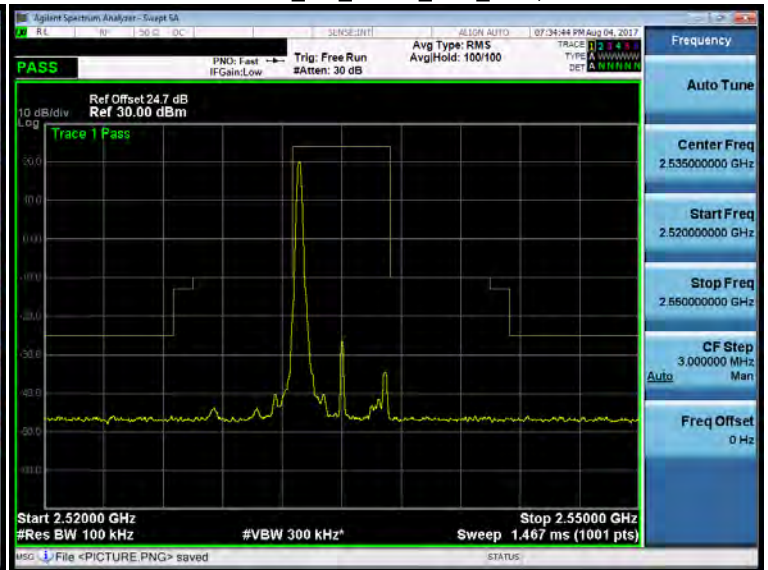
Band 7_5M_QPSK_MID_RB1,0
