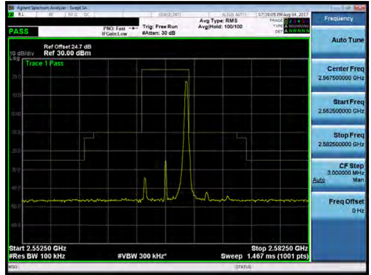
Band 7_5M_64QAM_HIGH_RB25,0
