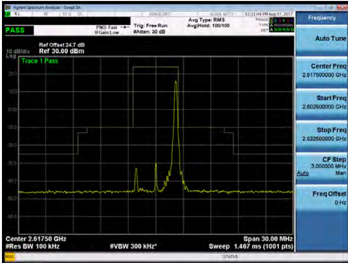
Band 38_5M_16QAM_HIGH_RB25,0
