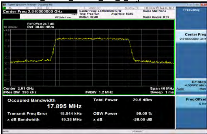
Band38_20MHz_64QAM_100_0_HighCH38150-2610
