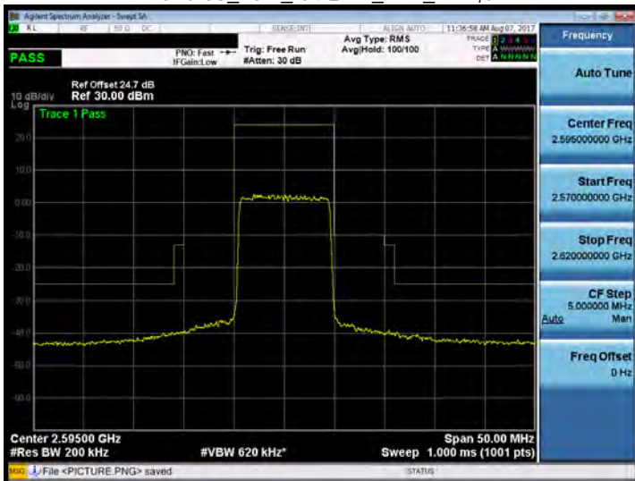
Band 38_10M_64QAM_MID_RB1,0
