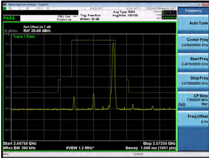
Band 7_20M_16QAM_MID_RB100,0
