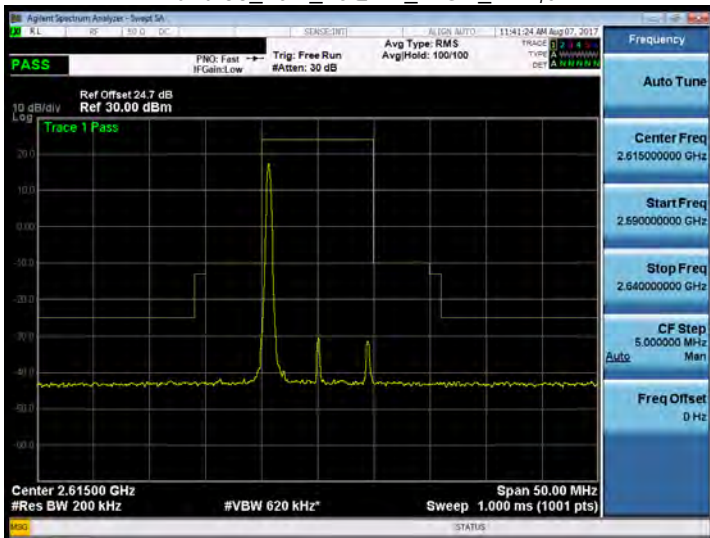
Band 38_10M_16QAM_HIGH_RB1,0
