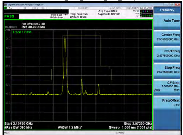
Band 7_20M_16QAM_MID_RB1,0
