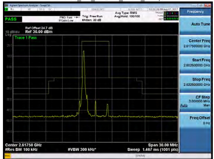
Band 38_5M_16QAM_HIGH_RB1,0
