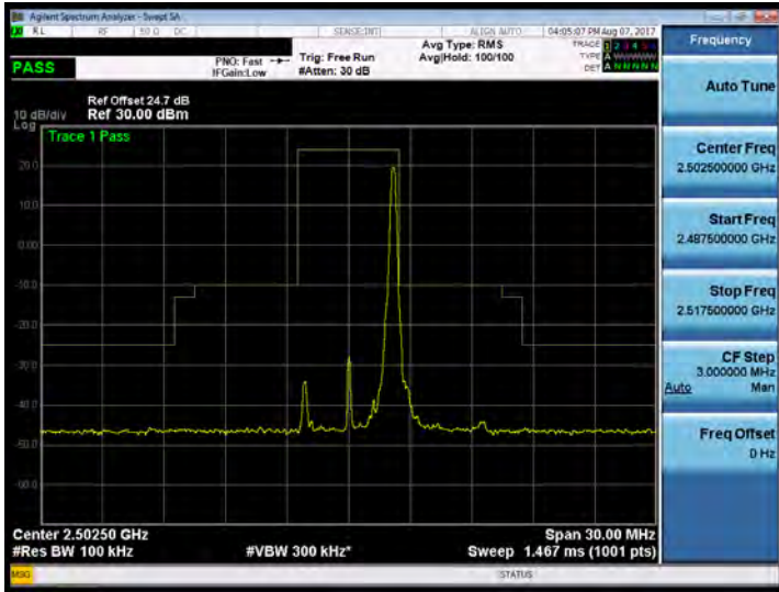
Band 7_5M_16QAM_LOW_RB25,0
