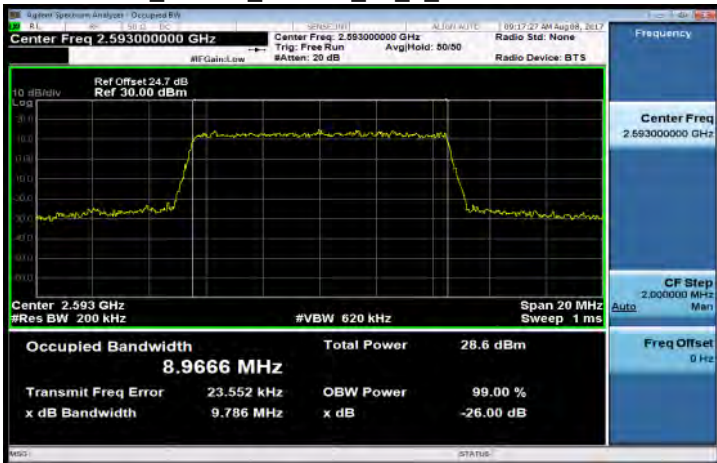
Band41_10MHz_64QAM_50_0_Mid CH40620-2593
