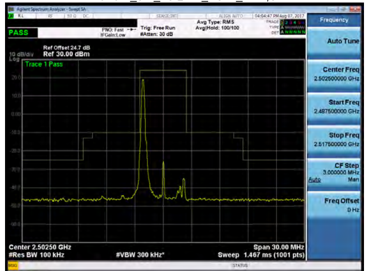
Band 7_5M_16QAM_LOW_RB1,0
