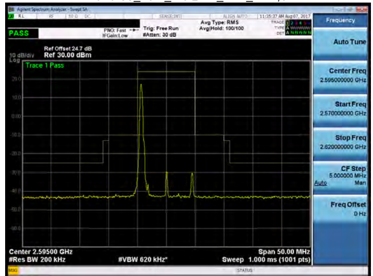
Band 38_10M_16QAM_MID_RB1,0
