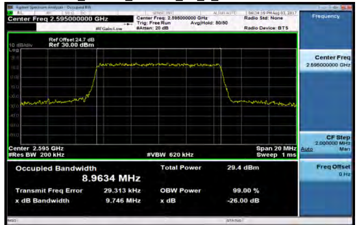
Band38_10MHz_16QAM_50_0_MidCH38000-2595
