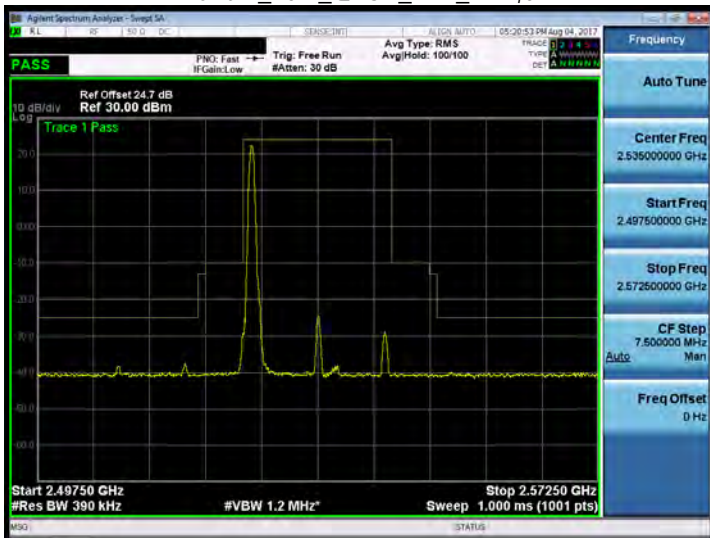
Band 7_20M_QPSK_MID_RB1,0
