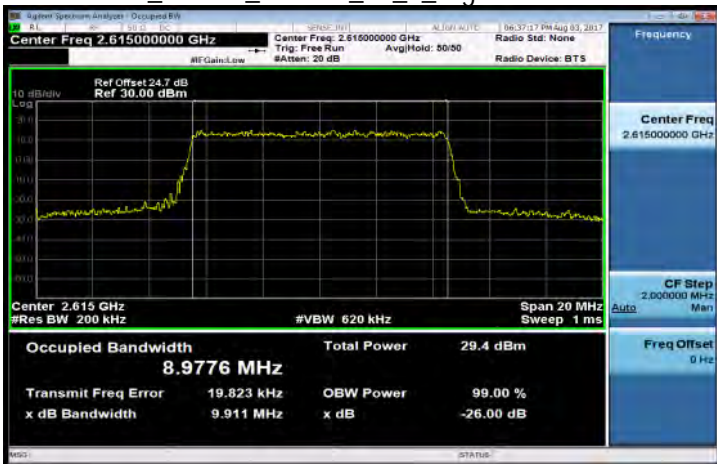
Band38_10MHz_64QAM_50_0_HighCH38200-2615
