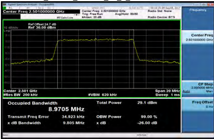
Band41_10MHz_64QAM_50_0_Low CH39700-2501
