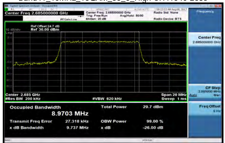
Band41_10MHz_16QAM_50_0_High CH41540-2685
