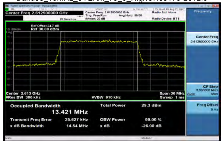
Band38_15MHz_64QAM_75_0_HighCH38175-2612.5
