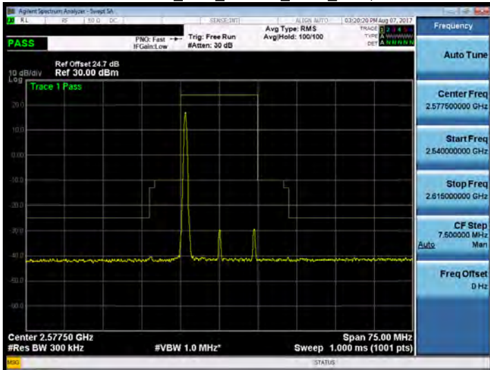
Band 38_15M_64QAM_LOW_RB1,0
