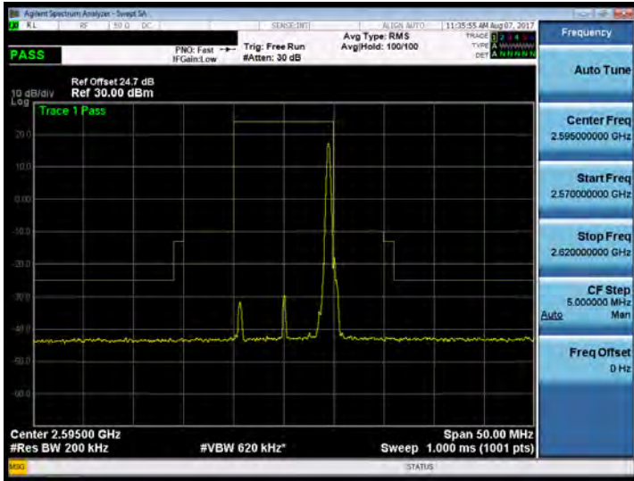
Band 38_10M_16QAM_MID_RB50,0
