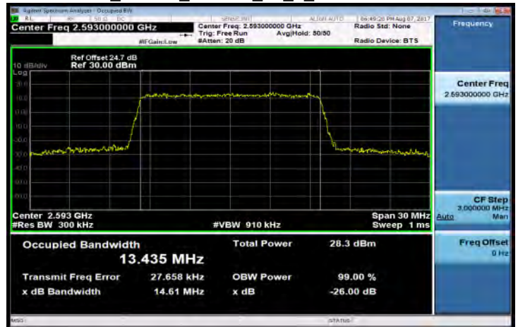
Band41_15MHz_64QAM_75_0_Mid CH40620-2593
