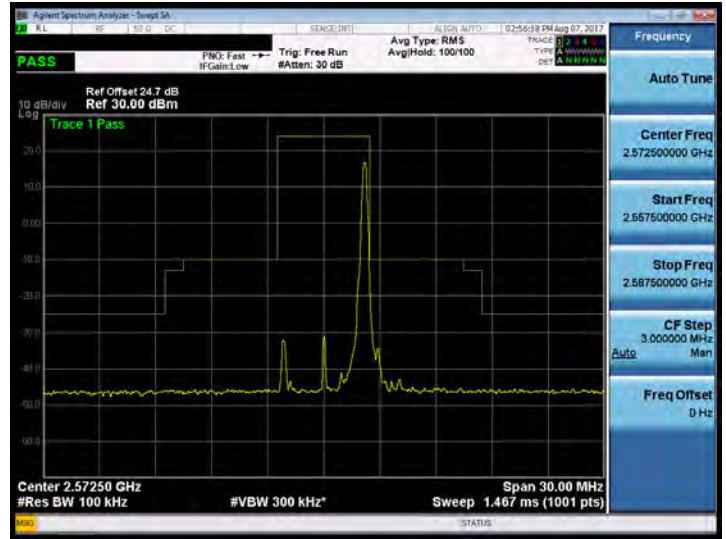
Band 38_5M_QPSK_LOW_RB25,0
