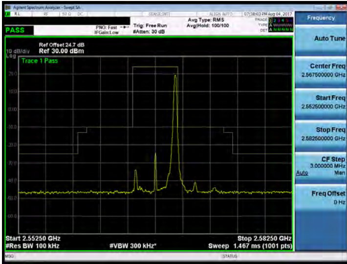
Band 7_5M_16QAM_HIGH_RB25,0
