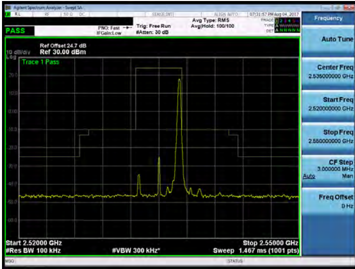
Band 7_5M_64QAM_MID_RB25,0
