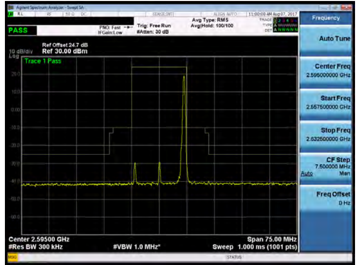
Band 38_15M_16QAM_MID_RB75,0
