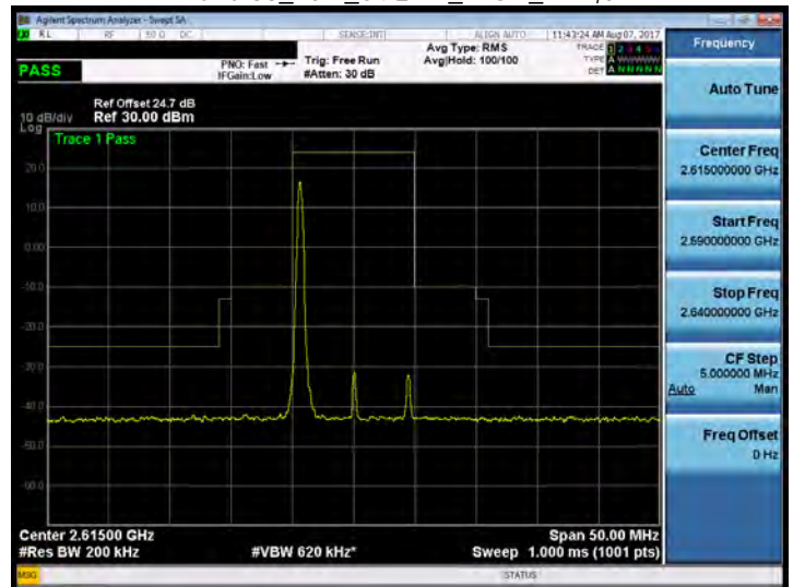
Band 38_10M_64QAM_HIGH_RB1,0
