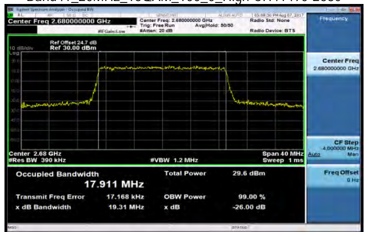
Band41_20MHz_16QAM_100_0_High CH41490-2680
