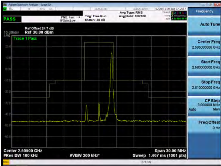
Band 38_5M_64QAM_MID_RB25,0
