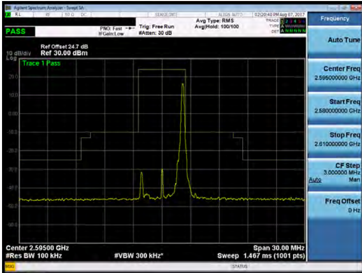
Band 38_5M_QPSK_MID_RB25,0
