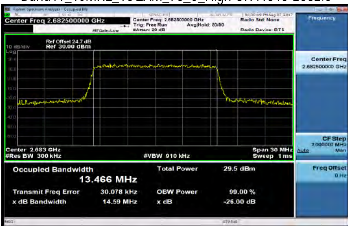
Band41_15MHz_16QAM_75_0_High CH41515-2682.5
