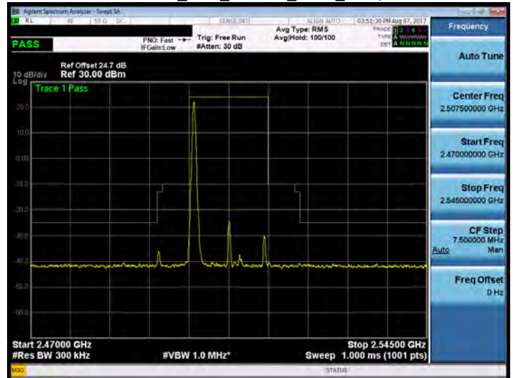
Band 7_15M_16QAM_LOW_RB1,0
