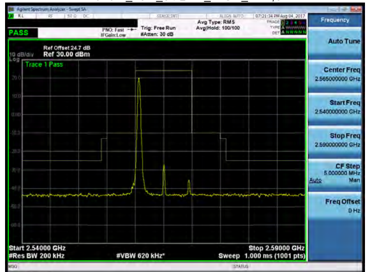
Band 7_10M_64QAM_HIGH_RB1,0
