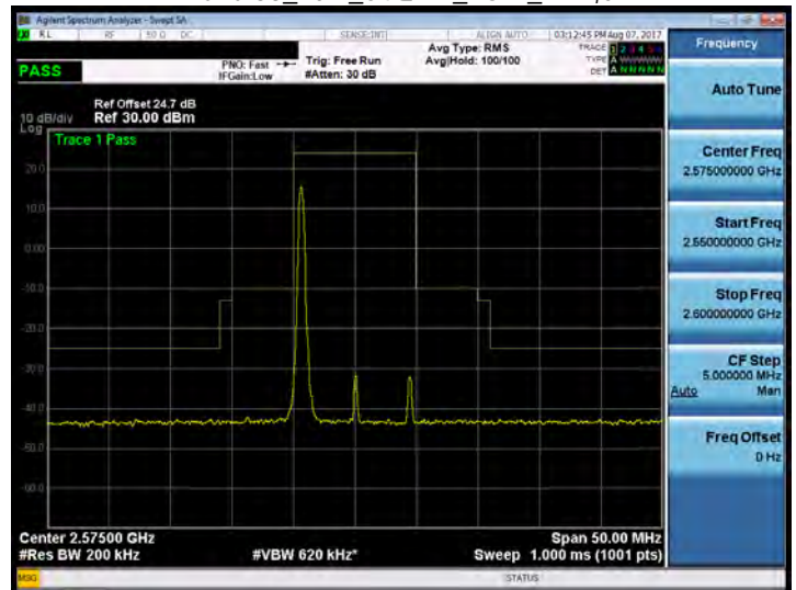
Band 38_10M_64QAM_LOW_RB1,0
