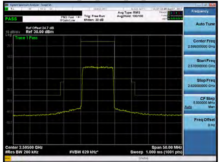
Band 38_10M_64QAM_HIGH_RB1,0
