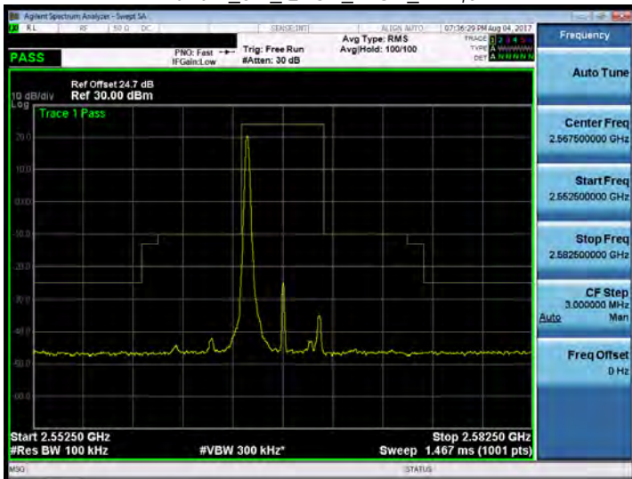
Band 7_5M_QPSK_HIGH_RB1,0
