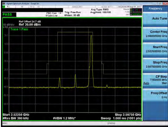
Band 7_20M_64QAM_HIGH_RB100,0
