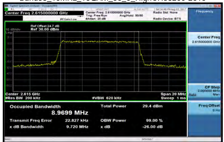
Band38_10MHz_16QAM_50_0_HighCH38200-2615
