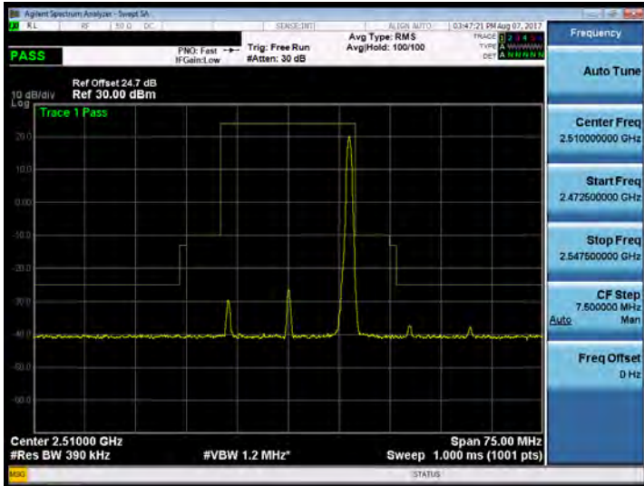
Band 7_20M_64QAM_LOW_RB100,0
