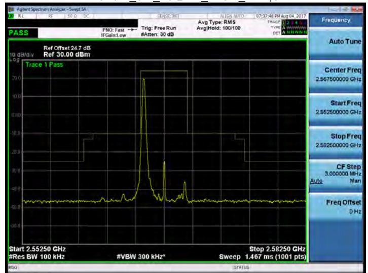
Band 7_5M_16QAM_HIGH_RB1,0
