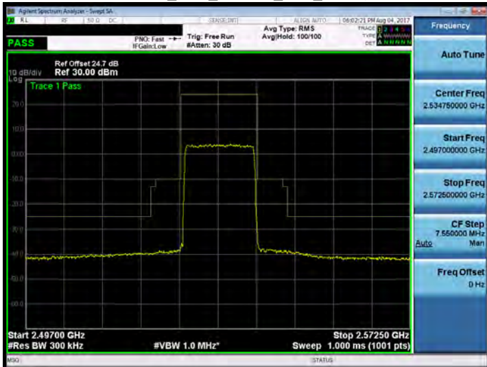
Band 7_15M_64QAM_HIGH_RB1,0
