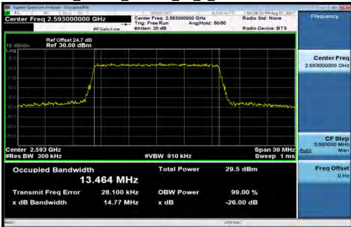
Band41_15MHz_16QAM_75_0_Mid CH40620-2593
