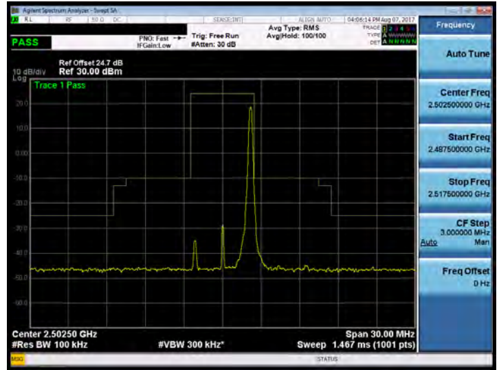
Band 7_5M_64QAM_LOW_RB25,0
