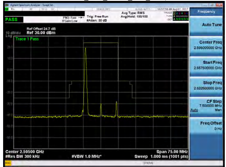
Band 38_15M_QPSK_MID_RB1,0
