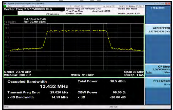
Band38_15MHz_QPSK_75_0_LowCH37825-2577.5
