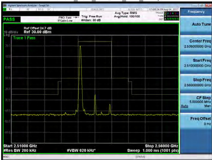
Band 7_10M_64QAM_MID_RB1,0
