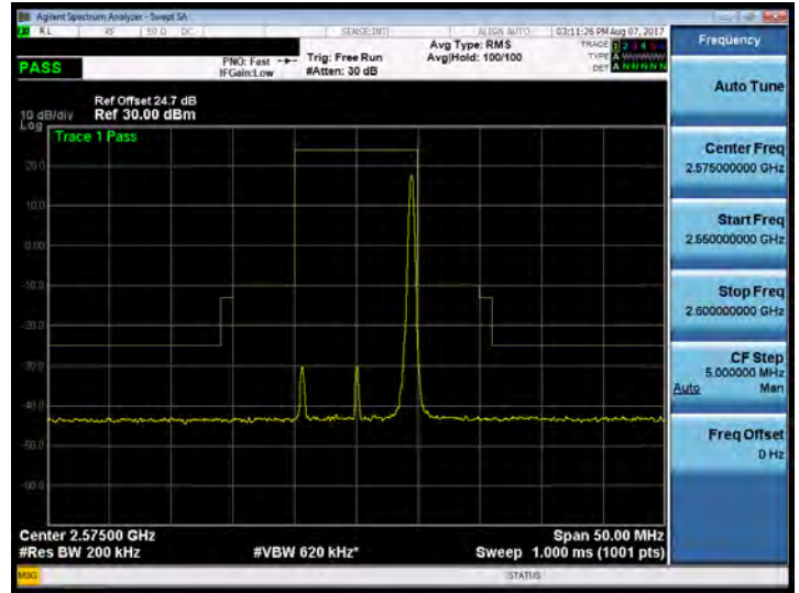
Band 38_10M_16QAM_LOW_RB50,0
