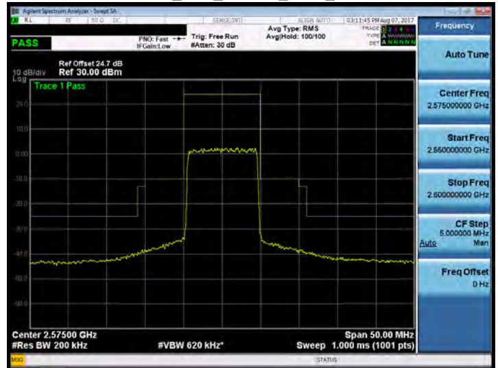
Band 38_10M_16QAM_MID_RB1,0
