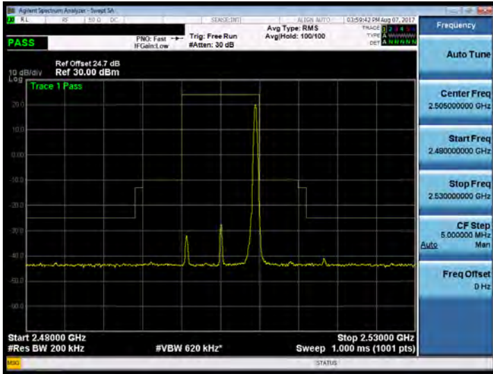
Band 7_10M_64QAM_LOW_RB50,0
