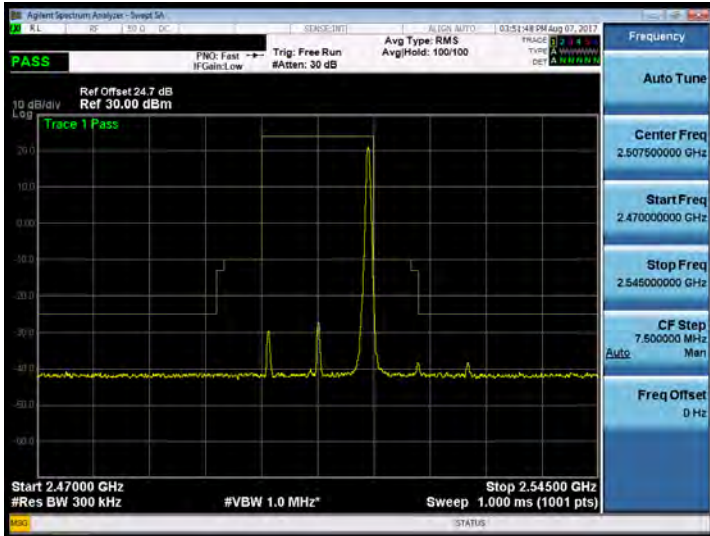
Band 7_15M_16QAM_LOW_RB75,0
