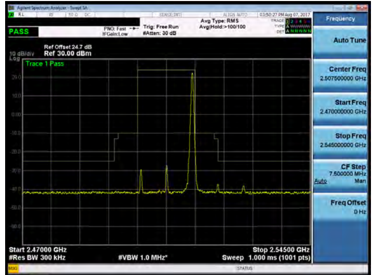
Band 7_15M_QPSK_LOW_RB75,0
