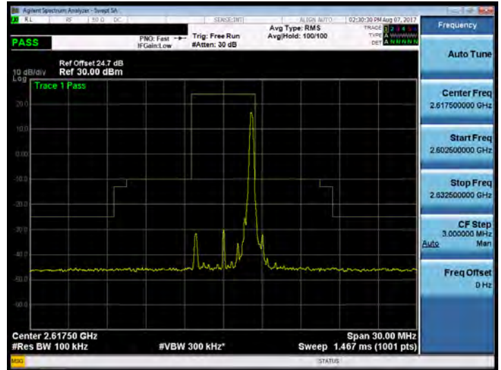
Band 38_5M_QPSK_HIGH_RB25,0
