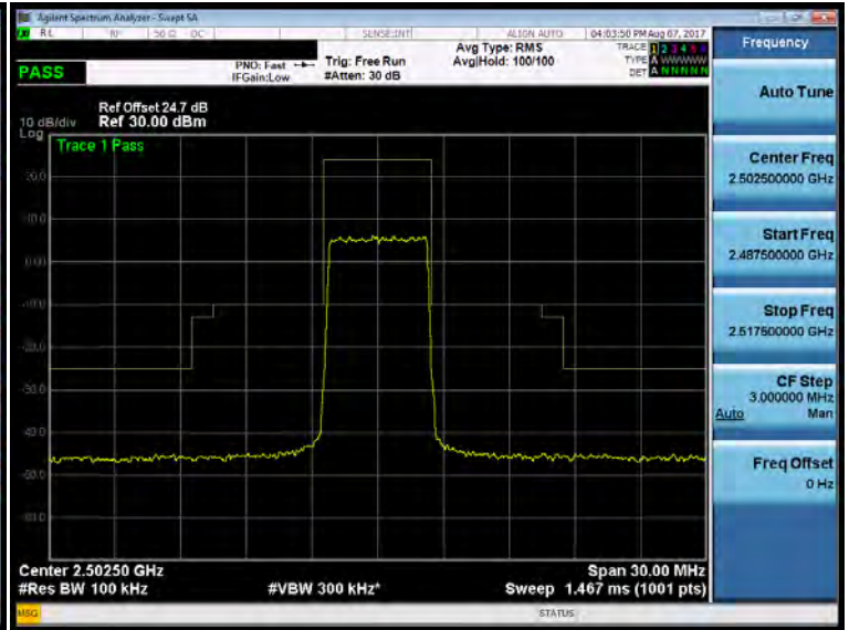
Band 7_5M_QPSK_LOW_RB25,0
