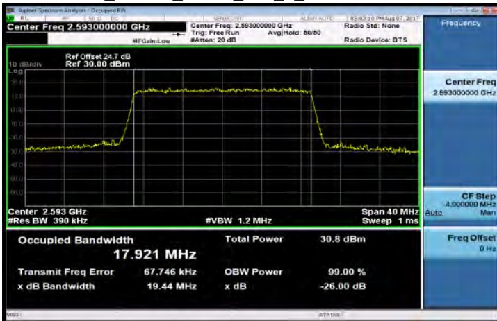
Band41_20MHz_QPSK_100_0_Mid CH40620-2593
