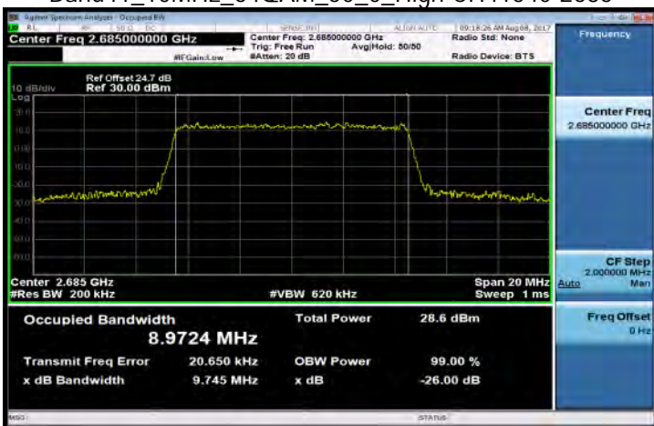
Band41_10MHz_64QAM_50_0_High CH41540-2685
