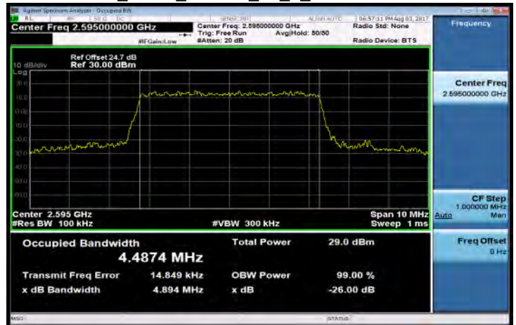
Band38_5MHz_64QAM_25_0_MidCH38000-2595
