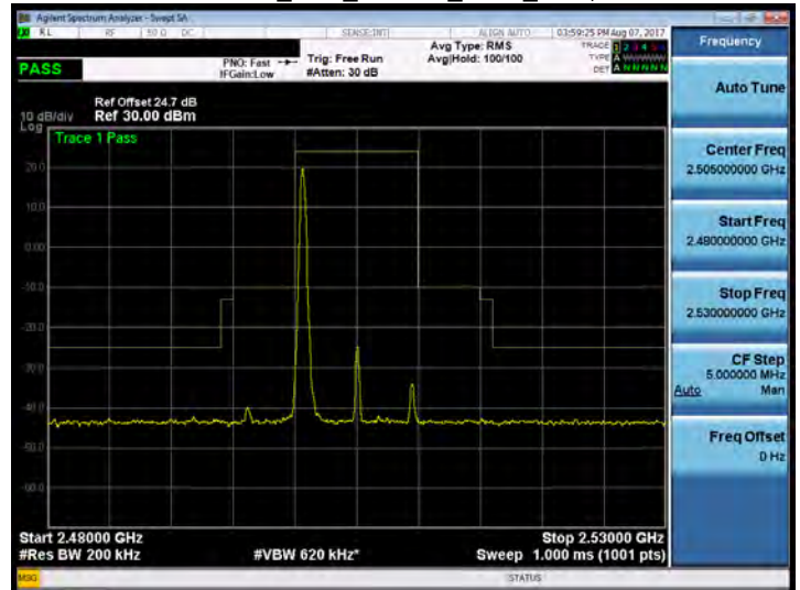
Band 7_10M_64QAM_LOW_RB1,0
