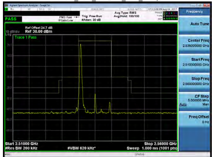
Band 7_10M_16QAM_MID_RB1,0
