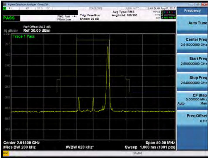
Band 38_10M_QPSK_HIGH_RB50,0
