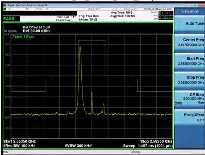
Band 7_5M_64QAM_HIGH_RB1,0
