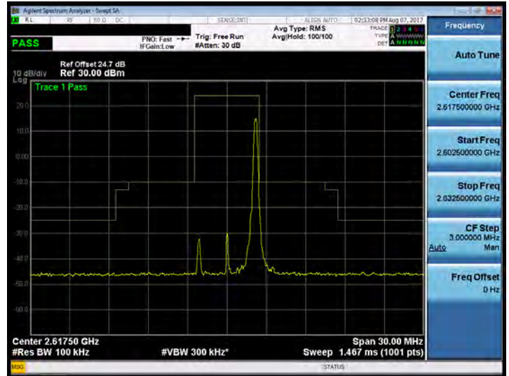
Band 38_5M_64QAM_HIGH_RB25,0
