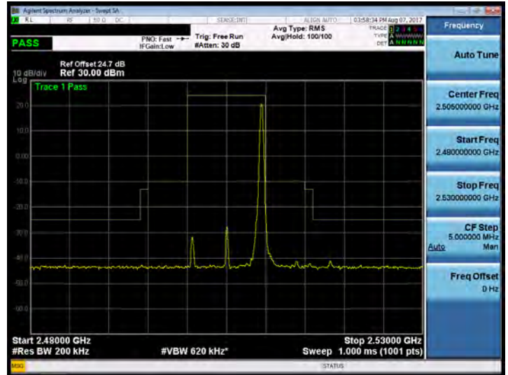
Band 7_10M_16QAM_LOW_RB50,0
