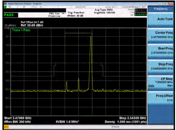
Band 7_15M_64QAM_LOW_RB75,0
