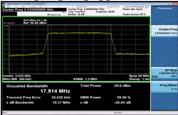
Band7_20MHz_64QAM_100_0_MidCH21100-2535
