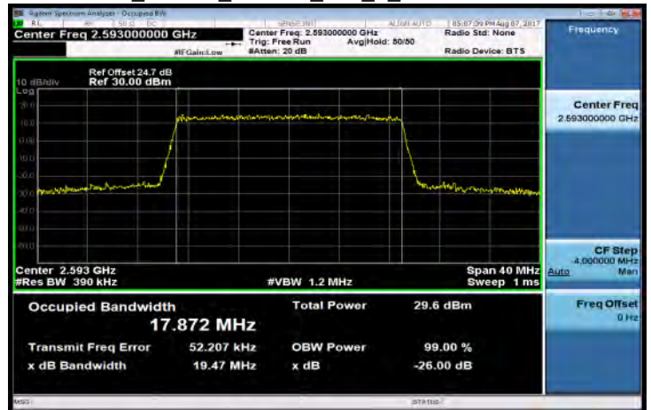
Band41_20MHz_16QAM_100_0_Mid CH40620-2593
