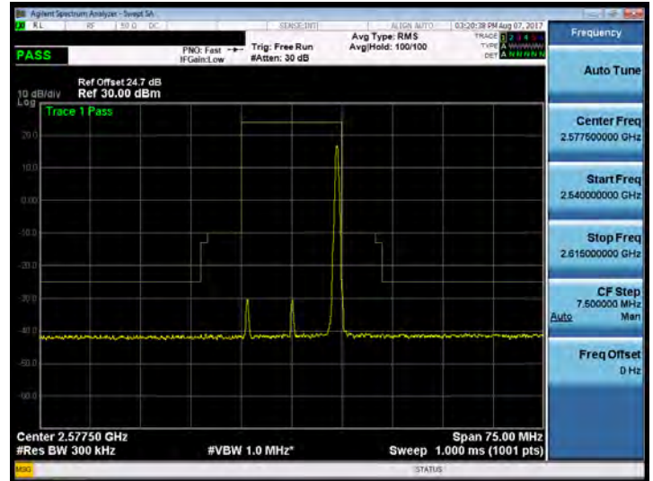
Band 38_15M_64QAM_LOW_RB75,0
