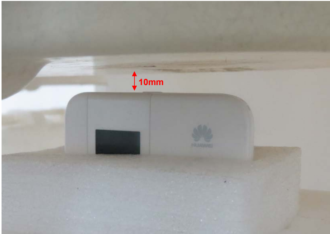
Picture 19: Test Position 5(Variant E5372s-32)
