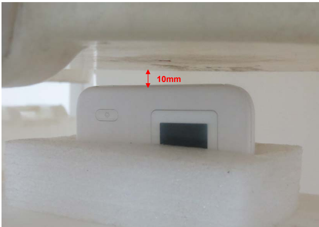
Picture 20: Test Position 6(Variant E5372s-32)
