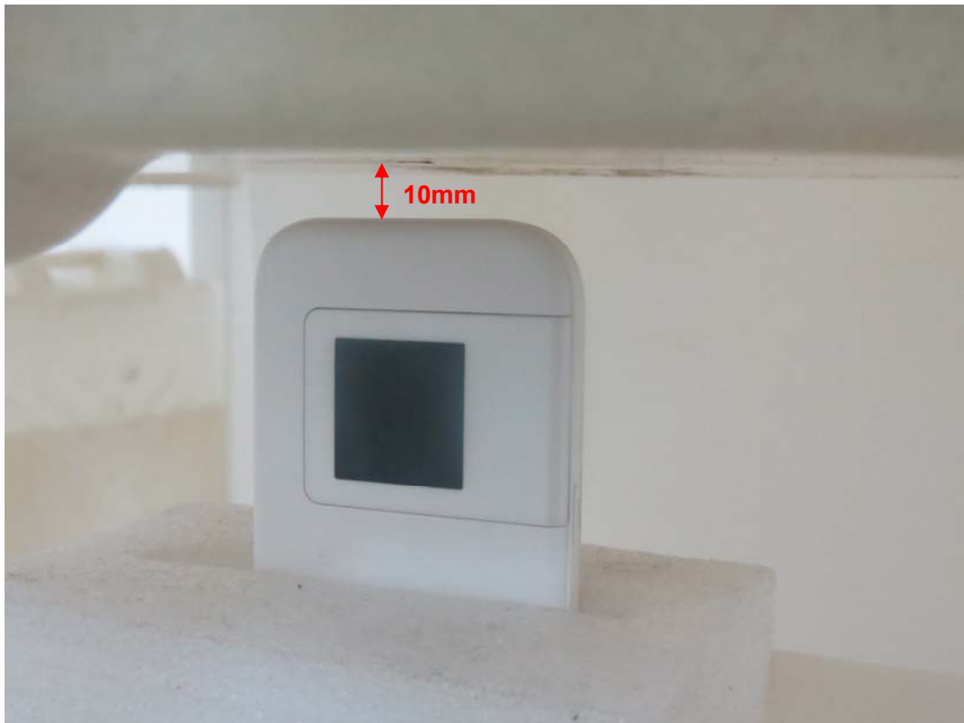
Picture 17: Test Position 3(Variant E5372s-32)
