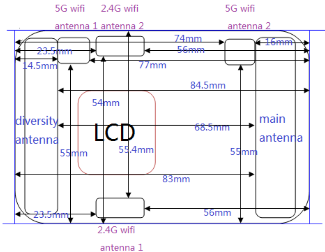
Picture 8: Constituents of the EUT
