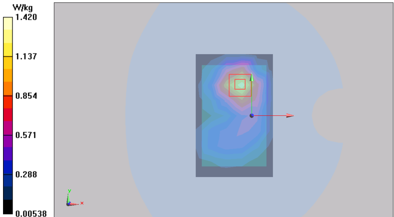
Figure 72 LTE Band 7 with Repeated SAR Test Position 6 Channel 21350
