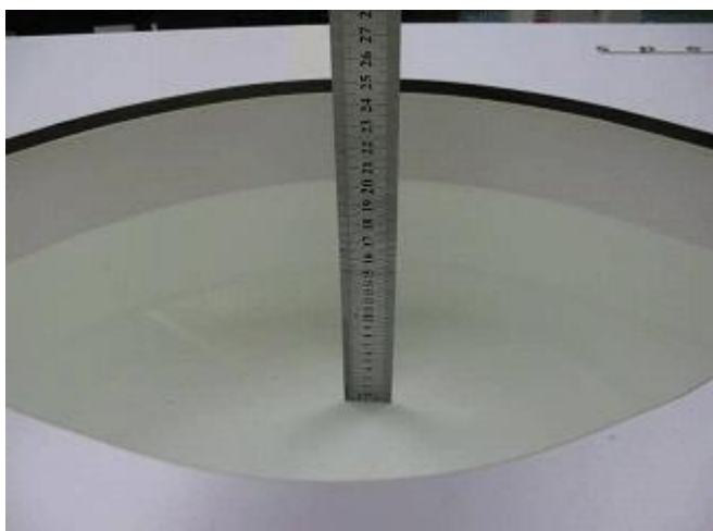
Photo 10: MSL1800MHz depth (15.00cm)
