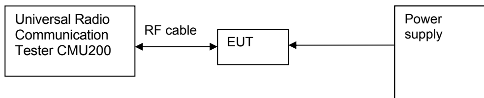
Figure 9. Test Set-up
