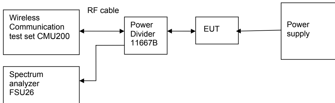
Figure 12. Test Set-up
