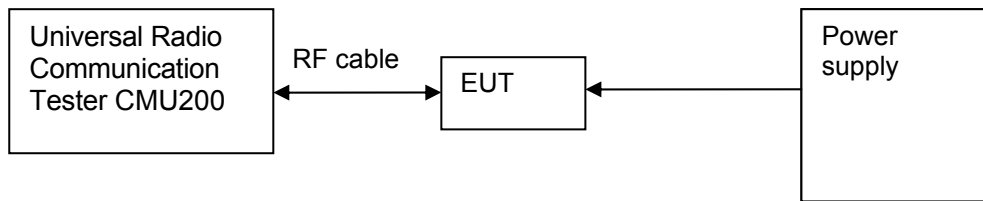
Figure 10. Test Set-up
