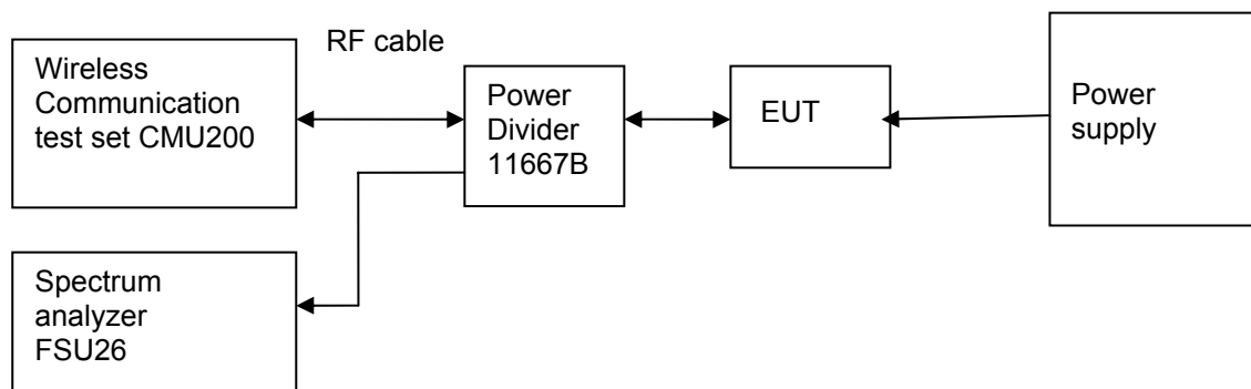
Figure 13. Test Set-up
