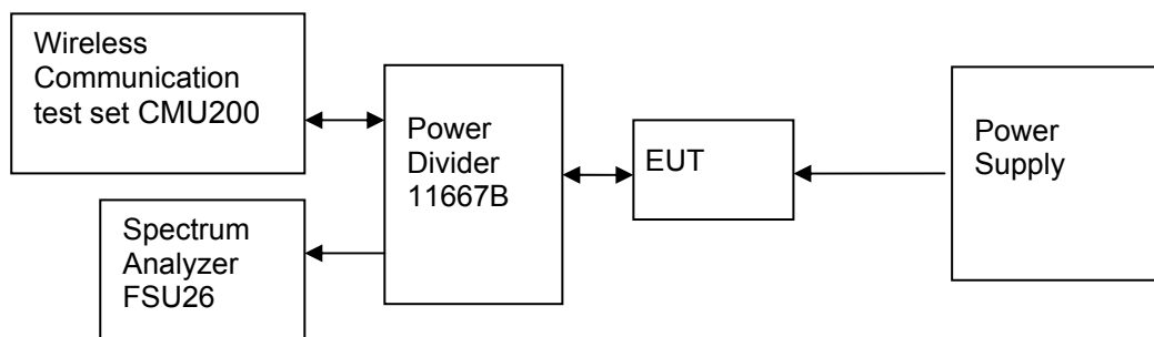
Figure 11. Test Set-up
