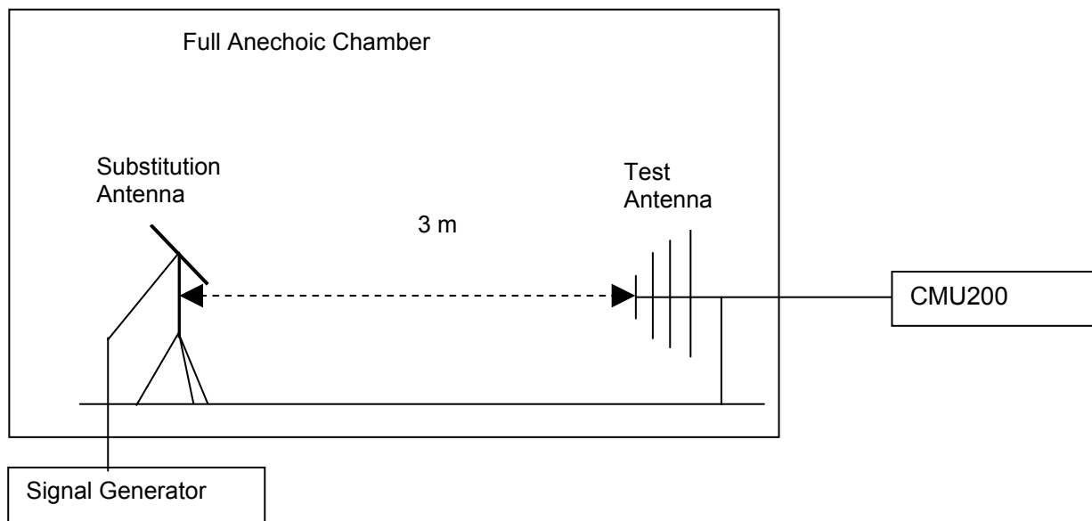
Figure 8. Test Set-up
