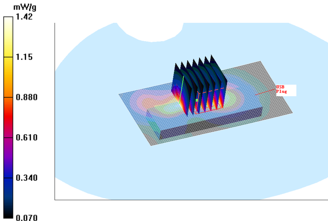
Figure 65 GSM 1900 EGPRS (1 timeslot in uplink) with BenQ Joybook R55V Test Position 5 Channel 810
