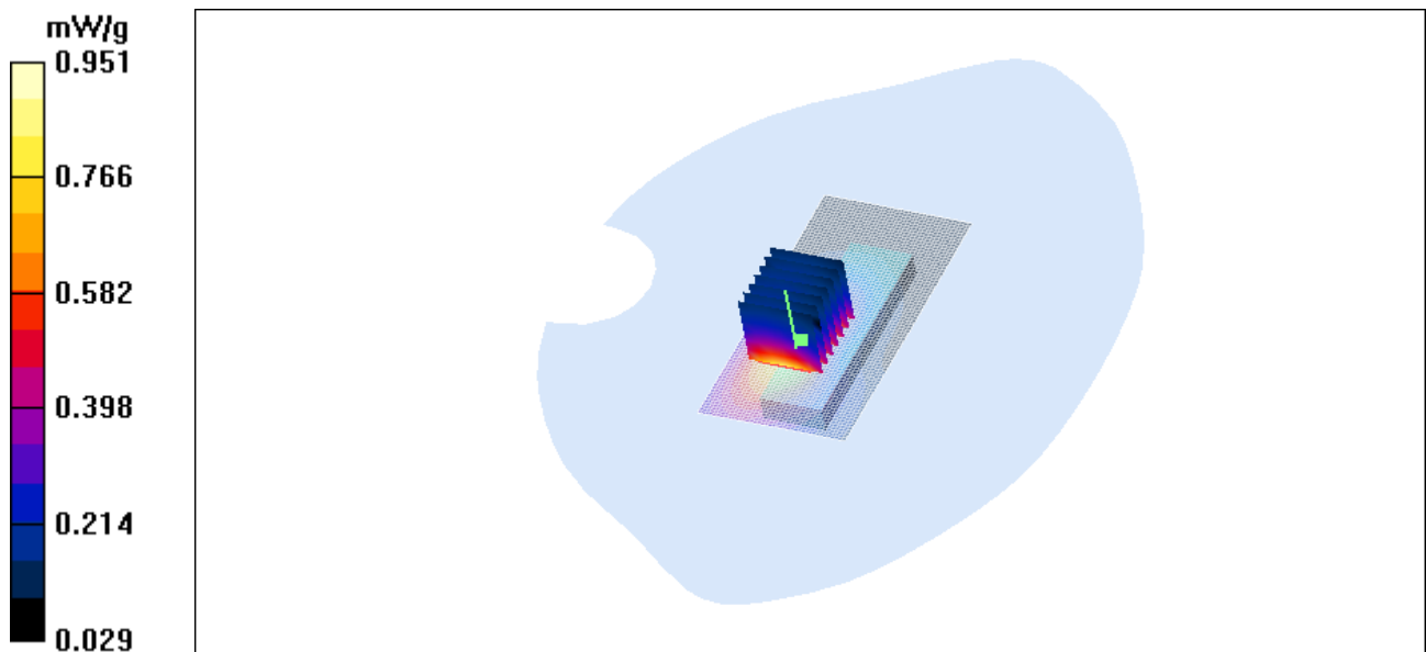
Figure 35 GSM 850 EGPRS (3 timeslots in uplink) with BenQ Joybook R55V Test Position 5 Channel 251
