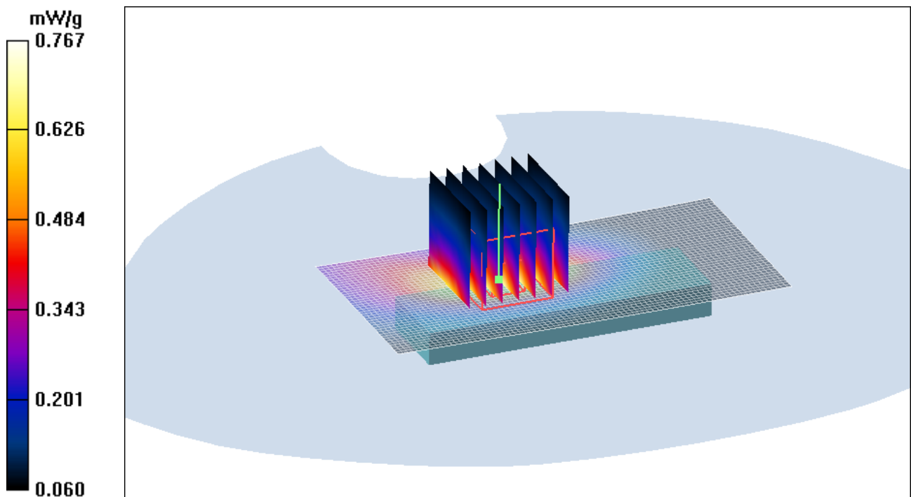
Figure 21 GSM 850 GPRS (1 timeslot in uplink) with IBM T61 Test Position 1 Channel 192
