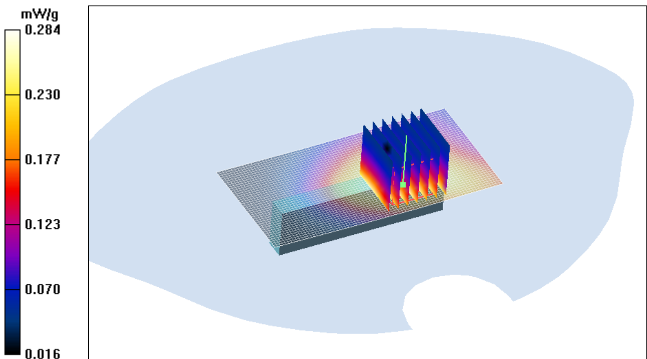
Figure 25 GSM 850 GPRS (3 timeslots in uplink) with IBM T61 Test Position 3 Channel 192
