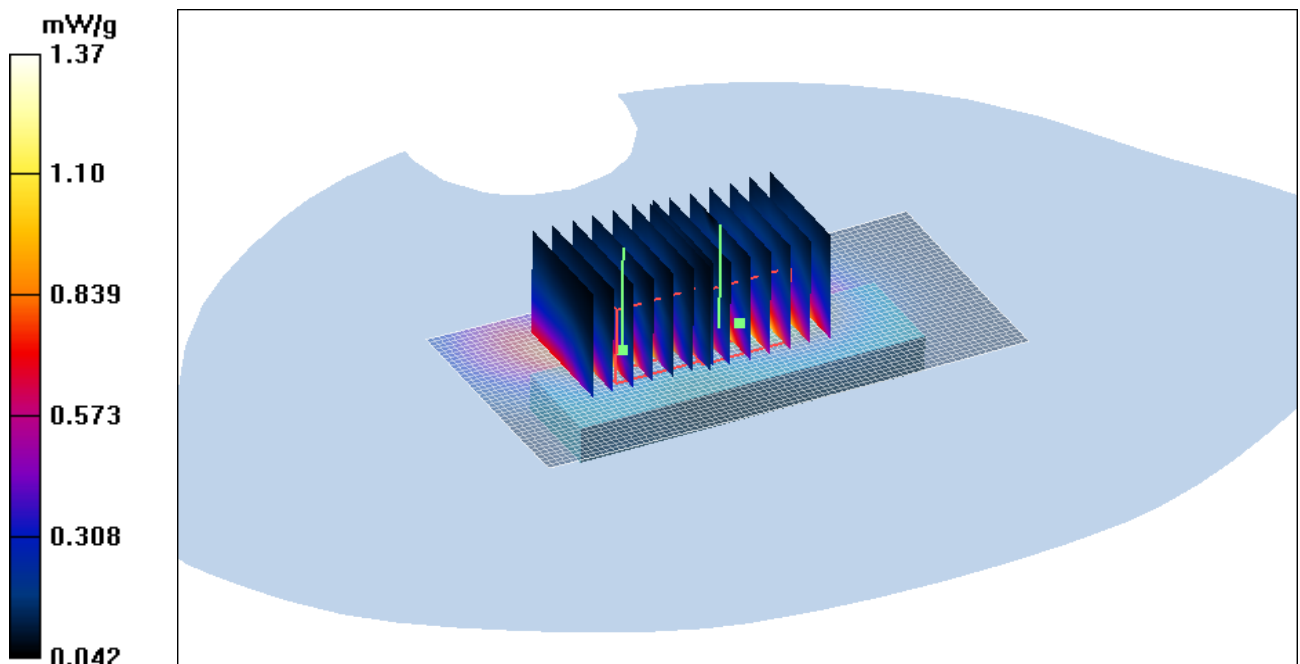
Figure 59 GSM 1900 GPRS (1 timeslot in uplink) with BenQ Joybook R55V Test Position 5 Channel 810
