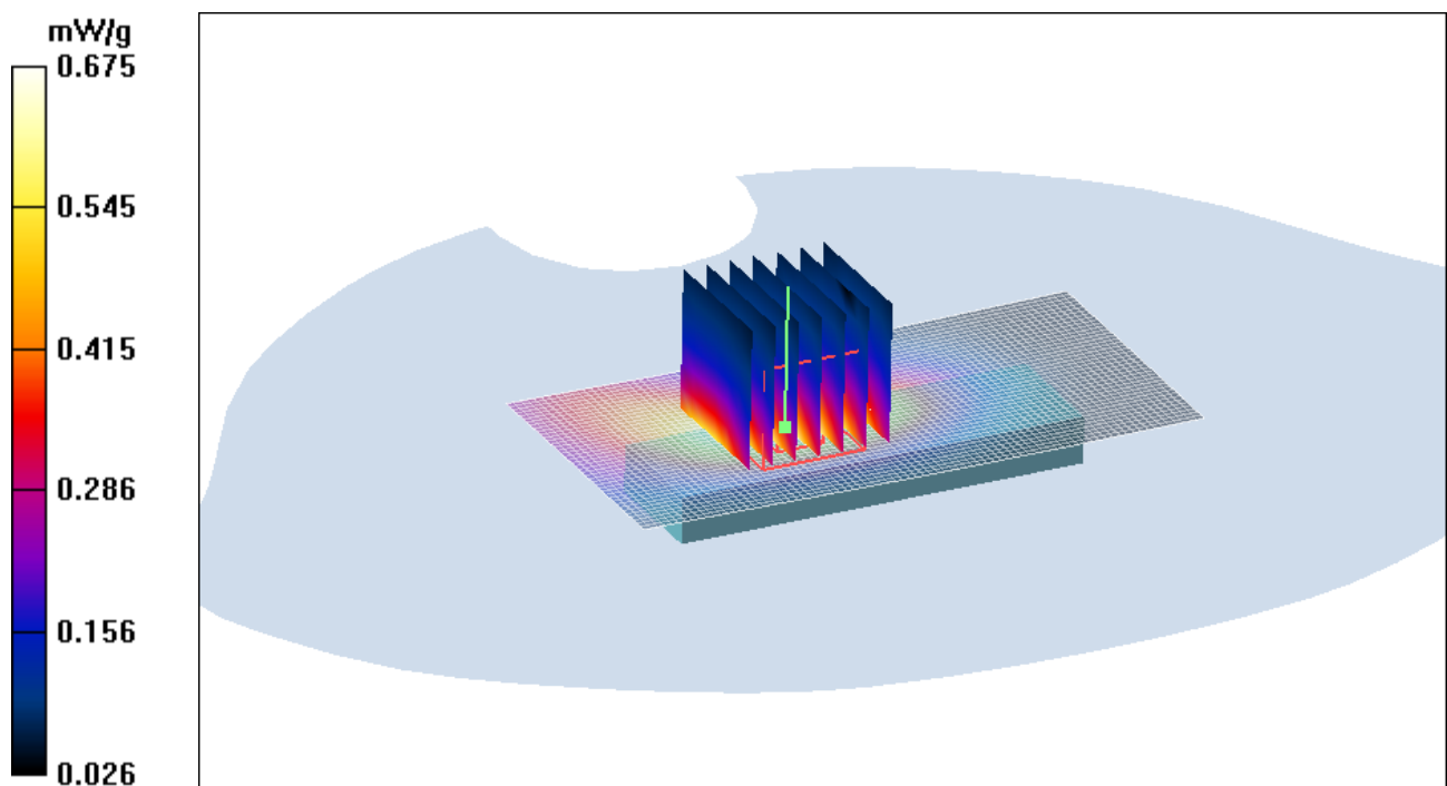
Figure 15 GSM 850 GPRS (4 timeslots in uplink) with IBM T61 Test Position 1 Channel 192
