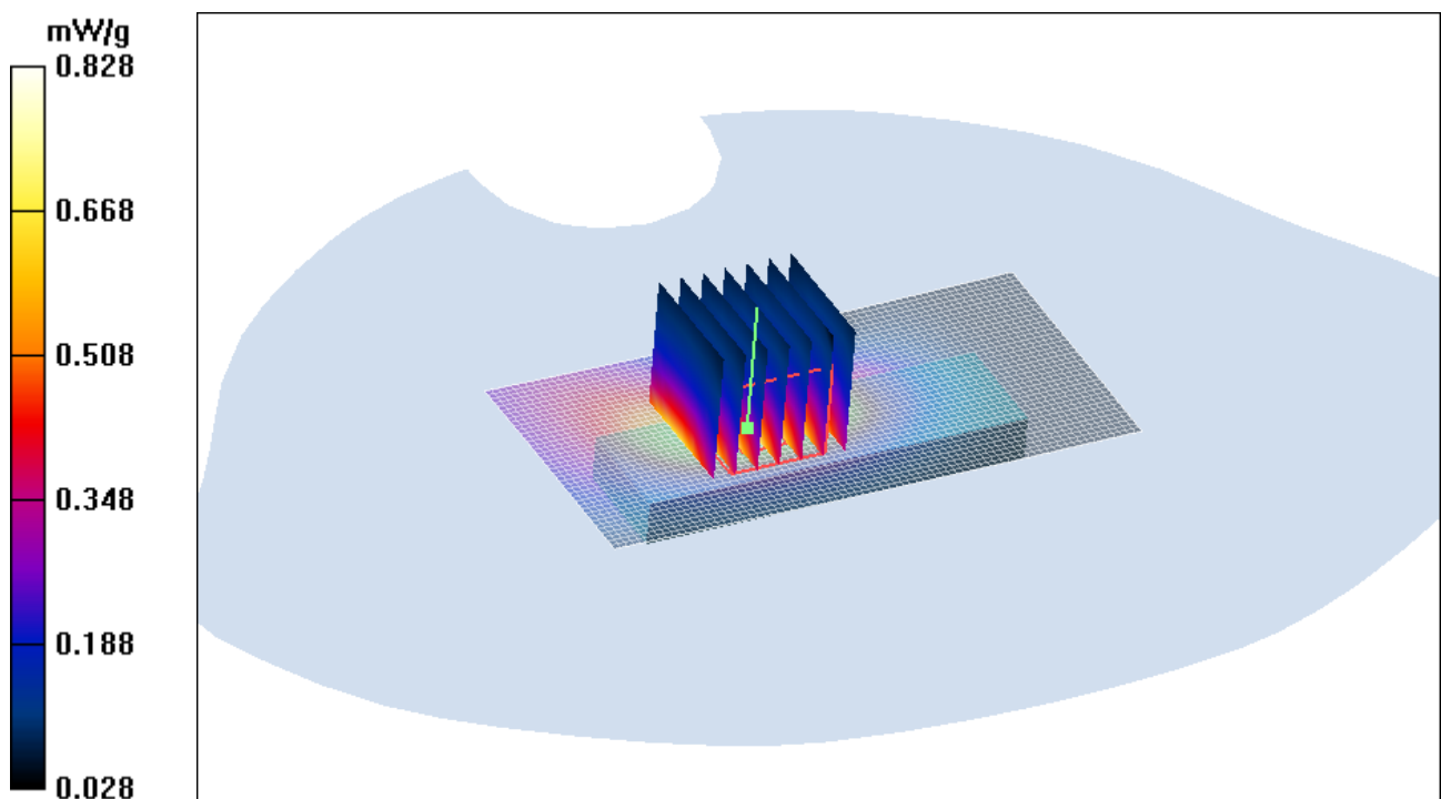
Figure 17 GSM 850 GPRS (3 timeslots in uplink) with IBM T61 Test Position 1 Channel 192
