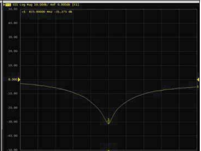
Impedance Test-Head Return Loss Test-Head
