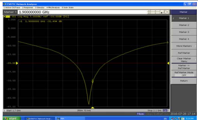
Return Loss-Body
