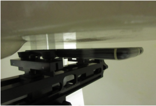
Photo 7: Left Side_10mm
