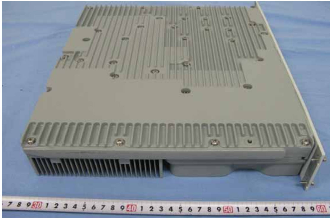
Figure 5, Bottom view of CRFU-AWS
