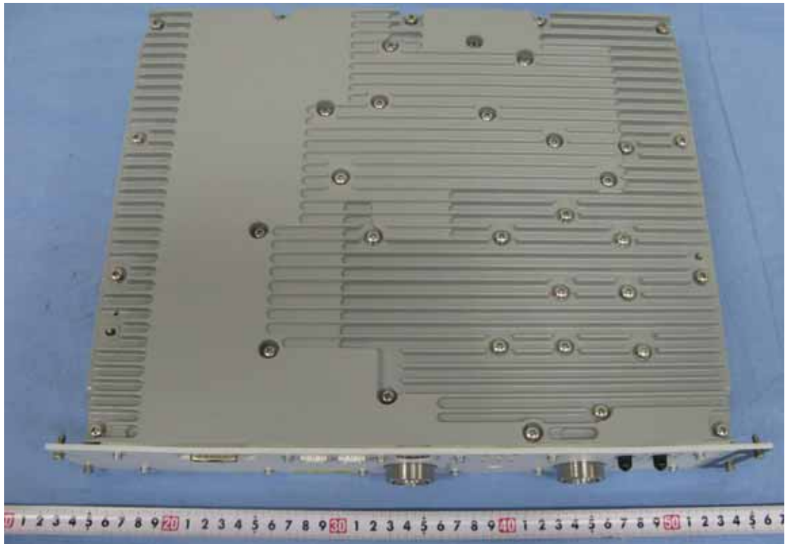
Figure 3, Left Side view of CRFU-AWS
