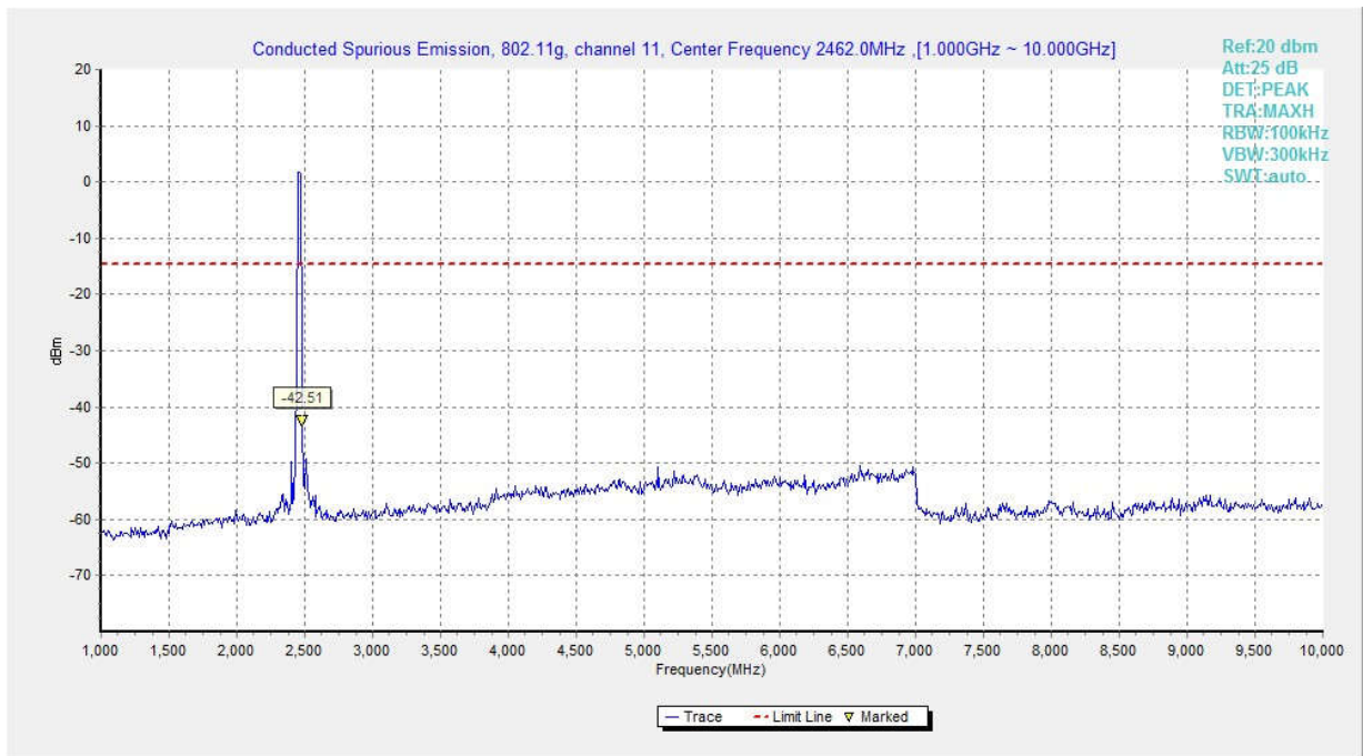
Fig.36 Conducted Spurious Emission (802.11g, Ch11, 1 GHz-10 GHz)
