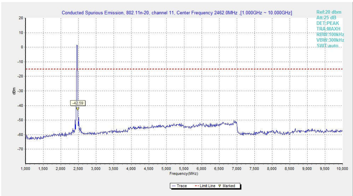
Fig.42 Conducted Spurious Emission (802.11n-20MHz, Ch11, 1 GHz-10 GHz)
