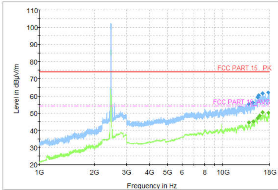
Fig.57 Radiated Spurious Emission (802.11n-20MHz, Ch11, 1 GHz-18 GHz)
