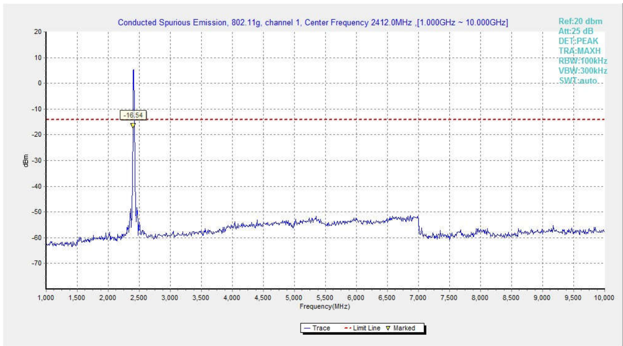
Fig.32 Conducted Spurious Emission (802.11g, Ch1, 1 GHz-10 GHz)
