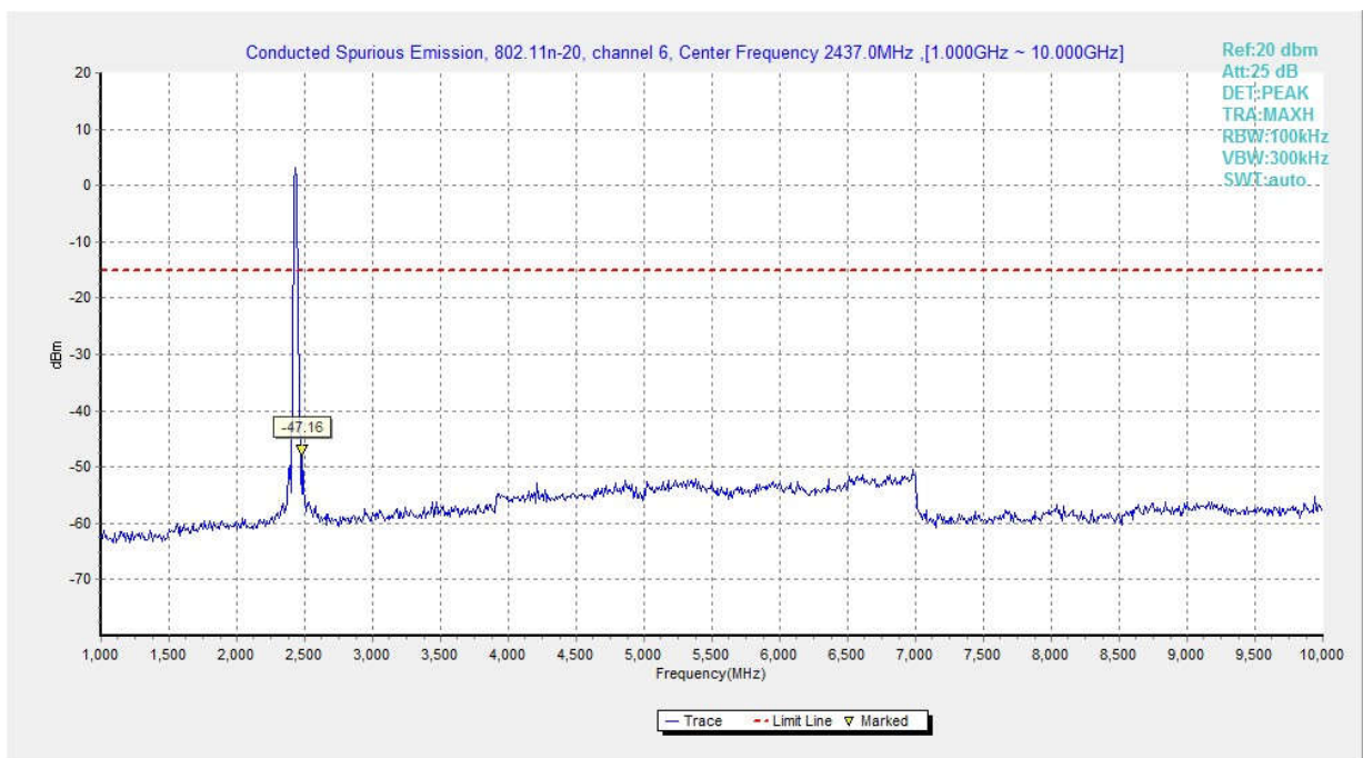
Fig.40 Conducted Spurious Emission (802.11n-20MHz, Ch6, 1 GHz-10 GHz)
