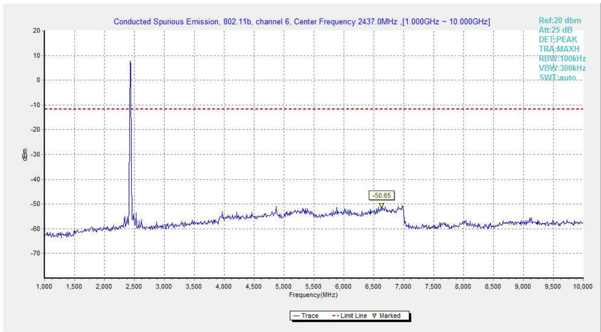
Fig.28 Conducted Spurious Emission (802.11b, Ch6, 1 GHz-10 GHz)
