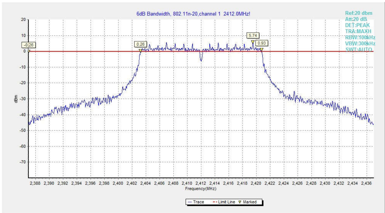
Fig.16 6dB Bandwidth (802.11 n-20MHz, Ch 1)
