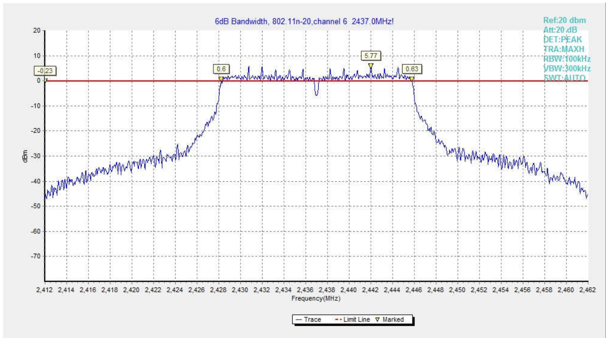
Fig.17 6dB Bandwidth (802.11 n-20MHz, Ch 6)
