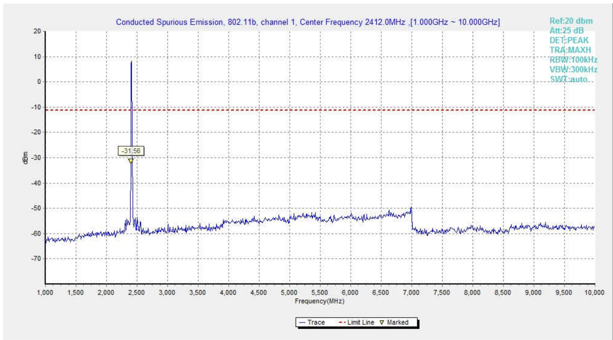
Fig.26 Conducted Spurious Emission (802.11b, Ch1, 1 GHz-10 GHz)
