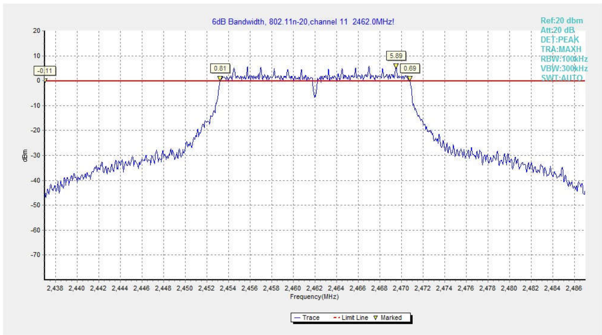
Fig.18 6dB Bandwidth (802.11 n-20MHz, Ch 11)
