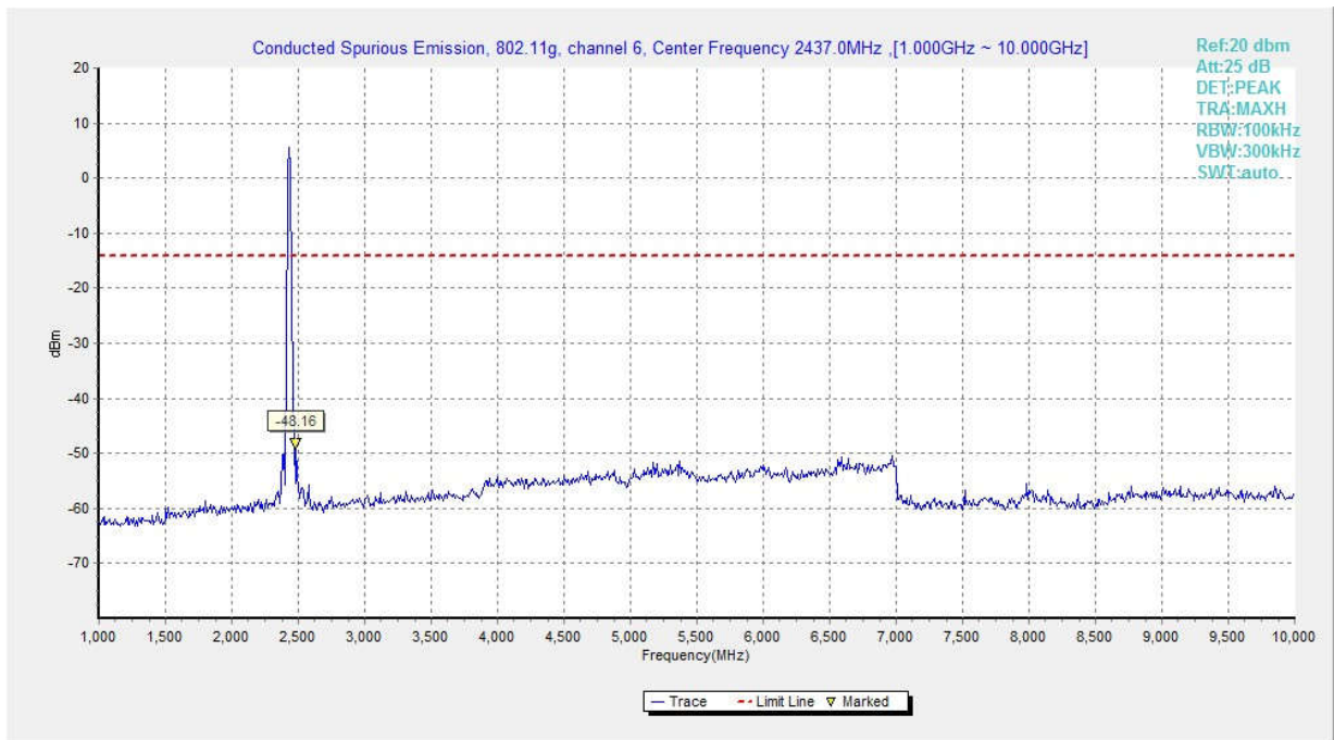
Fig.34 Conducted Spurious Emission (802.11g, Ch6, 1 GHz-10 GHz)
