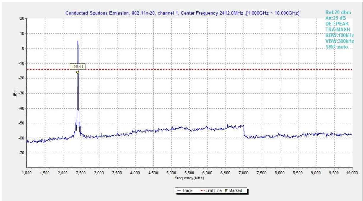
Fig.38 Conducted Spurious Emission (802.11n-20MHz, Ch1, 1 GHz-10 GHz)
