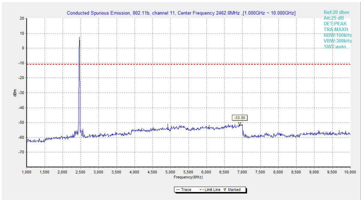
Fig.30 Conducted Spurious Emission (802.11b, Ch11, 1 GHz-10 GHz)
