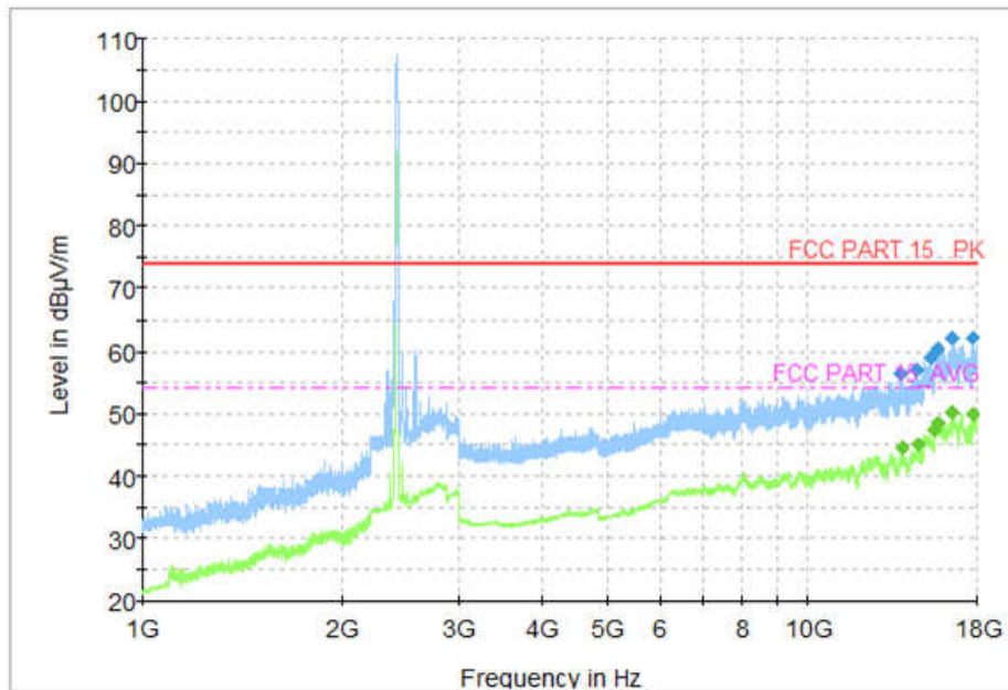
Fig.55 Radiated Spurious Emission (802.11n-20MHz, Ch1, 1 GHz-18 GHz)
