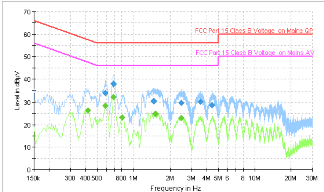
Fig.64 AC Power line Conducted Emission (Idle, AE1)
