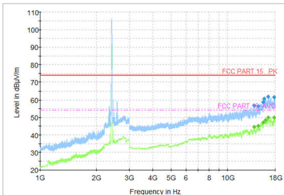
Fig.56 Radiated Spurious Emission (802.11n-20MHz, Ch6, 1 GHz-18 GHz)
