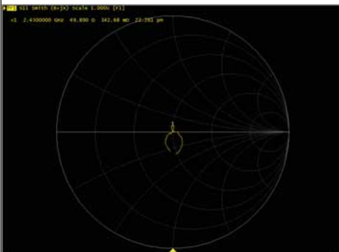
Impedance Test-Body
