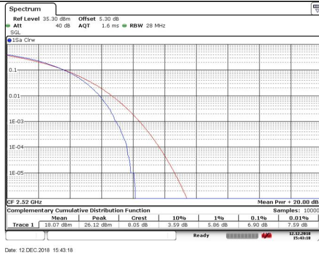
CA_7C_64QAM_100RB+100RB_21199+21001_PCC:100RB@0_SCC:100RB@0
