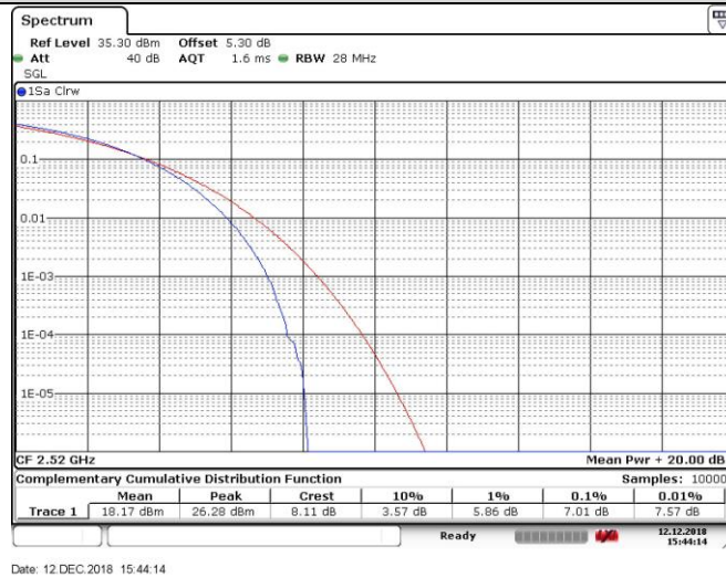
CA_7C_16QAM_100RB+100RB_21001+21199_PCC:100RB@0_SCC:100RB@0
