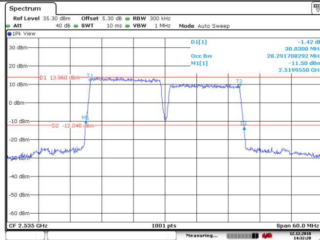
CA_7C_QPSK_75RB+75RB_21025+21175_PCC:75RB@0_SCC:75RB@0
