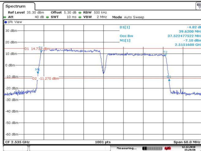
CA_7C_16QAM_100RB+100RB_21001+21199_PCC:100RB@0_SCC:100RB@0
