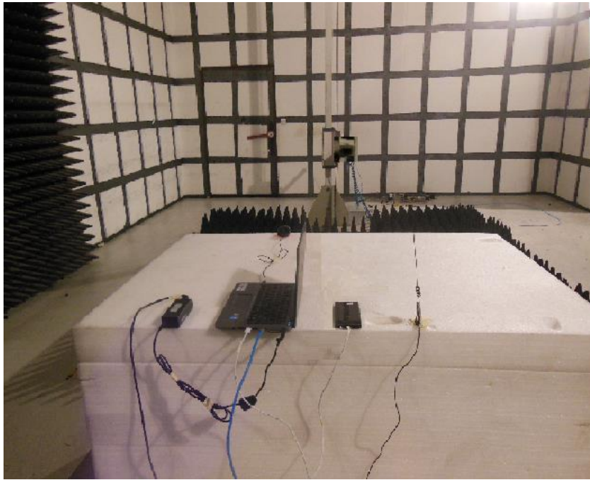
Radiated Disturbance Emissions (18GHz to 40GHz)
