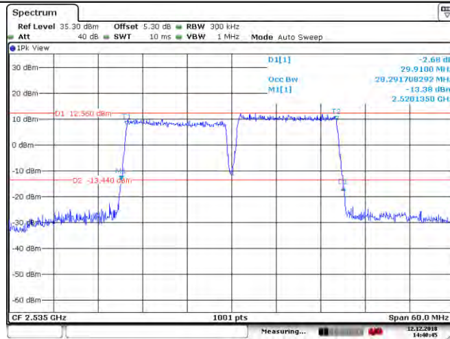
CA_7C_16QAM_75RB+75RB_21175+21025_PCC:75RB@0_SCC:75RB@0
