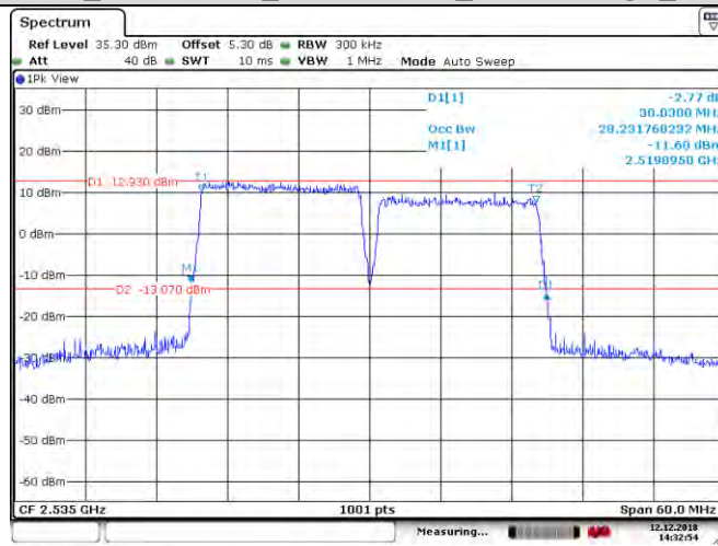
CA_7C_16QAM_75RB+75RB_21025+21175_PCC:75RB@0_SCC:75RB@0
