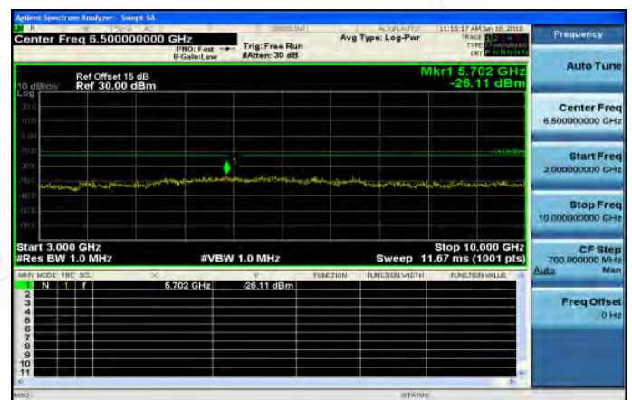
3GHz~10GHz_Band26_5MHz_QPSK_1_0_HighCH26765
