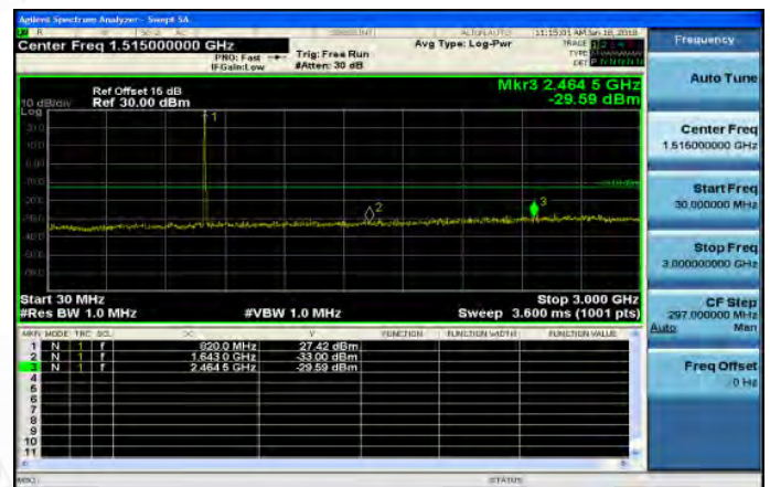
30MHz~3GHz_Band26_5MHz_QPSK_1_0_HighCH26765
