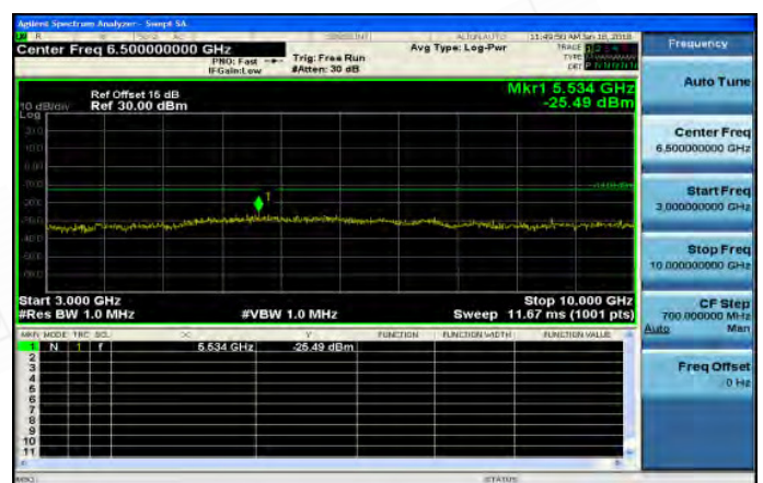
3GHz~10GHz_Band26_3MHz_QPSK_1_0_HighCH26775
