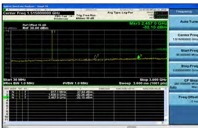
30MHz~3GHz_Band26_3MHz_QPSK_1_0_MidCH26740
