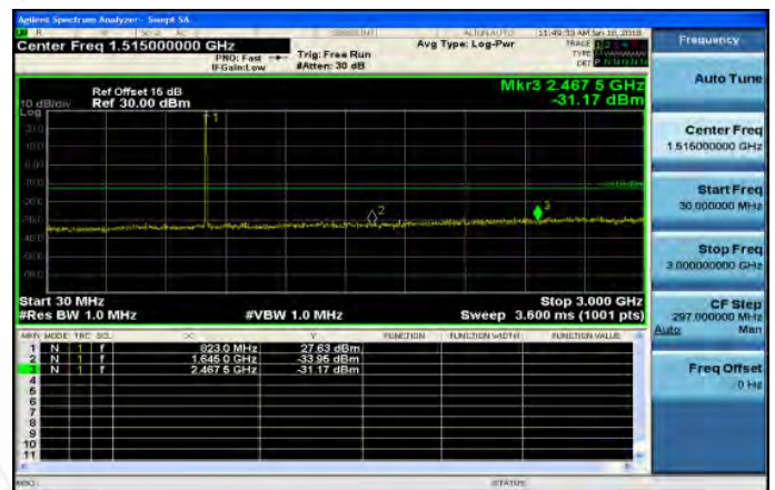
30MHz~3GHz_Band26_3MHz_QPSK_1_0_HighCH26775
