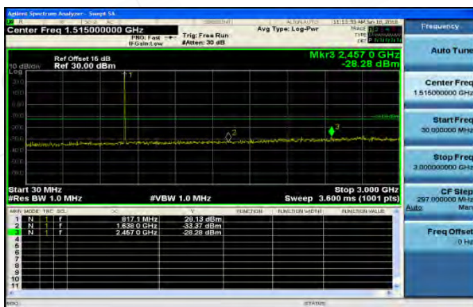
30MHz~3GHz_Band26_5MHz_QPSK_1_0_MidCH26740
