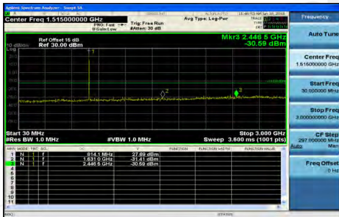
30MHz~3GHz_Band26_3MHz_QPSK_1_0_LowCH26705
