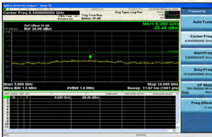
3GHz~10GHz_Band26_3MHz_QPSK_1_0_LowCH26705
