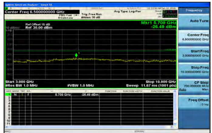
3GHz~10GHz_Band26_5MHz_QPSK_1_0_MidCH26740
