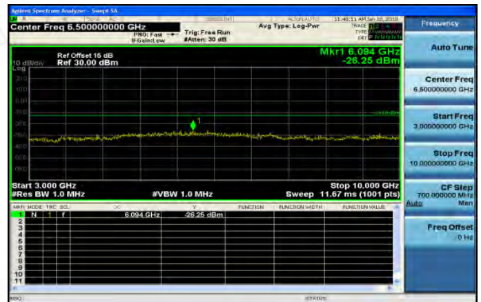
3GHz~10GHz_Band26_3MHz_QPSK_1_0_MidCH26740
