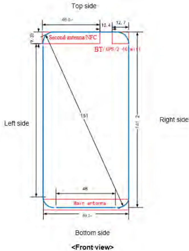
Fig.17 Antenna position of EUT
