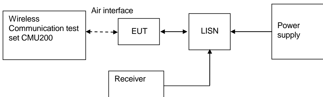
Figure 3. Test Set-up
