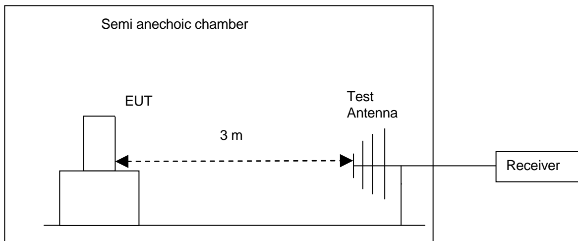
Figure 2. Test set-up
