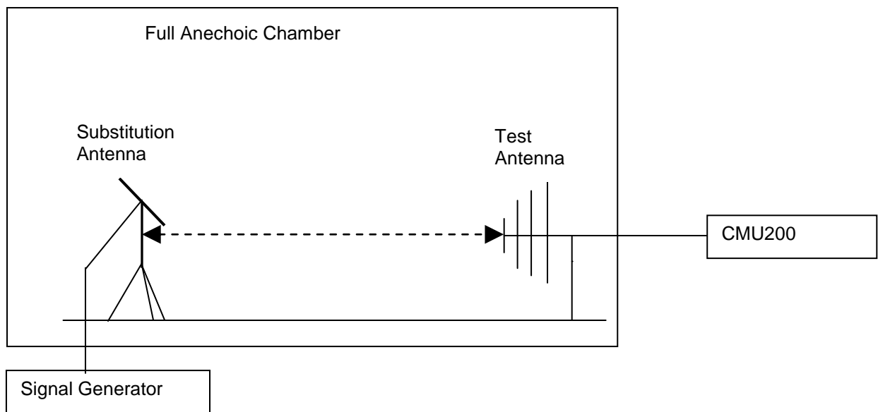
Figure 1. Test Set-up
