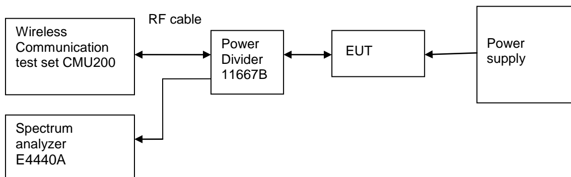
Figure 6. Test Set-up
