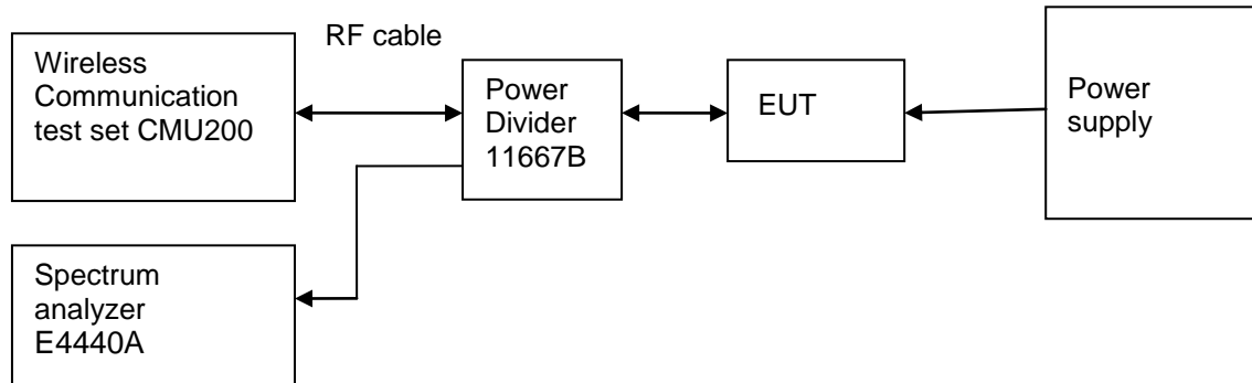
Figure 5. Test Set-up
