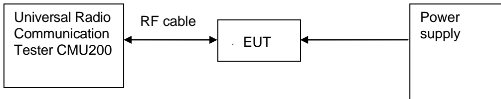
Figure 2. Test Set-up
