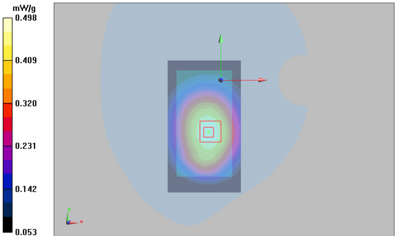
Figure 15 Body, Towards Ground, CDMA Cellular Channel 777
