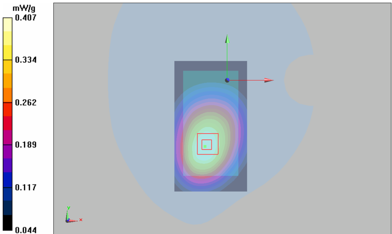
Figure 18 Body, Towards Phantom, CDMA Cellular Channel 384
