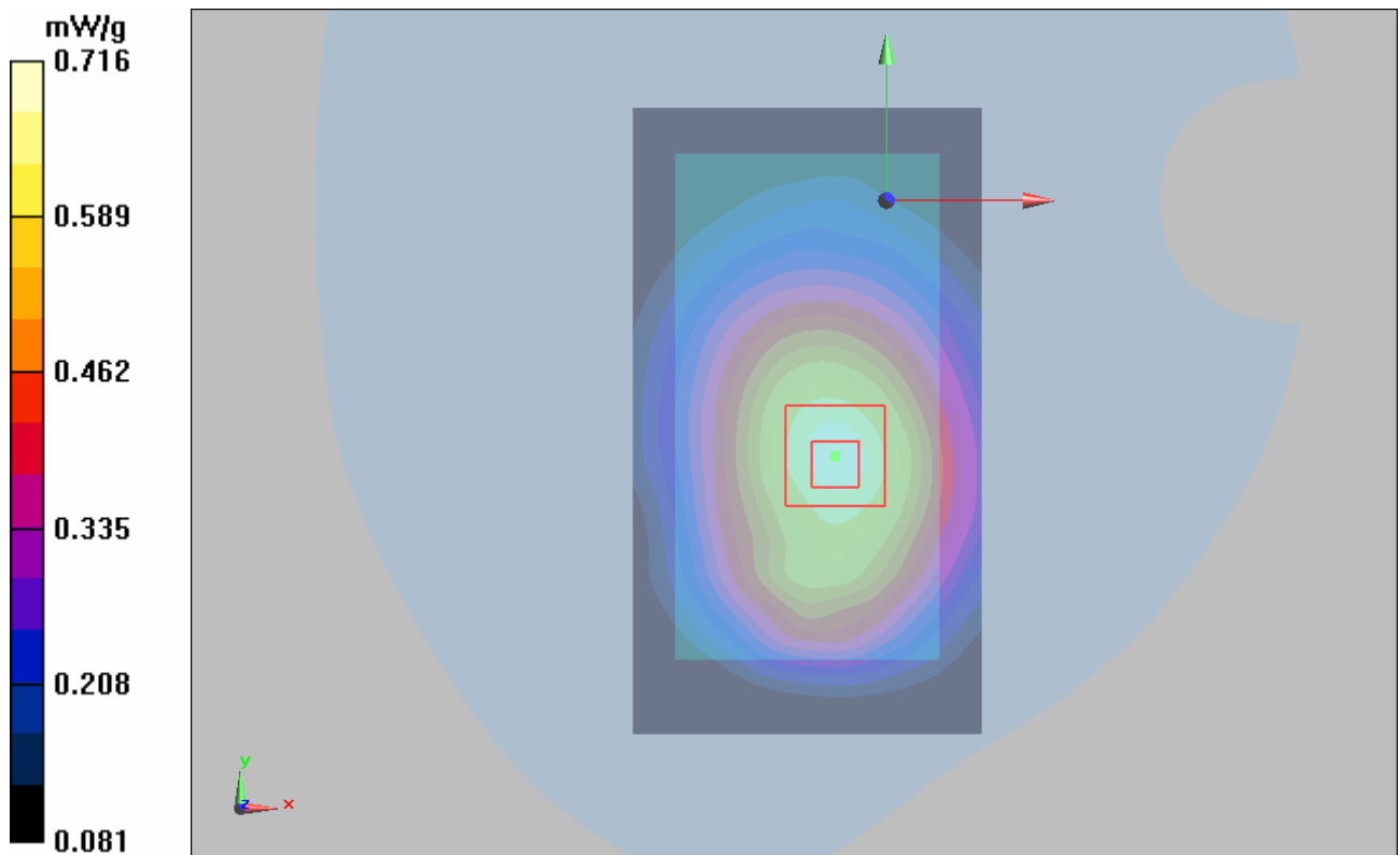
Figure 20 Body, Towards Ground, CDMA Cellular EVDO Rev.0 Channel 1013
