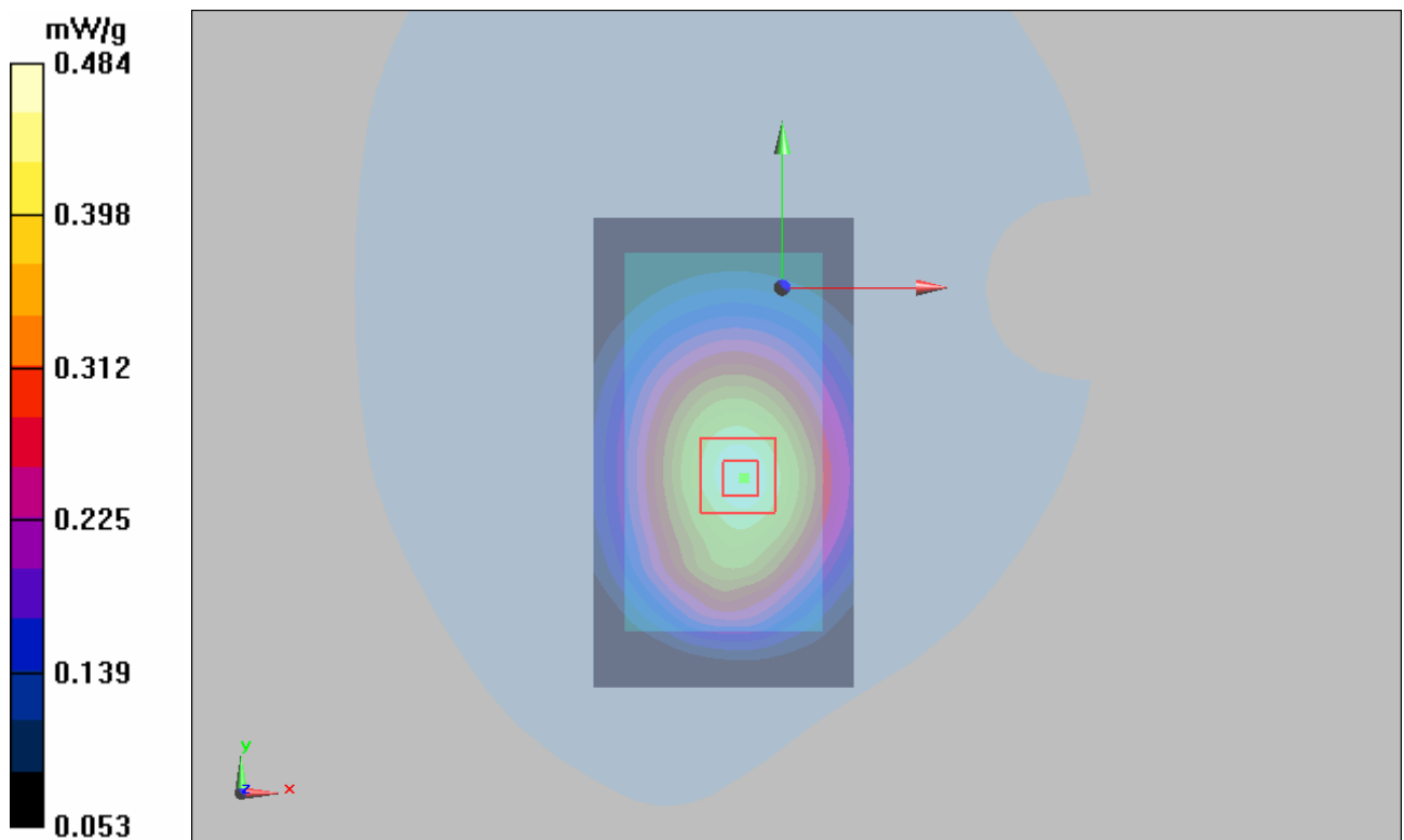
Figure 16 Body, Towards Ground, CDMA Cellular Channel 384
