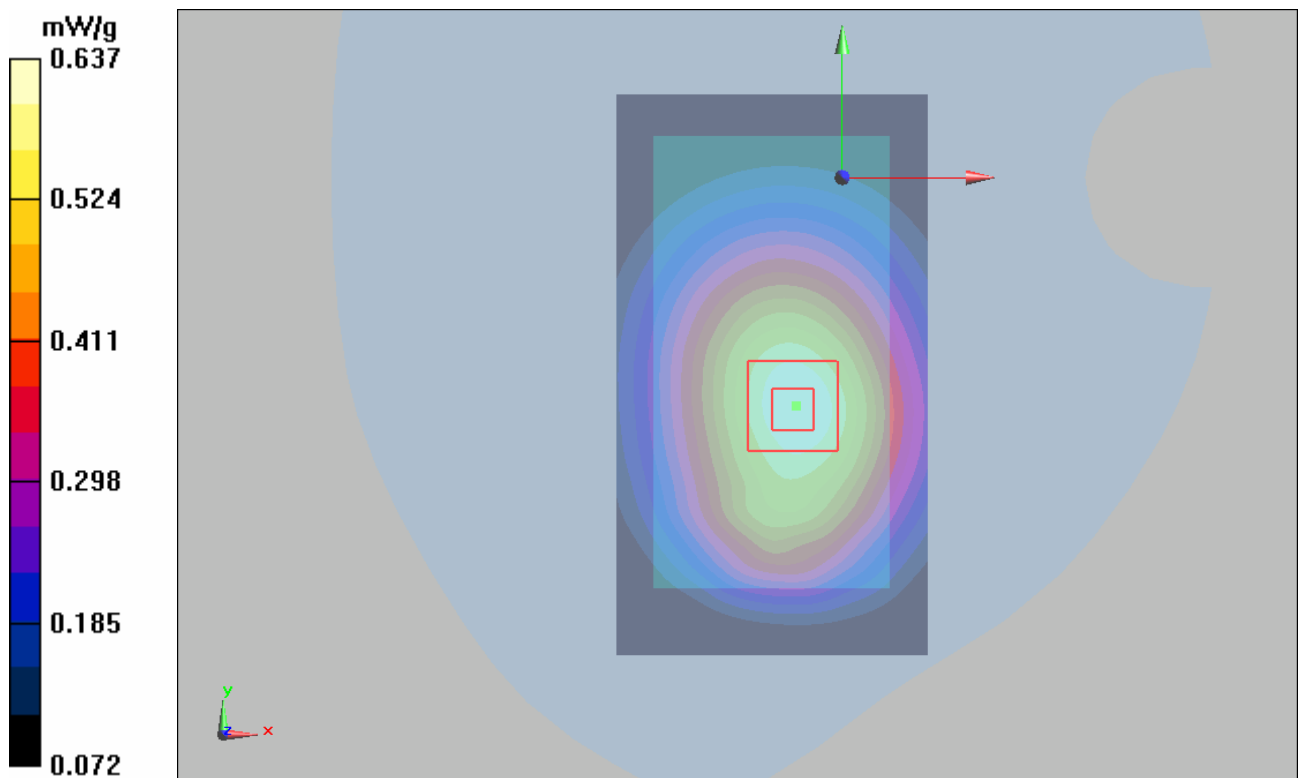
Figure 17 Body, Towards Ground, CDMA Cellular Channel 1013
