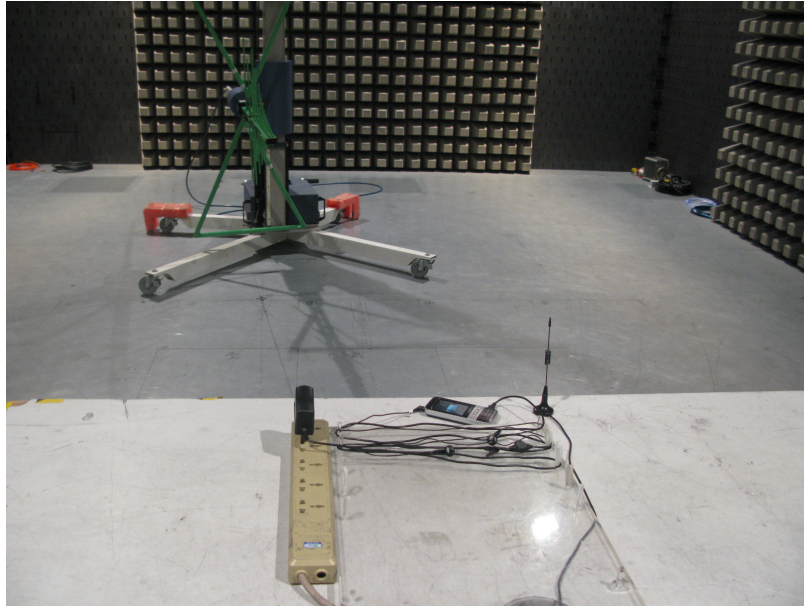
Radiated Disturbance
