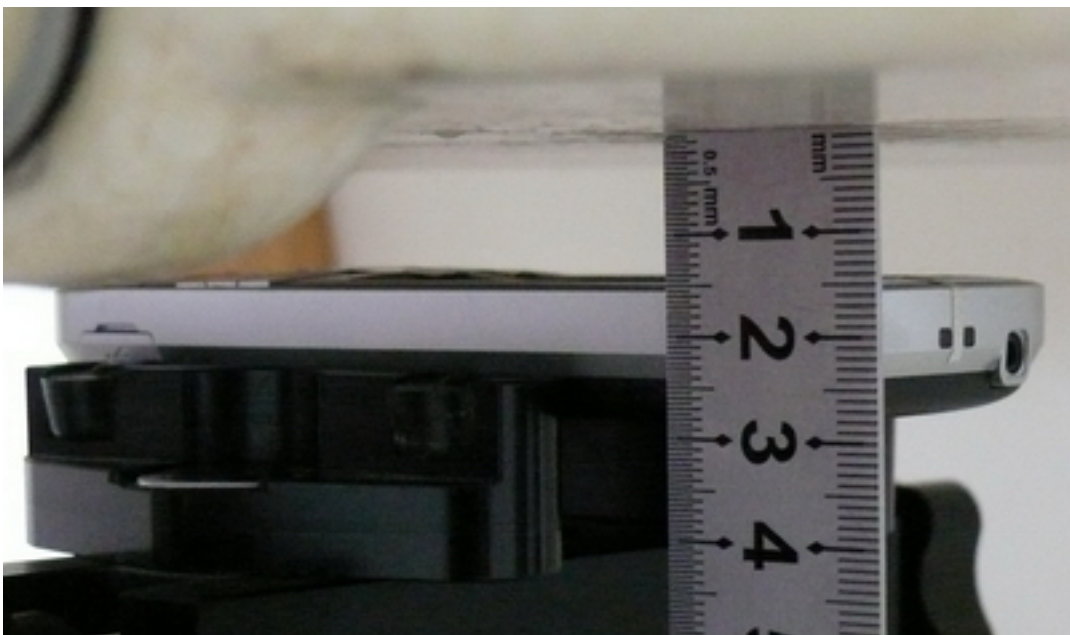
Picture 10 Body, towards the Phantom, the distance from handset to the bottom of the Phantom is 15mm)
