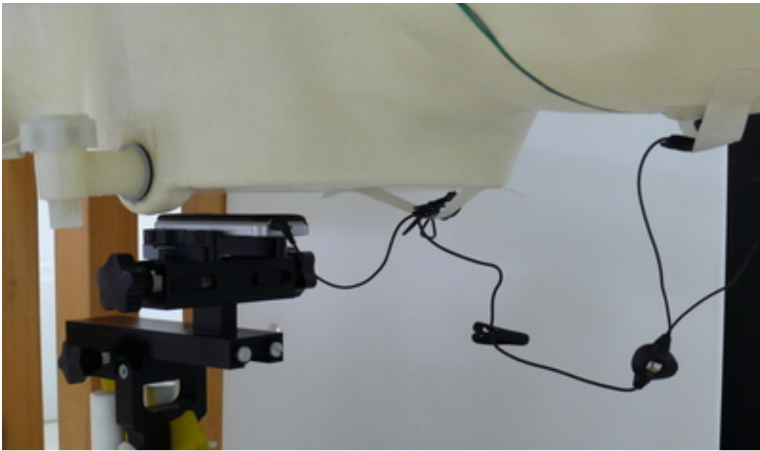
Picture 11 Body with earphone, towards the ground, the distance from handset to the bottom of the Phantom is 15mm)
