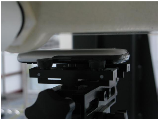
Photo 12: HUAWEI M635 body worn rear side with Bluetooth Headset (15mm distance)
