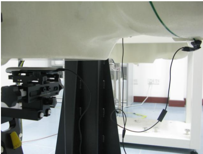
Photo 11: HUAWEI M635 body worn rear side with Headset (15mm distance)
