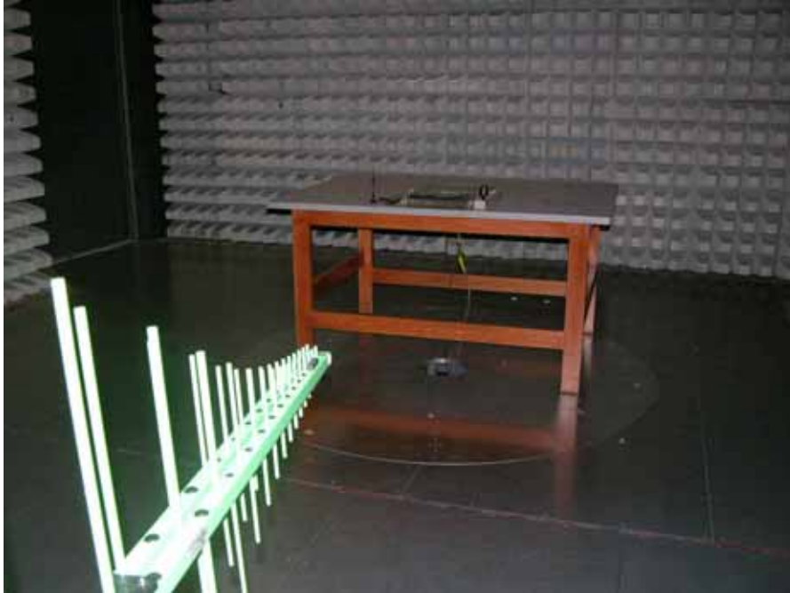
Radiated Disturbance
