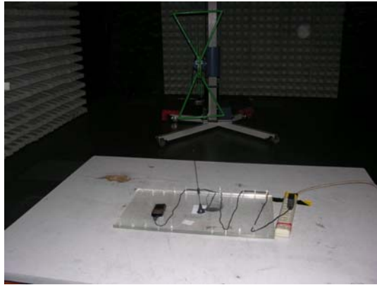
Radiated Disturbance
