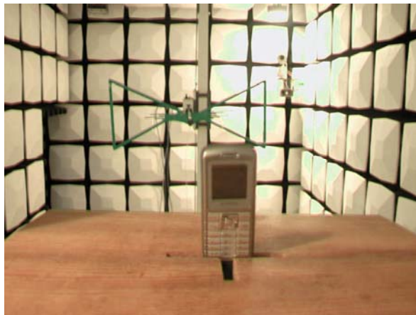
Radiated Spurious Emission (below 2GHz)
