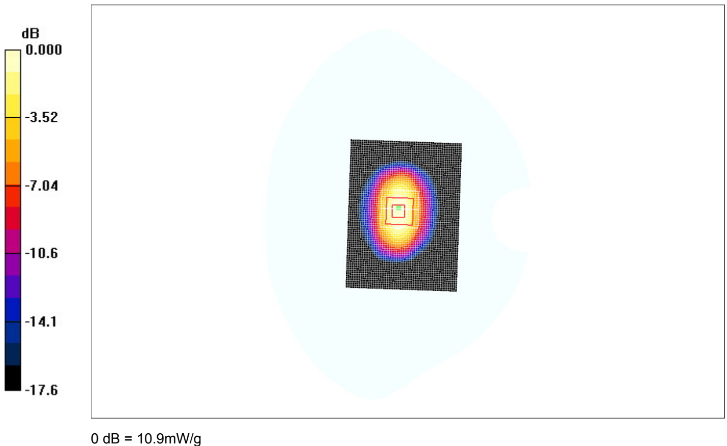
Figure.43 System Performance Check 1900MHz 250mW
