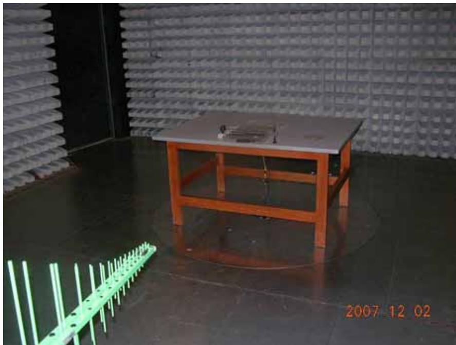
Radiated Disturbance
