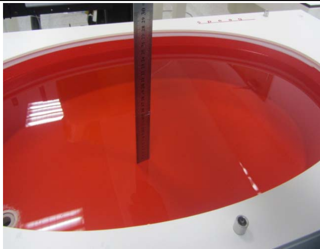
Photo 4: Body2450MHz depth (15.1cm)
