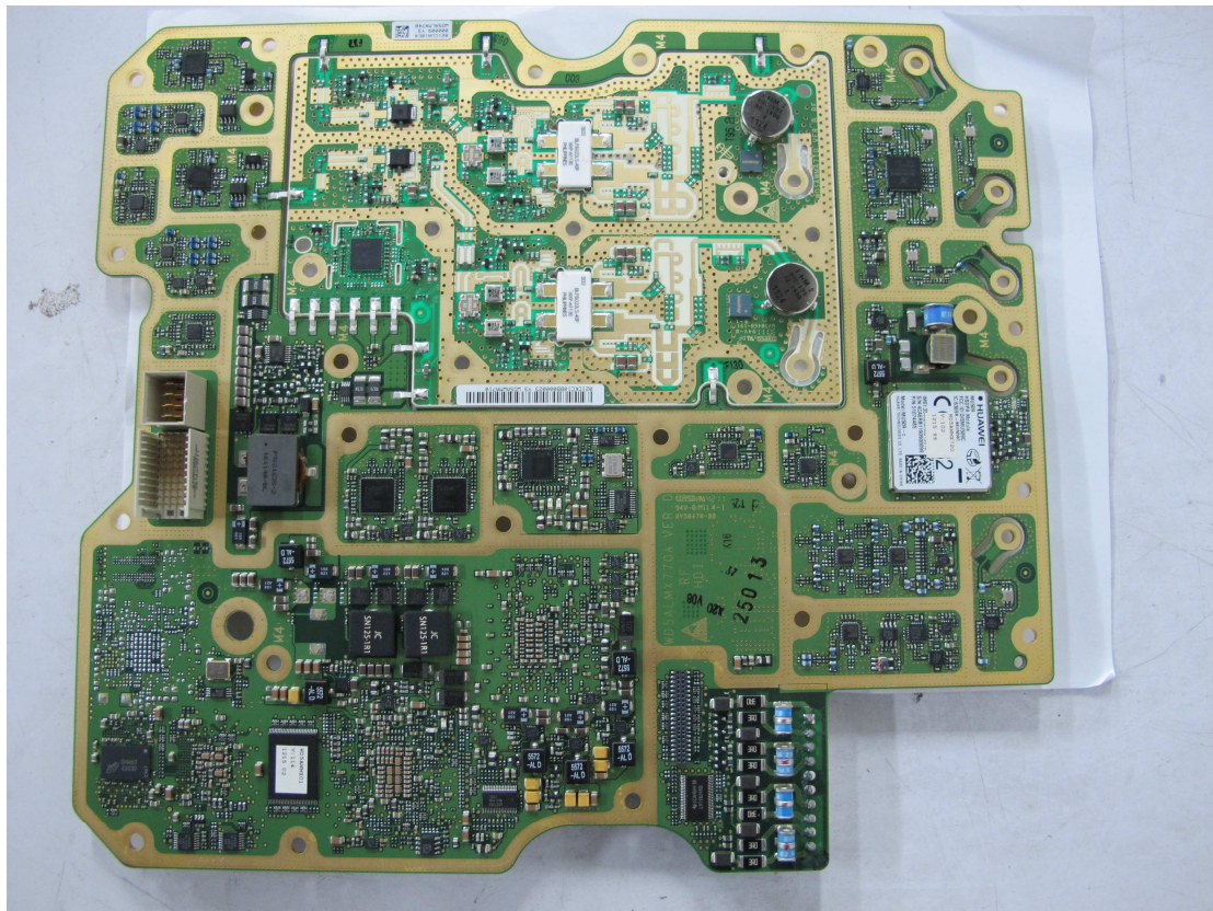
Photo-09 Internal View - Radio Board (top)
