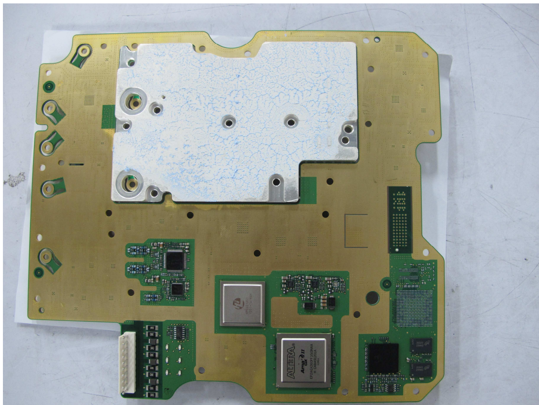
Photo-10 Internal View - Radio Board (bottom)
