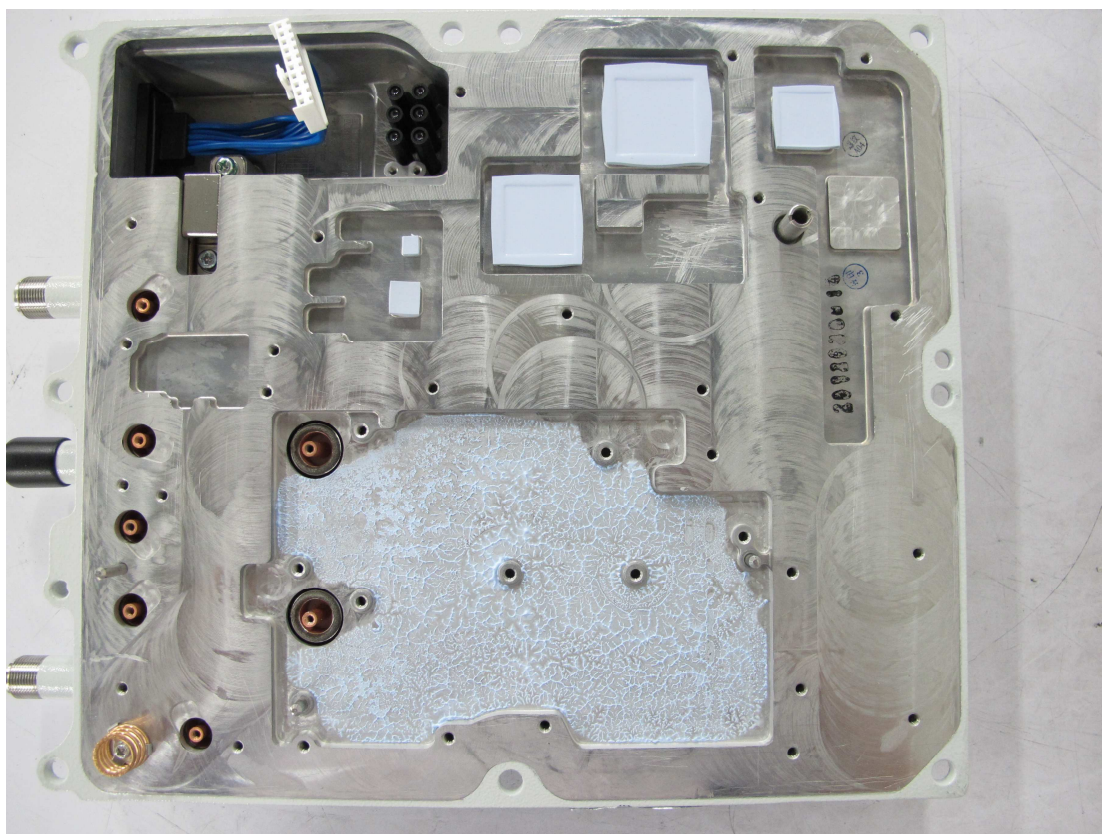
Photo-11 Internal View - Remove Radio Board
