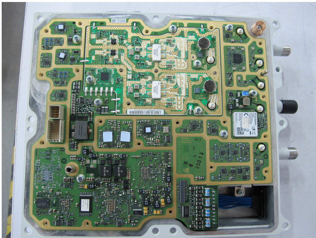
Photo-08 Internal View - Radio Unit
