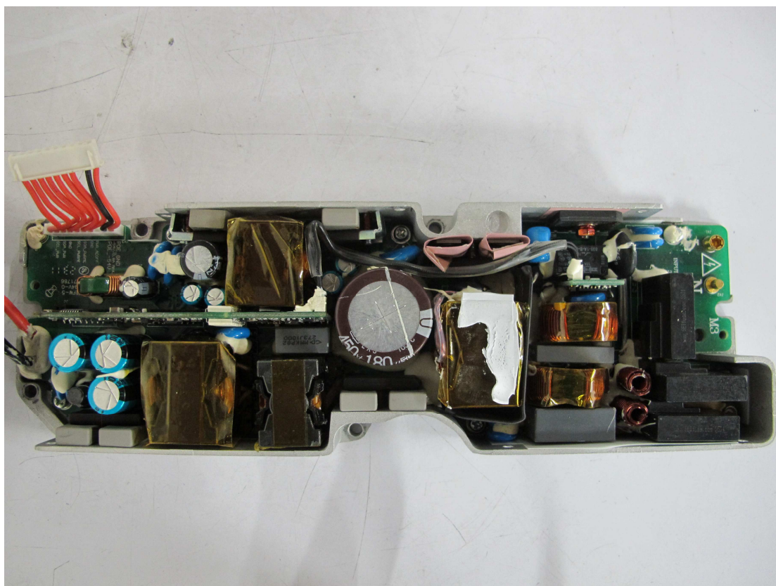
Photo-05 Internal View - Power Board with "GYE" Log (internal)
