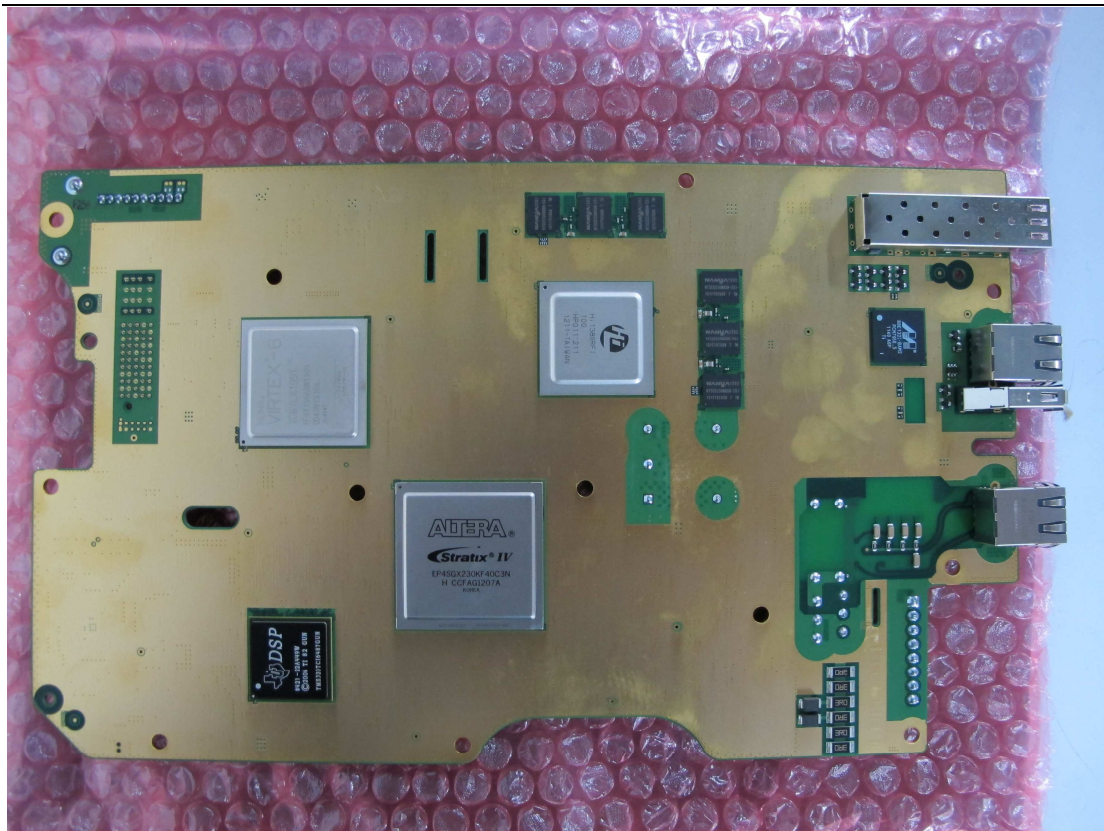
Photo-03 Internal View - Baseband Board (bottom)
