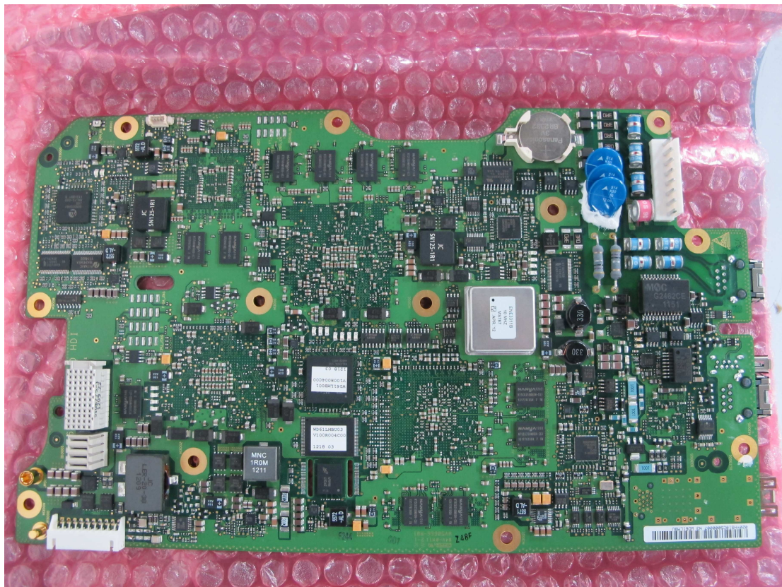
Photo-02 Internal View - Baseband Board (top)
