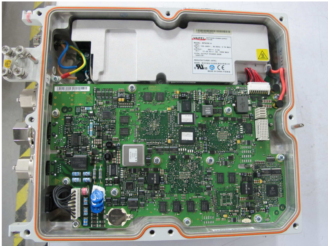
Photo-01 Internal View - Digital Unit
