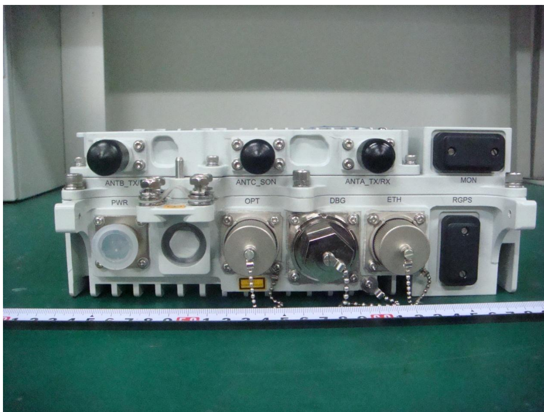
Photo-04 External view – Front(with interface cover)
