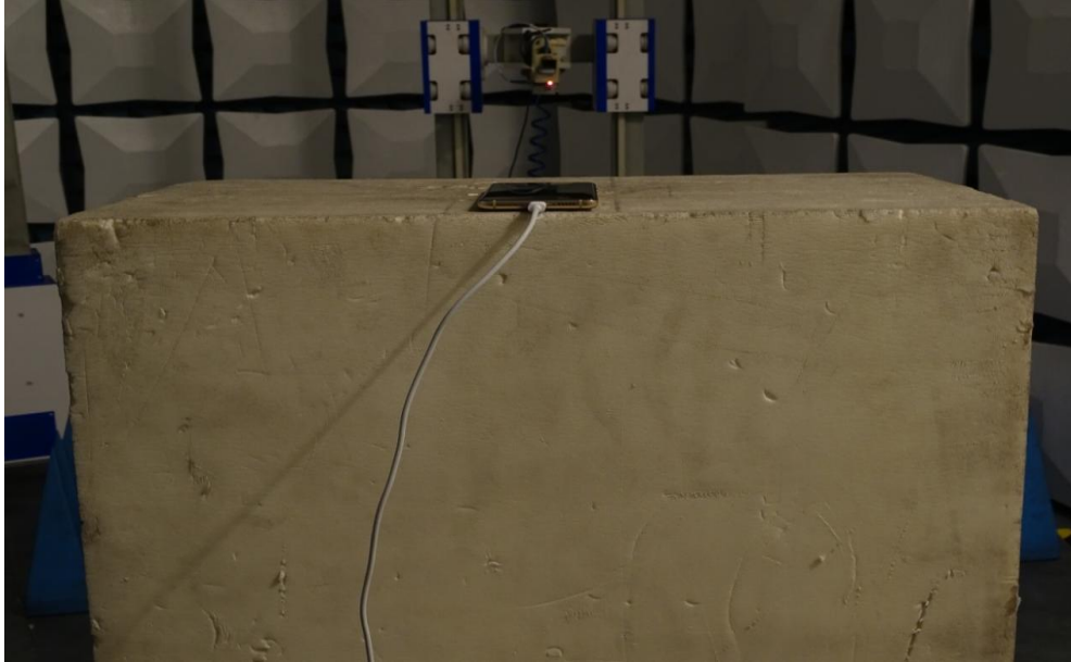
Radiated Spurious Emission (above 18GHz)
