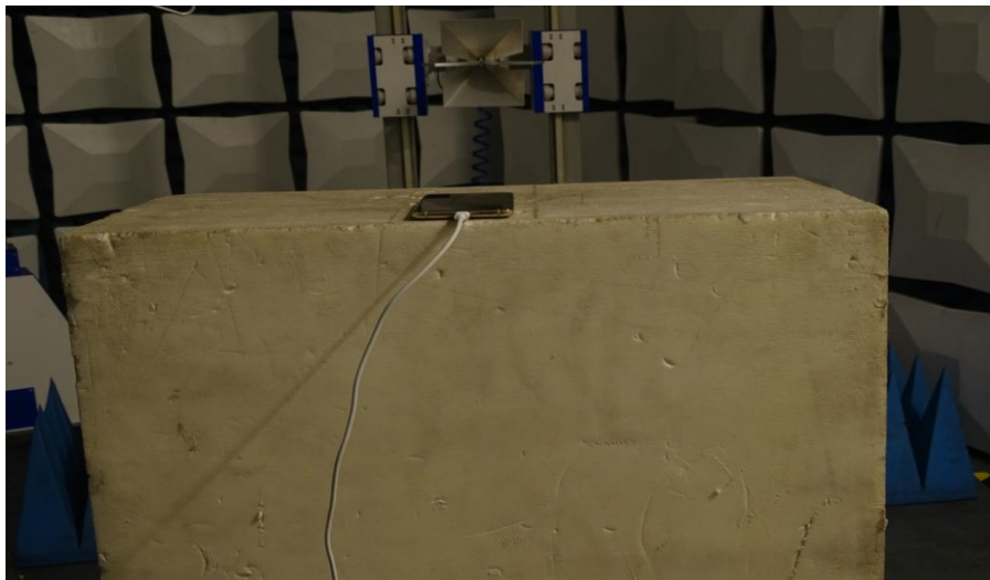
Radiated Spurious Emission (1GHz to18GHz)
