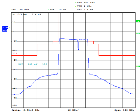
CA_7C 20MHz+10MHz 64QAM RB=100#0+50#0 CH- Middle
