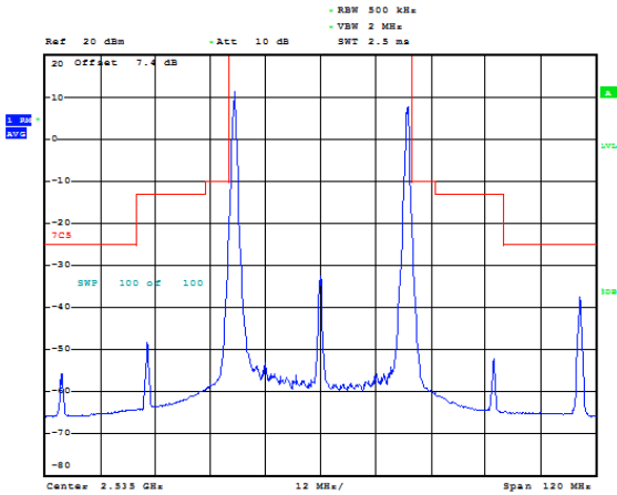
CA_7C 20MHz+20MHz QPSK RB=1#0+1#99 CH- Middle
