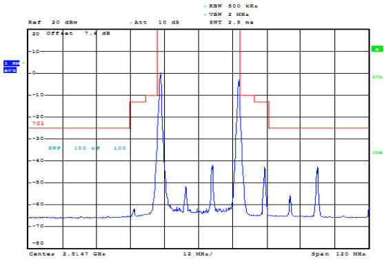
CA_7C 20MHz+10MHz 64QAM RB=1#0+1#49 CH- Low
