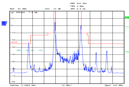
CA_41C 20MHz+5MHz QPSK RB=1#0+1#24 CH- High
