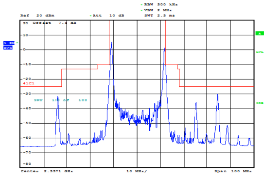
CA_41C 20MHz+5MHz QPSK RB=1#0+1#24 CH- Low
