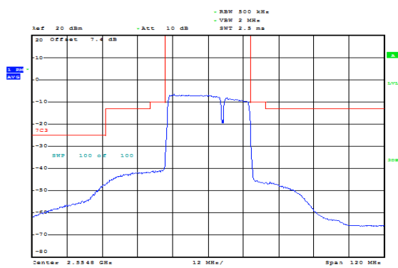
CA_7C 20MHz+10MHz 64QAM RB=100#0+50#0 CH- High
