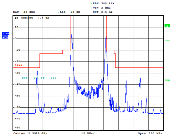
CA_41C 20MHz+5MHz QPSK RB=1#0+1#24 CH- Middle
