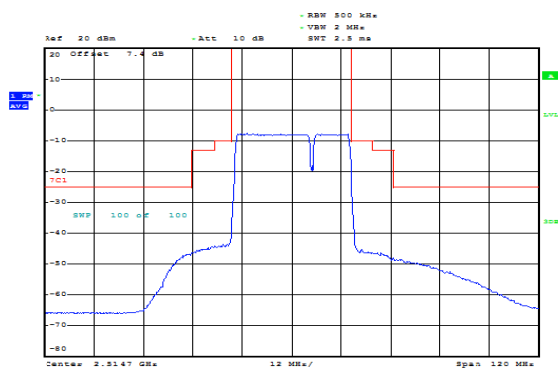
CA_7C 20MHz+10MHz 64QAM RB=100#0+50#0 CH- Low
