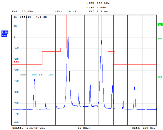
CA_7C 20MHz+10MHz 64QAM RB=1#0+1#49 CH- Middle
