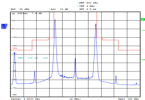
CA_7C 20MHz+20MHz QPSK RB=1#0+1#99 CH- High
