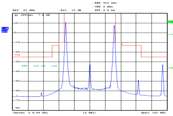
CA_7C 20MHz+20MHz QPSK RB=1#0+1#99 CH- Low
