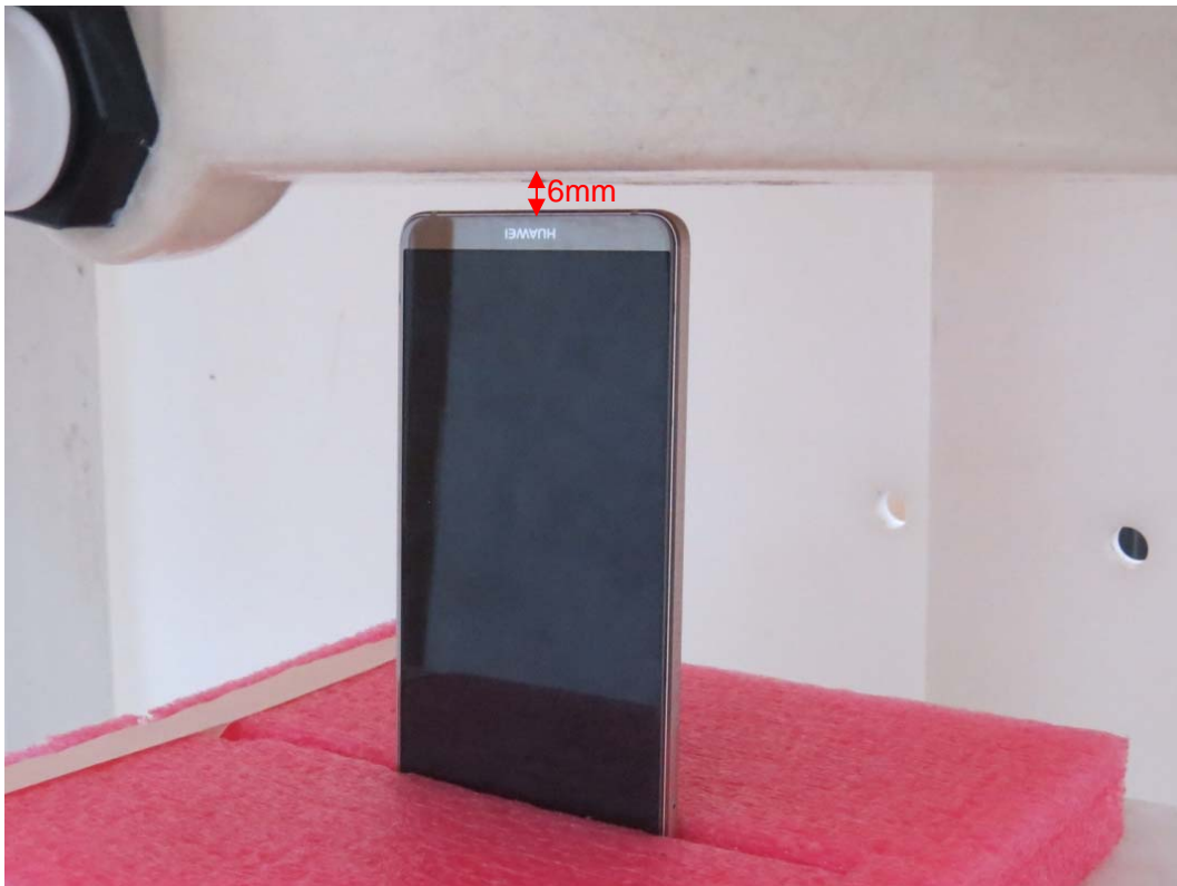
Picture 15: Bottom Side, the distance from handset to the bottom of the Phantom is 6mm
