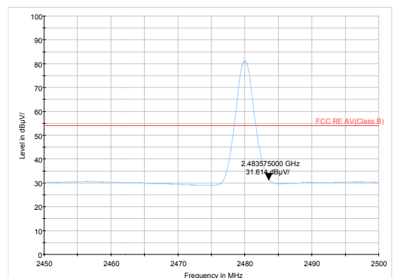
3DH5-Channel 78: Average
