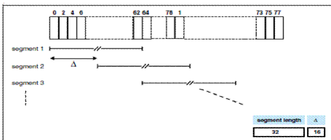
Hop selection scheme in CONNECTION state.
