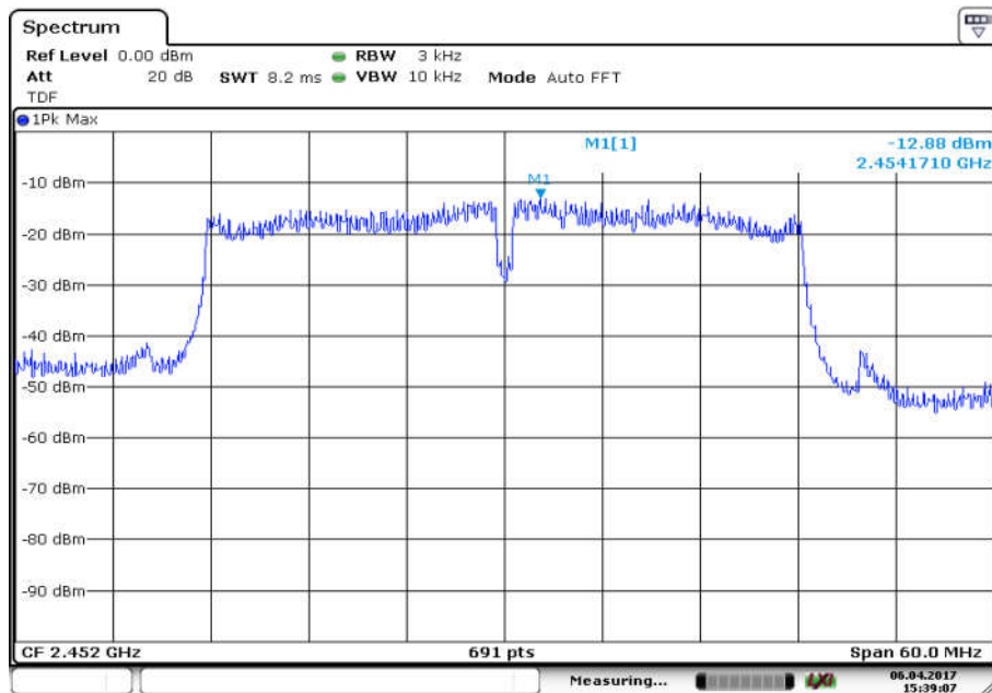
Fig.24 Power Spectral Density (802.11n-40MHz, Ch 9, MIMO Ant 2)
