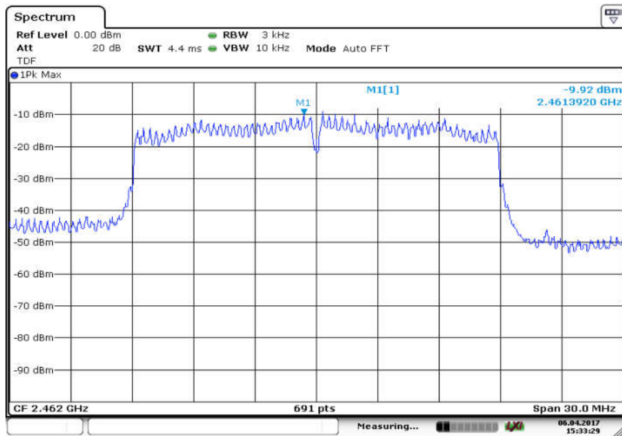
Fig.17 Power Spectral Density (802.11n-20MHz, Ch 11, MIMO Ant 1)
