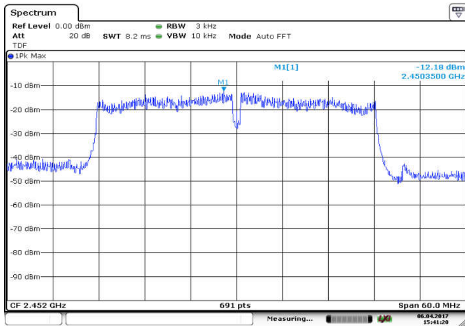
Fig.23 Power Spectral Density (802.11n-40MHz, Ch 9, MIMO Ant 1)
