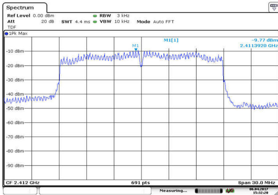
Fig.13 Power Spectral Density (802.11n-20MHz, Ch 1,MIMO Ant 1)
