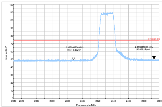
802.11g-Channel 5 Peak
